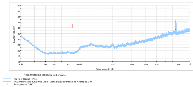
Figure 8.6-8: Radiated spurious emissions mid channel 30-1000 MHz
