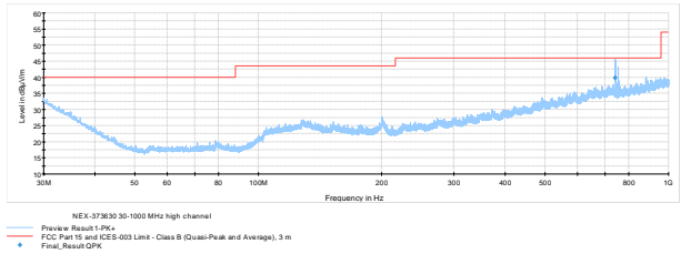
Figure 8.6-11: Radiated spurious emissions high channel 30-1000 MHz
