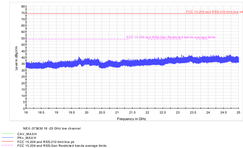
Figure 8.6-7: Radiated spurious emissions low channel 18-25 GHz
