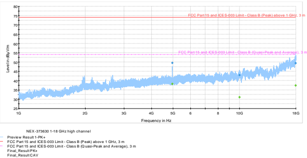
Figure 8.6-12: Radiated spurious emissions high channel 1-18 GHz
