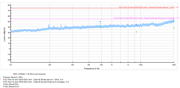
Figure 8.6-9: Radiated spurious emissions mid channel 1-18 GHz
