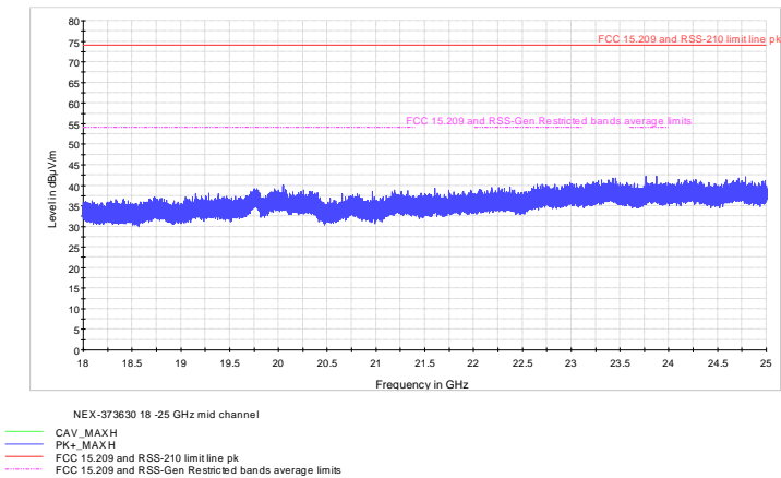
Figure 8.6-10: Radiated spurious emissions mid channel 18-25 GHz
