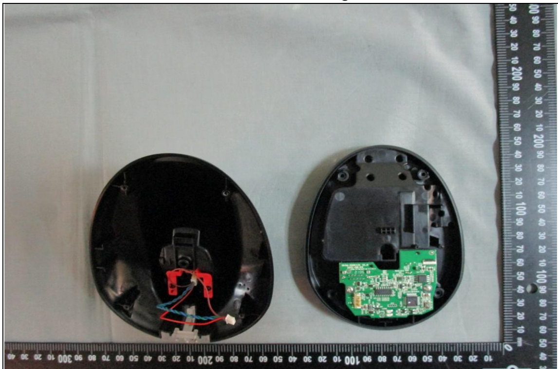
< Inside View of Charger >
