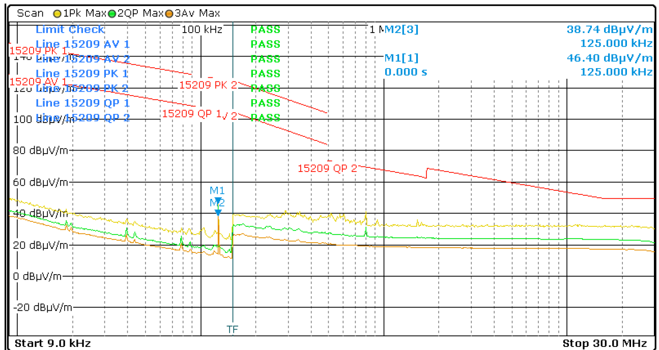
Figure 8: Chart of radiated emissions test below 30 MHz, EUT position Y, antenna polarization parallel, without tag
