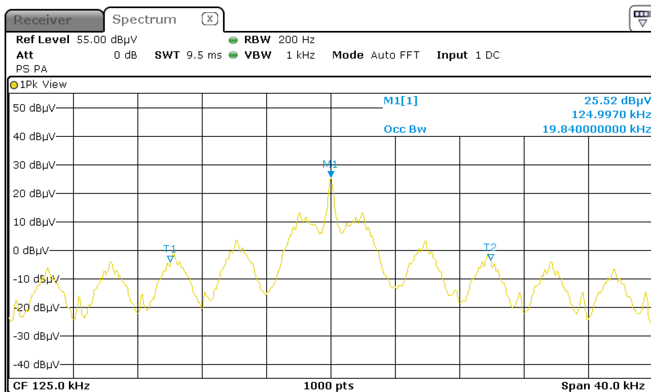
Figure 7: Chart of occupied bandwidth test, with tag
