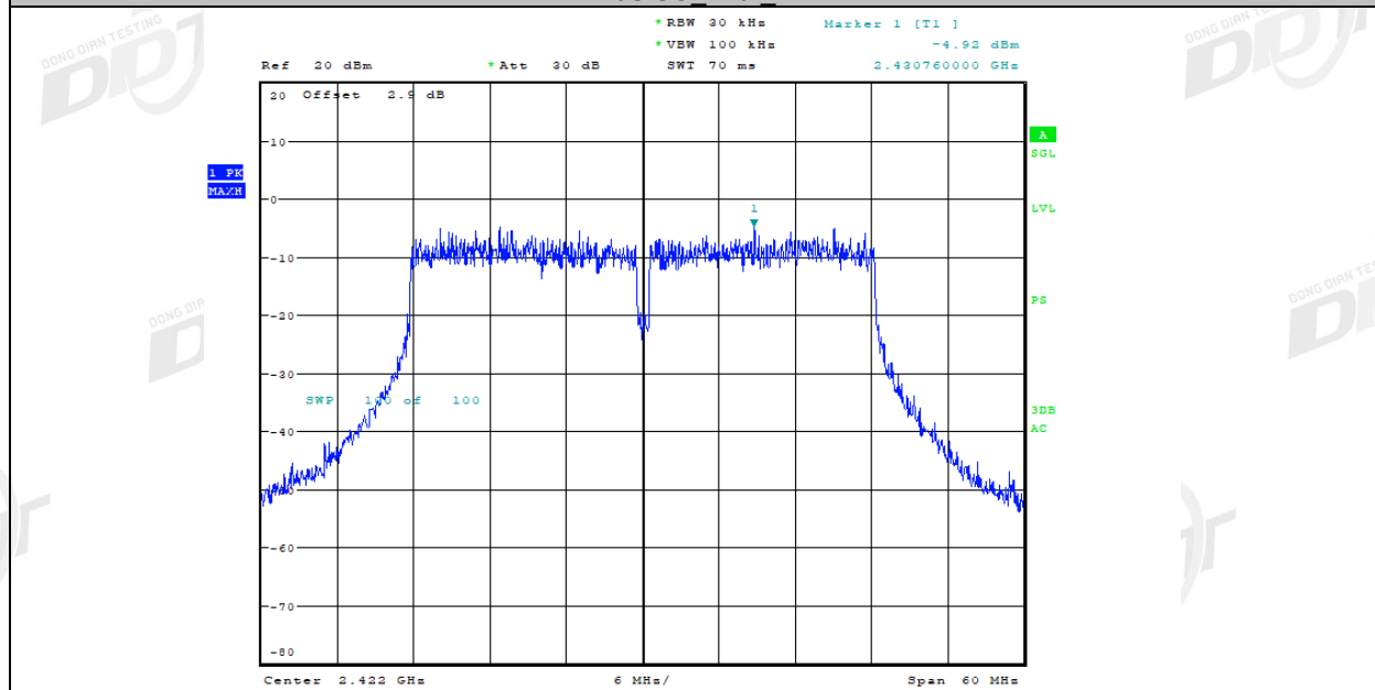
11N40SISO_Ant1_2422
