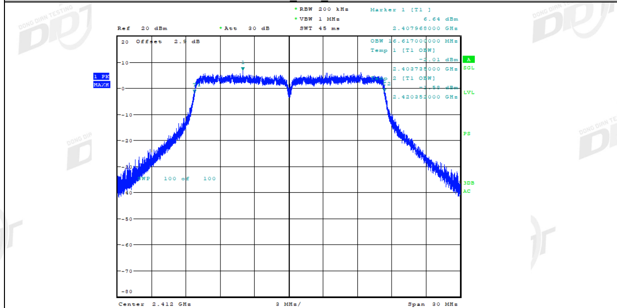
11G Ant1_2412
