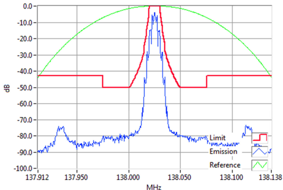
FFSK2400 138.0250MHz Mask C 1W RBW=300Hz, VBW=3000Hz, Detector Mode=Peak Result=Pass
