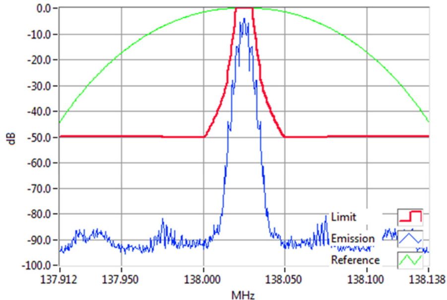
FFSK2400 138.0250MHz Mask C 5W RBW=300Hz, VBW=3000Hz, Detector Mode=Peak Result=Pass
