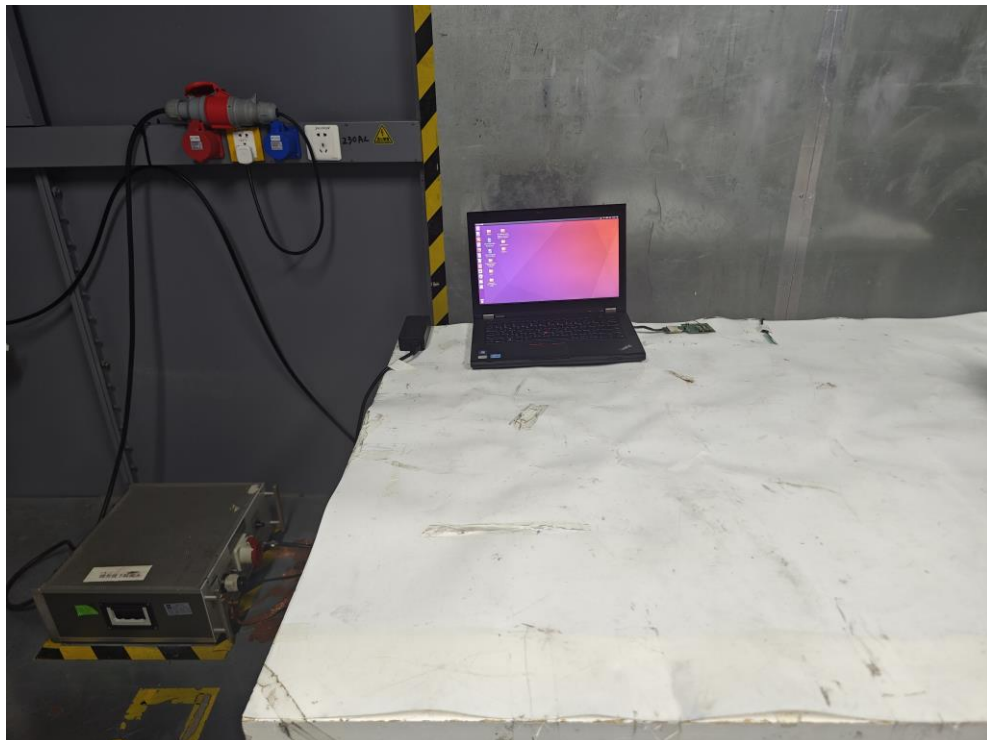
11.2.Photo of Conducted Emission test
