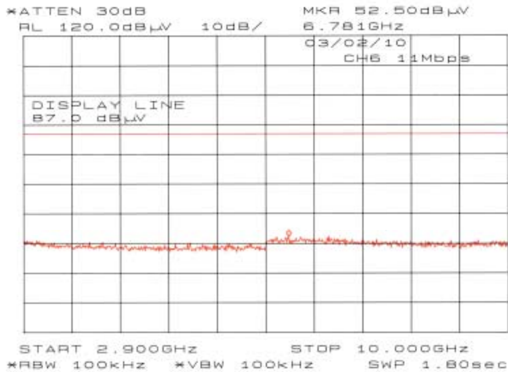
Chart of ch 6 with 11Mbps (2.9GHz-10GHz)
