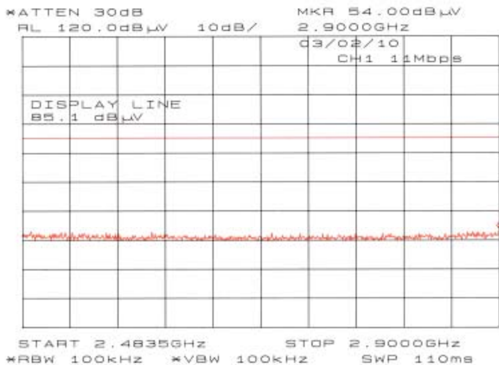
Chart of ch 1 with 11Mbps (2.4835GHz-2.9GHz)
