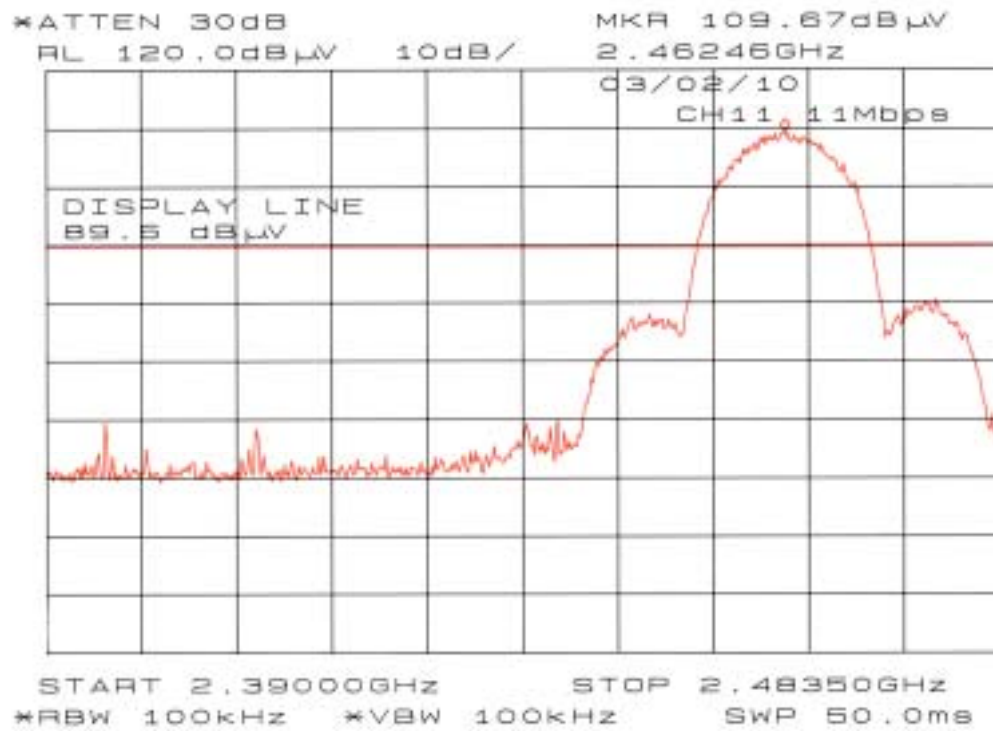
Chart of ch 11 with 11Mbps (2.390GHz-2.4835GHz)
