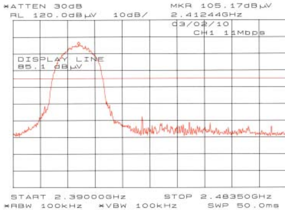
Chart of ch 1 with 11Mbps (2.390GHz-2.4835GHz)
