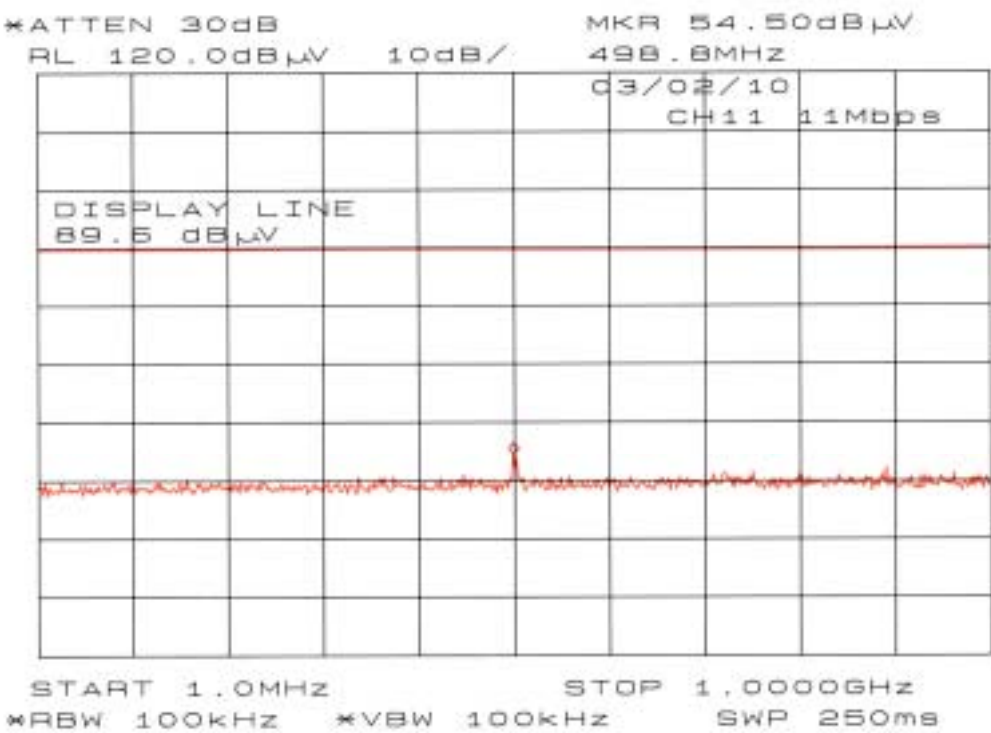
Chart of ch 11 with 11Mbps (1MHz-1GHz)
