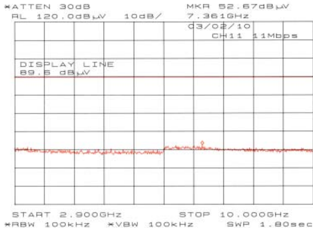
Chart of ch 11 with 11Mbps (2.9GHz-10GHz)
