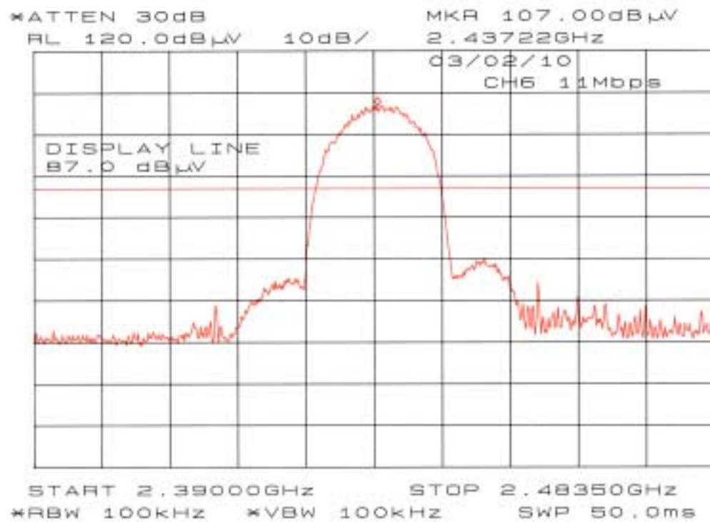
Chart of ch 6 with 11Mbps (2.390GHz-2.4835GHz)
