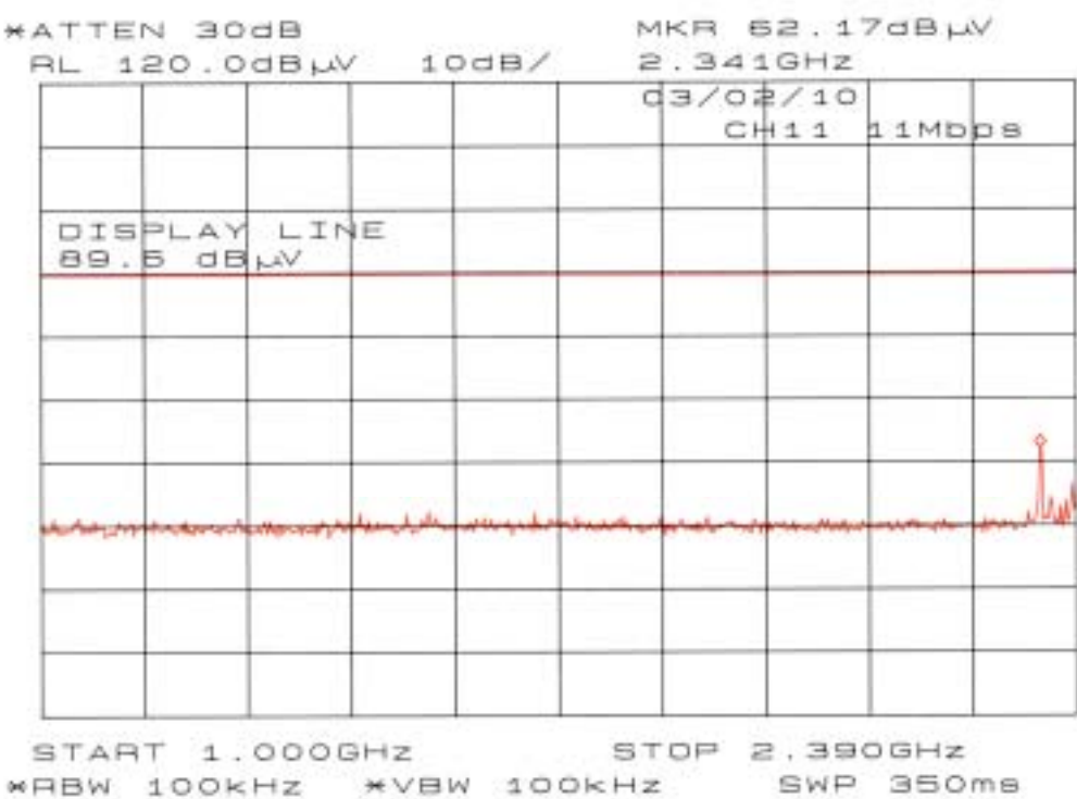
Chart of ch 11 with 11Mbps (1GHz-2.390GHz)
