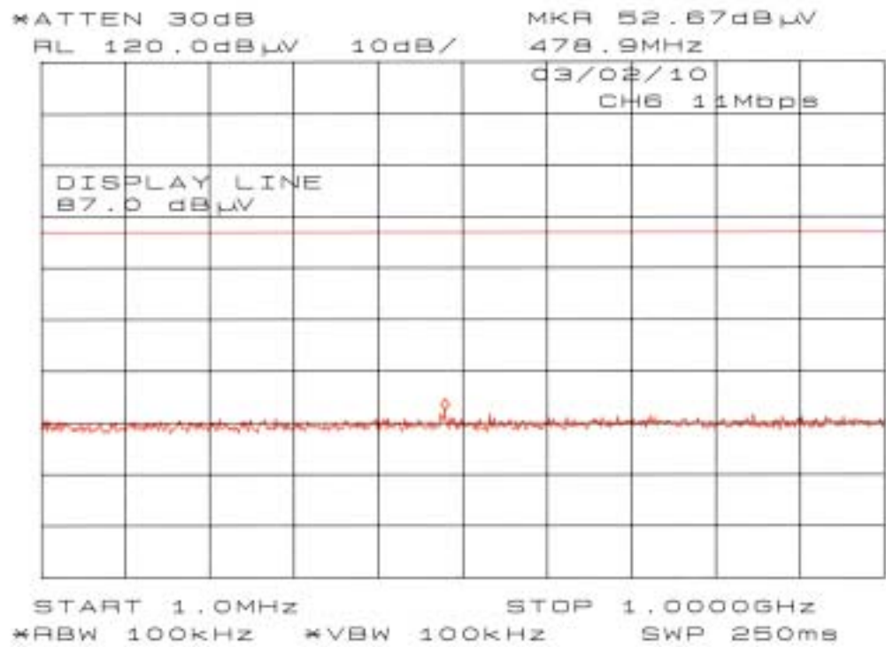
Chart of ch 6 with 11Mbps (1MHz-1GHz)
