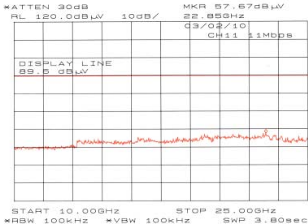
Chart of ch 11 with 11Mbps (10GHz-25GHz)
