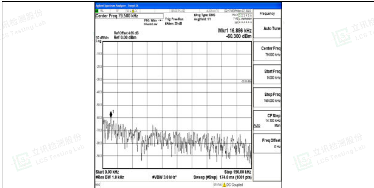
Band12_10MHz_64QAM_23130_1RB#0_0.009~0.15_0.009~0.15
