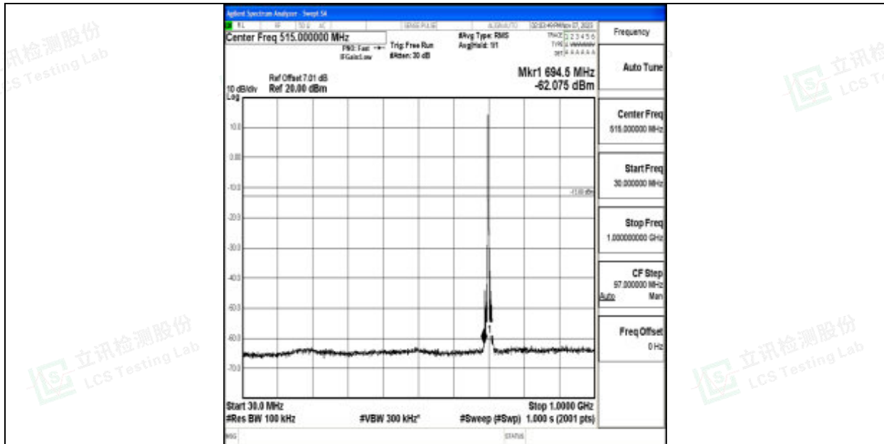
Band12_5MHz_64QAM_23095_1RB#0_30~1000_30~1000
