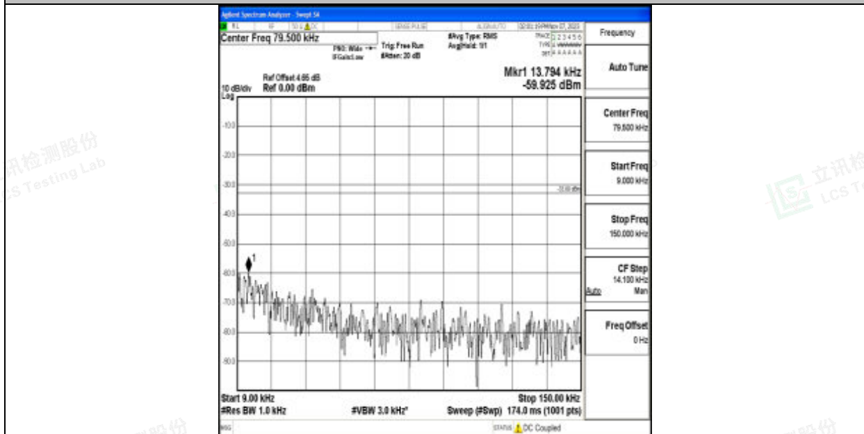
Band12_5MHz_64QAM_23035_1RB#0_0.009~0.15_0.009~0.15
