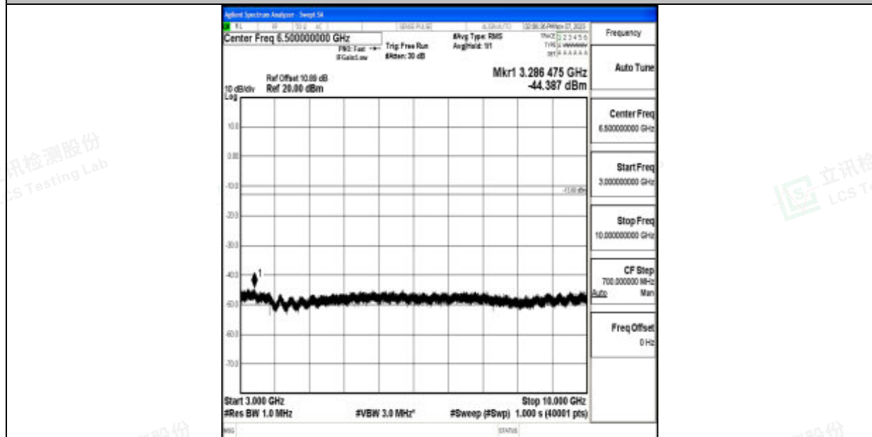
Band12_5MHz_64QAM_23155_1RB#0_3000~10000_3000~10000
