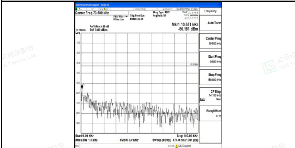
Band12_5MHz_64QAM_23155_1RB#0_0.009~0.15_0.009~0.15
