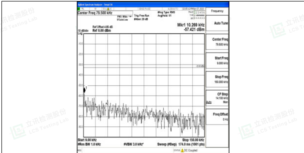
Band12_5MHz_16QAM_23155_1RB#0_0.009~0.15_0.009~0.15
