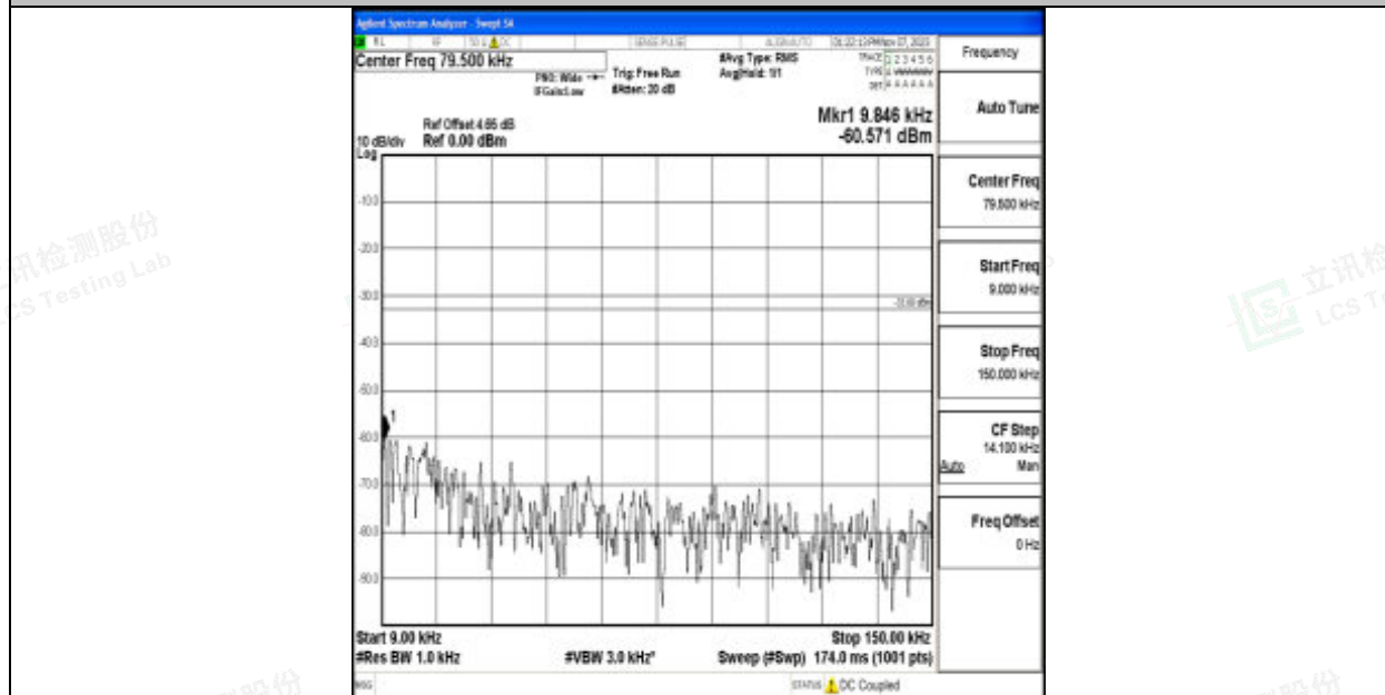
Band12_3MHz_64QAM_23095_1RB#0_0.009~0.15_0.009~0.15
