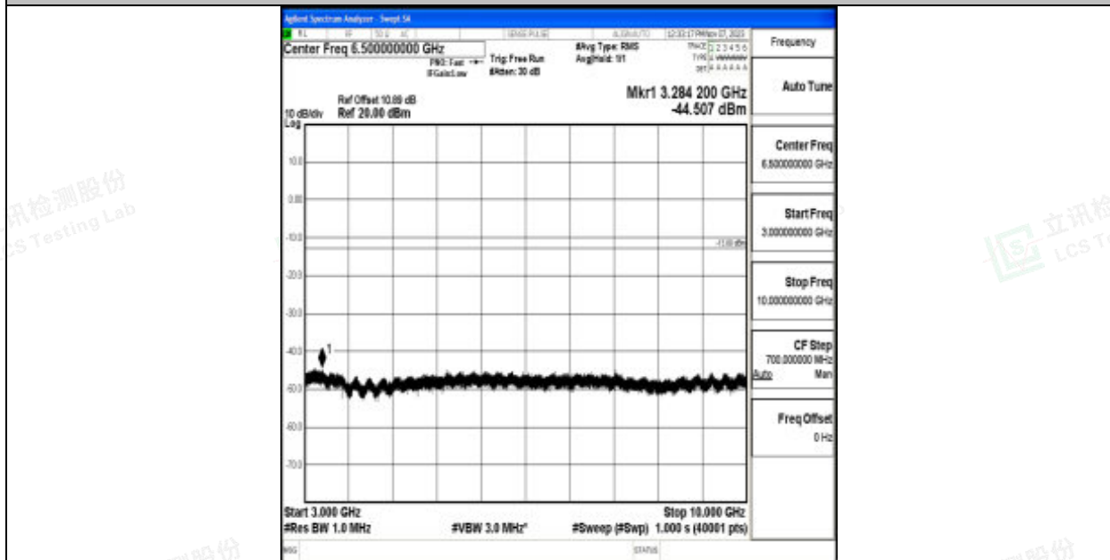
Band12_1.4MHz_QPSK_23173_1RB#0_3000~10000_3000~10000
