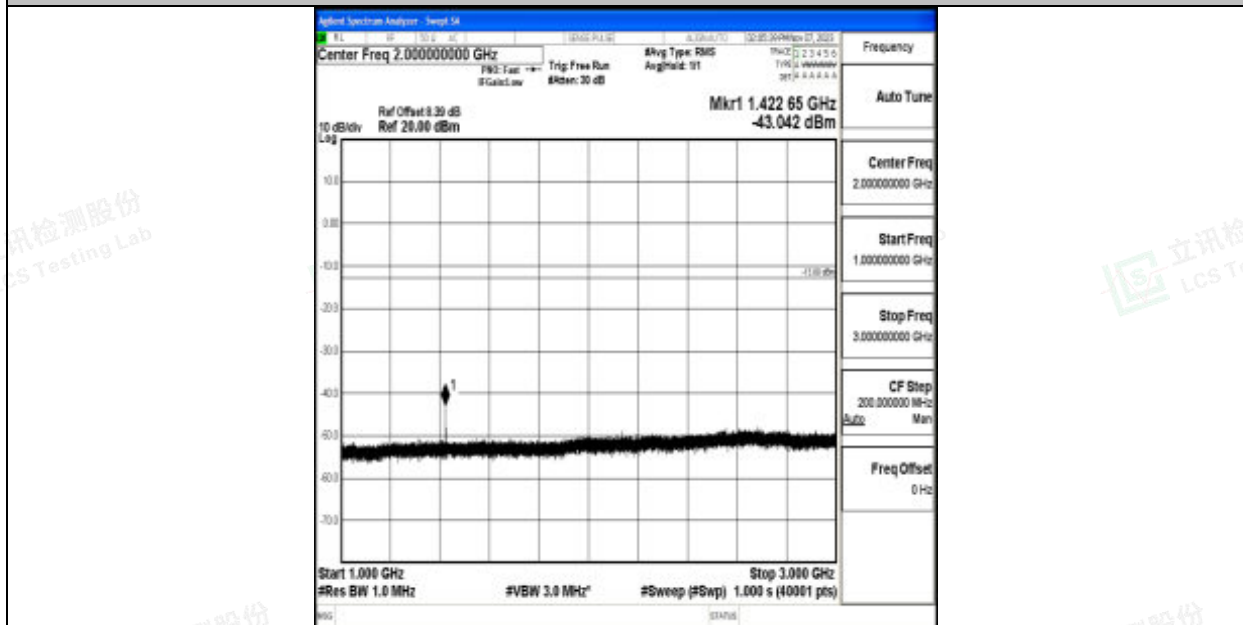
Band12_5MHz_16QAM_23155_1RB#0_1000~3000_1000~3000
