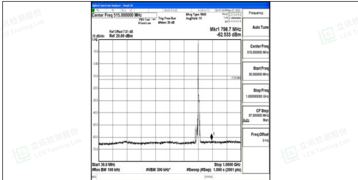
Band12_10MHz_64QAM_23130_1RB#0_30~1000_30~1000
