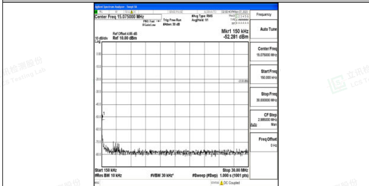
Band12_5MHz_16QAM_23035_1RB#0_0.15~30_0.15~30
