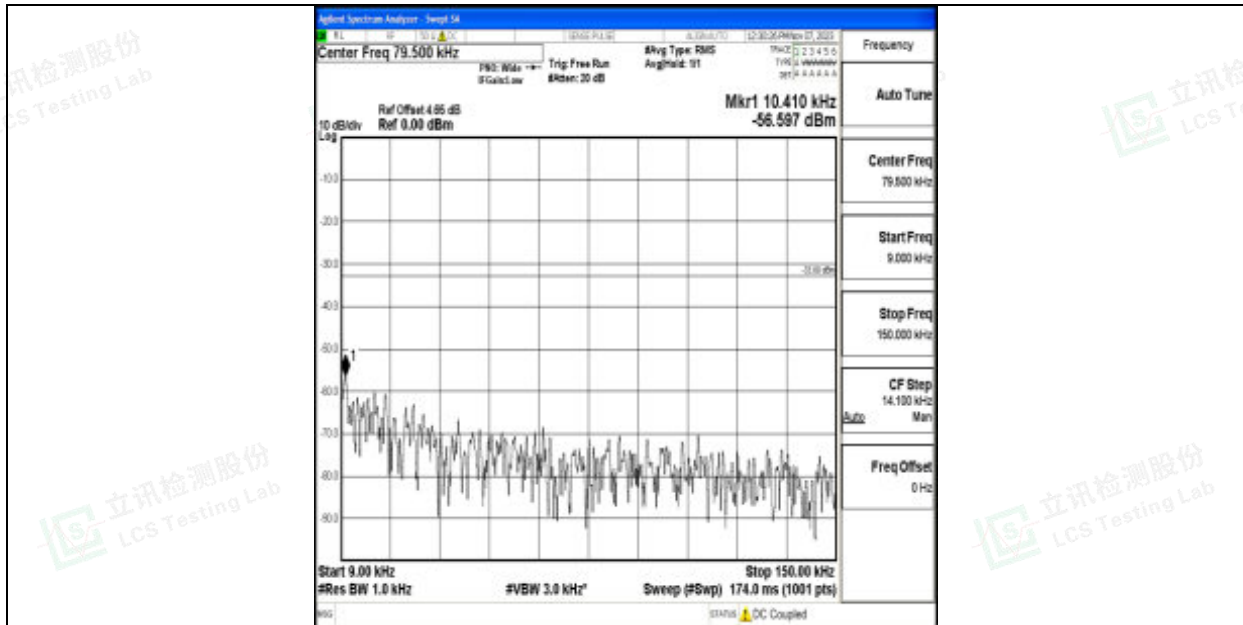
Band12_1.4MHz_QPSK_23095_1RB#0_0.009~0.15_0.009~0.15
