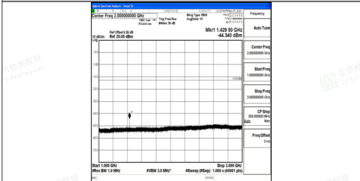
Band12_1.4MHz_16QAM_23173_1RB#0_1000~3000_1000~3000
