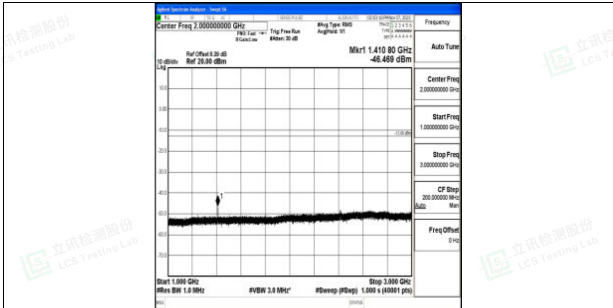
Band12_5MHz_16QAM_23095_1RB#0_1000~3000_1000~3000
