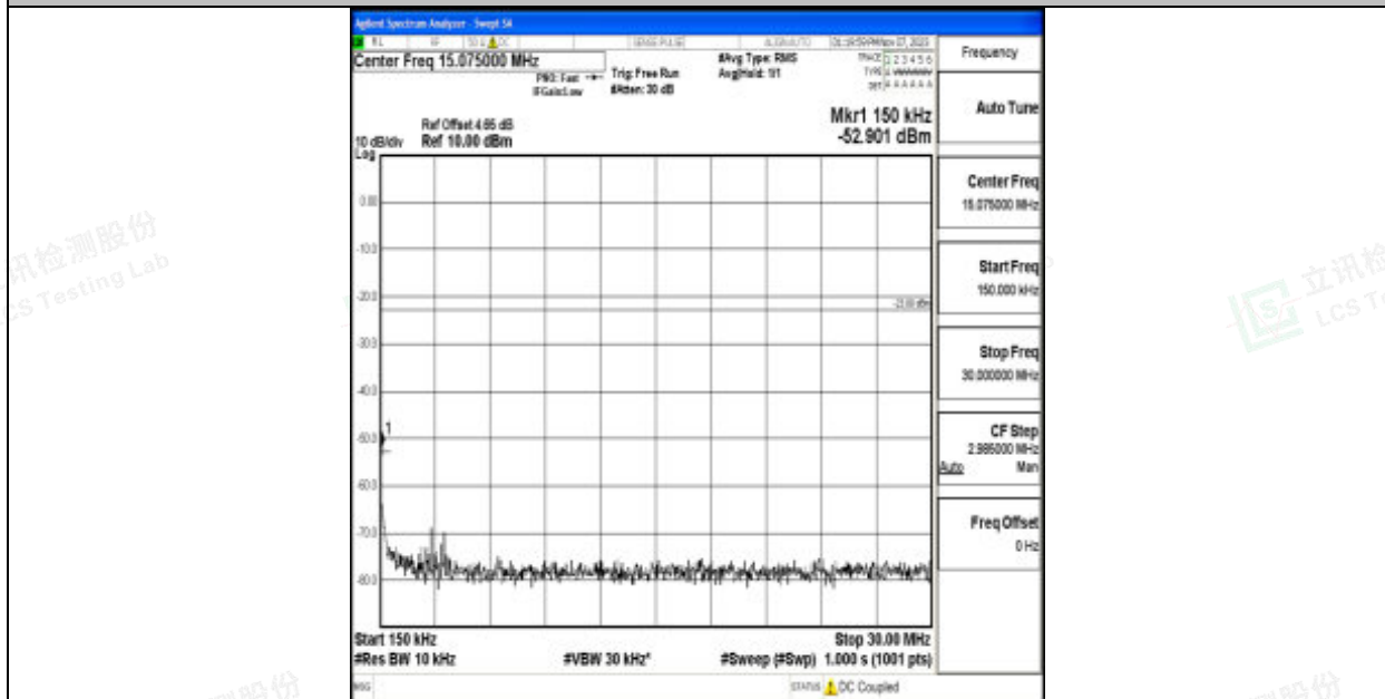
Band12_3MHz_64QAM_23025_1RB#0_0.15~30_0.15~30
