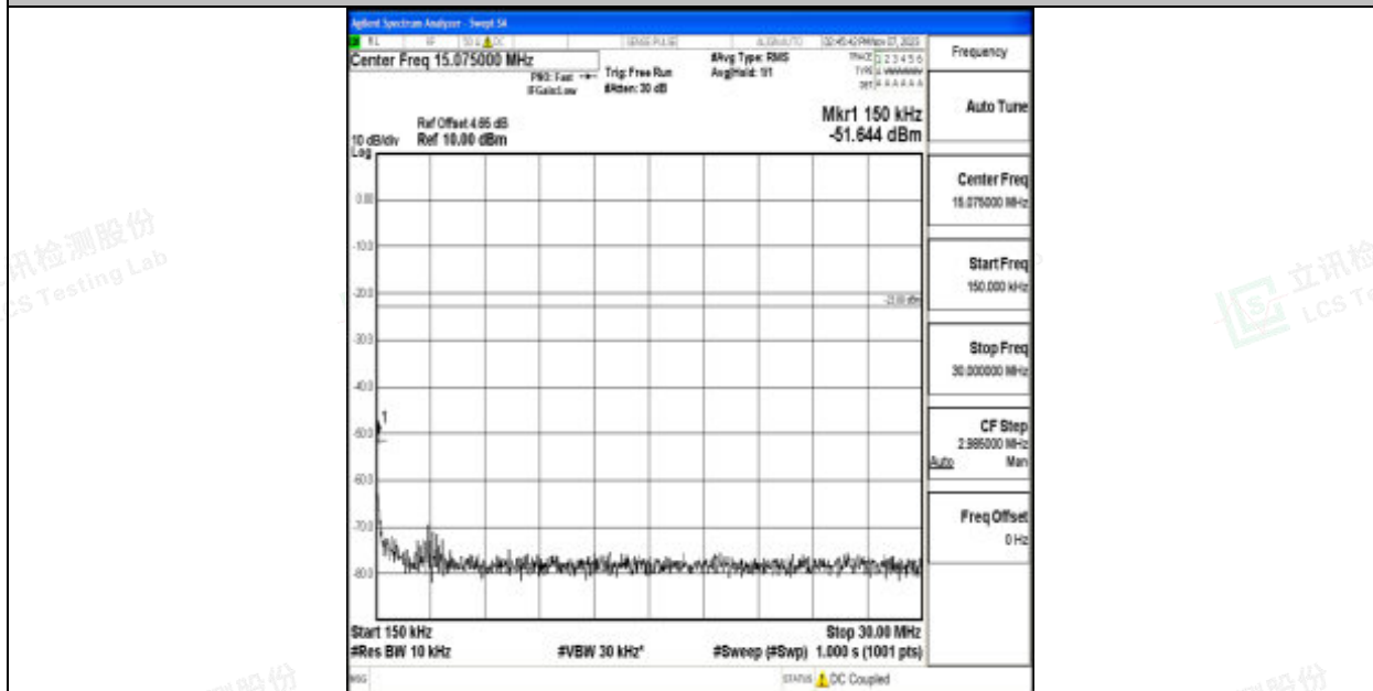
Band12_10MHz_QPSK_23130_1RB#0_0.15~30_0.15~30
