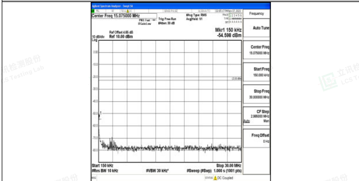
Band12_5MHz_16QAM_23155_1RB#0_0.15~30_0.15~30
