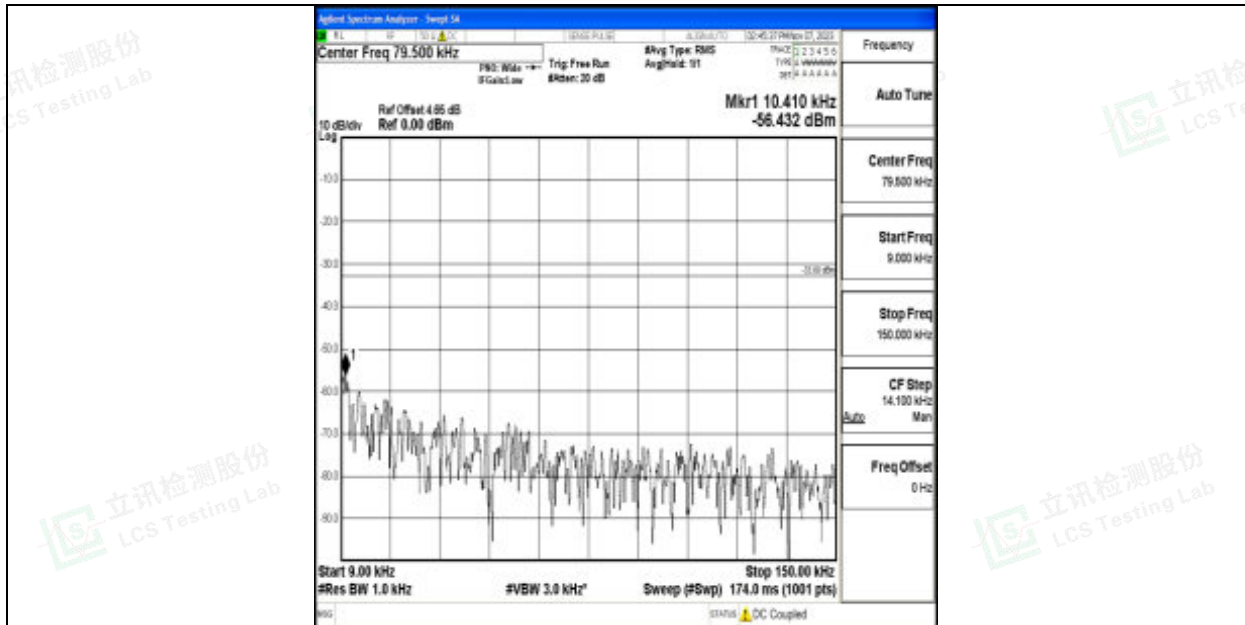
Band12_10MHz_QPSK_23130_1RB#0_0.009~0.15_0.009~0.15
