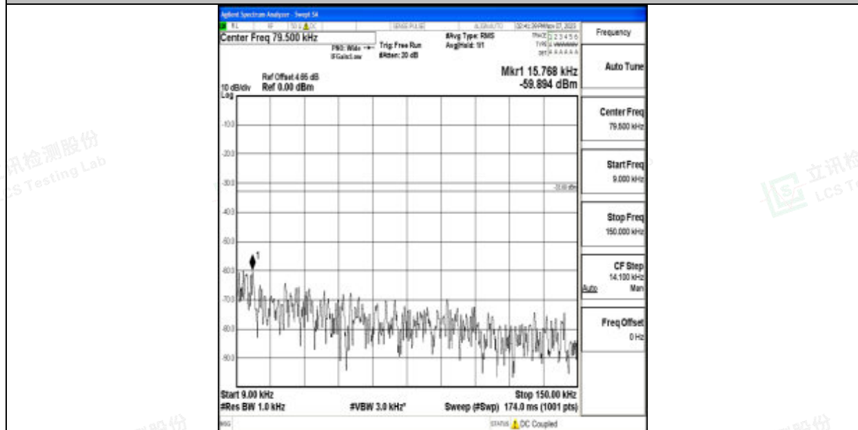
Band12_10MHz_16QAM_23060_1RB#0_0.009~0.15_0.009~0.15
