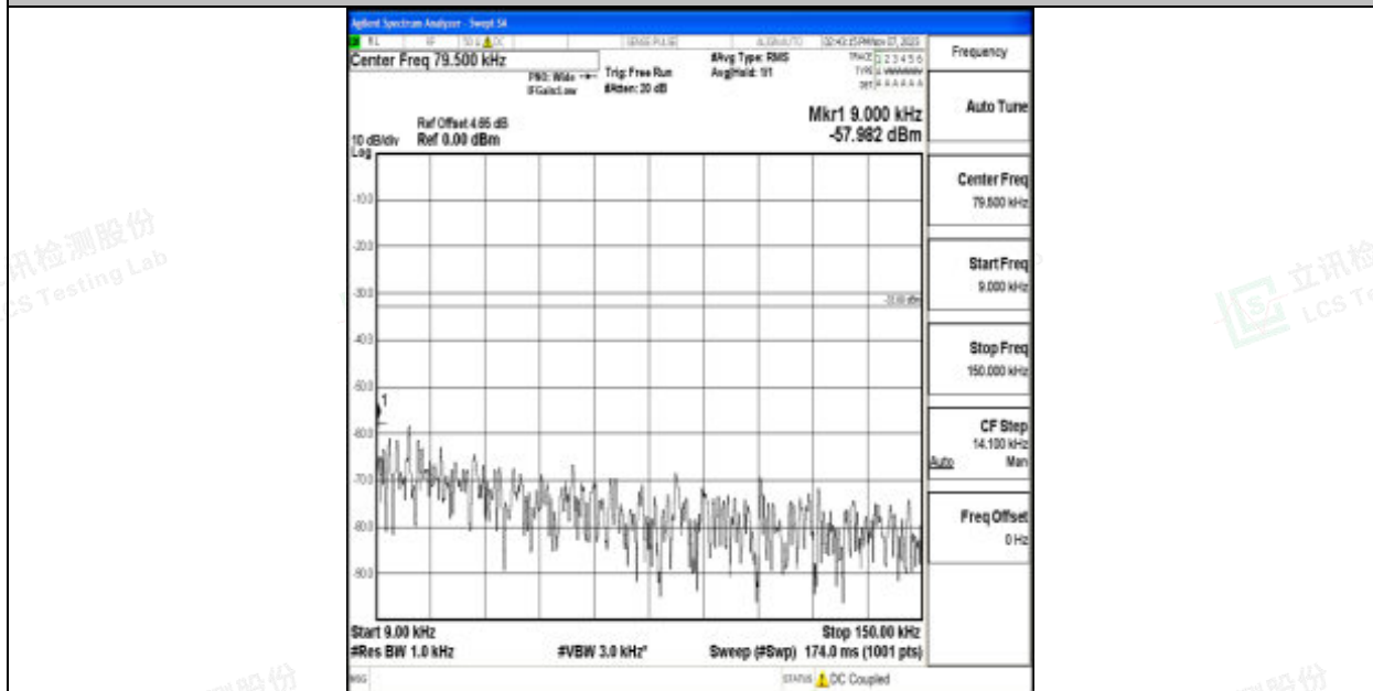
Band12_10MHz_QPSK_23095_1RB#0_0.009~0.15_0.009~0.15
