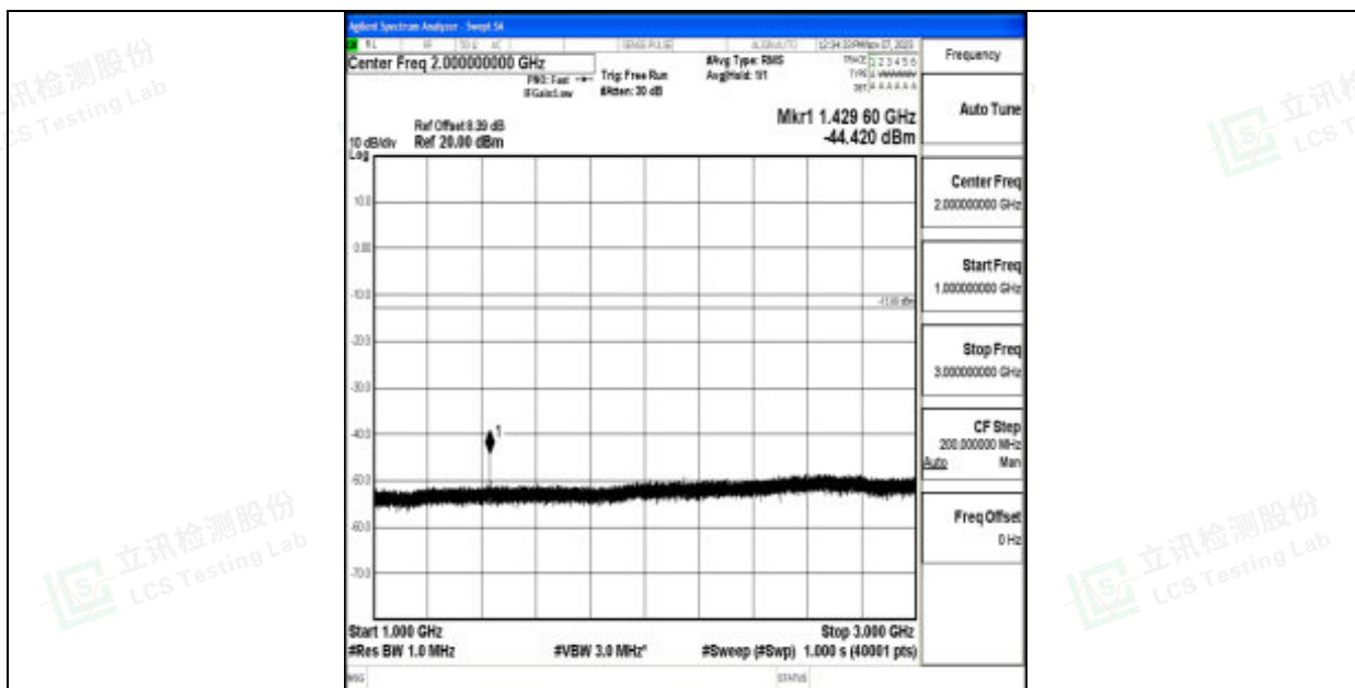
Band12 1.4MHz 64QAM 23173 1RB#0 1000~3000 1000~3000
