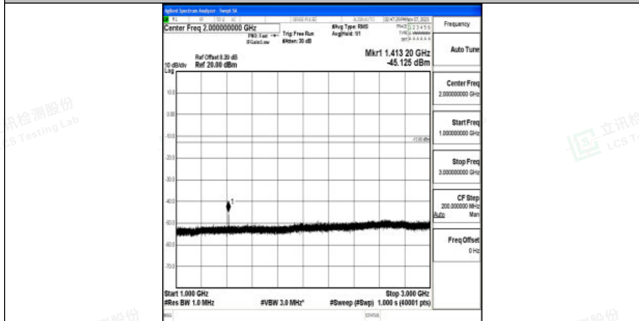
Band12_10MHz_64QAM_23130_1RB#0_1000~3000_1000~3000
