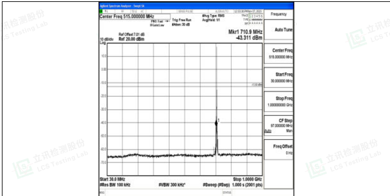
Band12_1.4MHz_16QAM_23173_1RB#0_30~1000_30~1000
