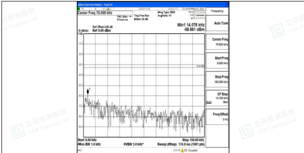
Band12_3MHz_64QAM_23025_1RB#0_0.009~0.15_0.009~0.15
