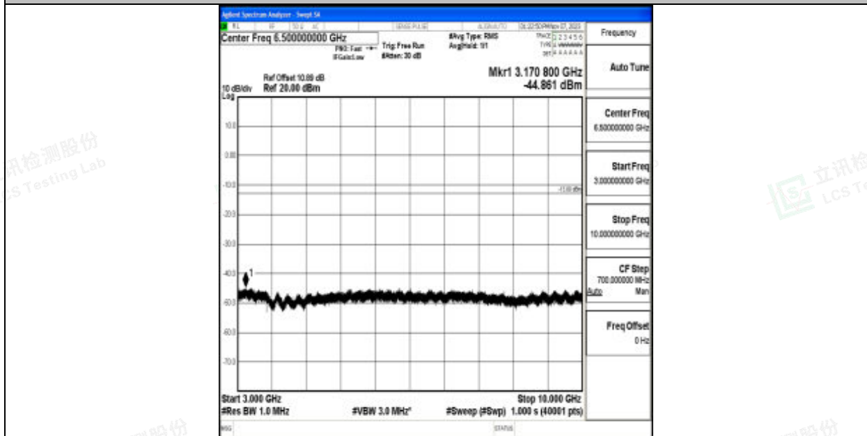
Band12_3MHz_64QAM_23095_1RB#0_3000~10000_3000~10000
