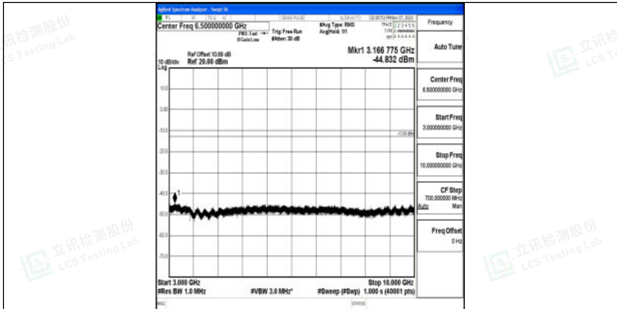
Band12_5MHz_16QAM_23155_1RB#0_3000~10000_3000~10000
