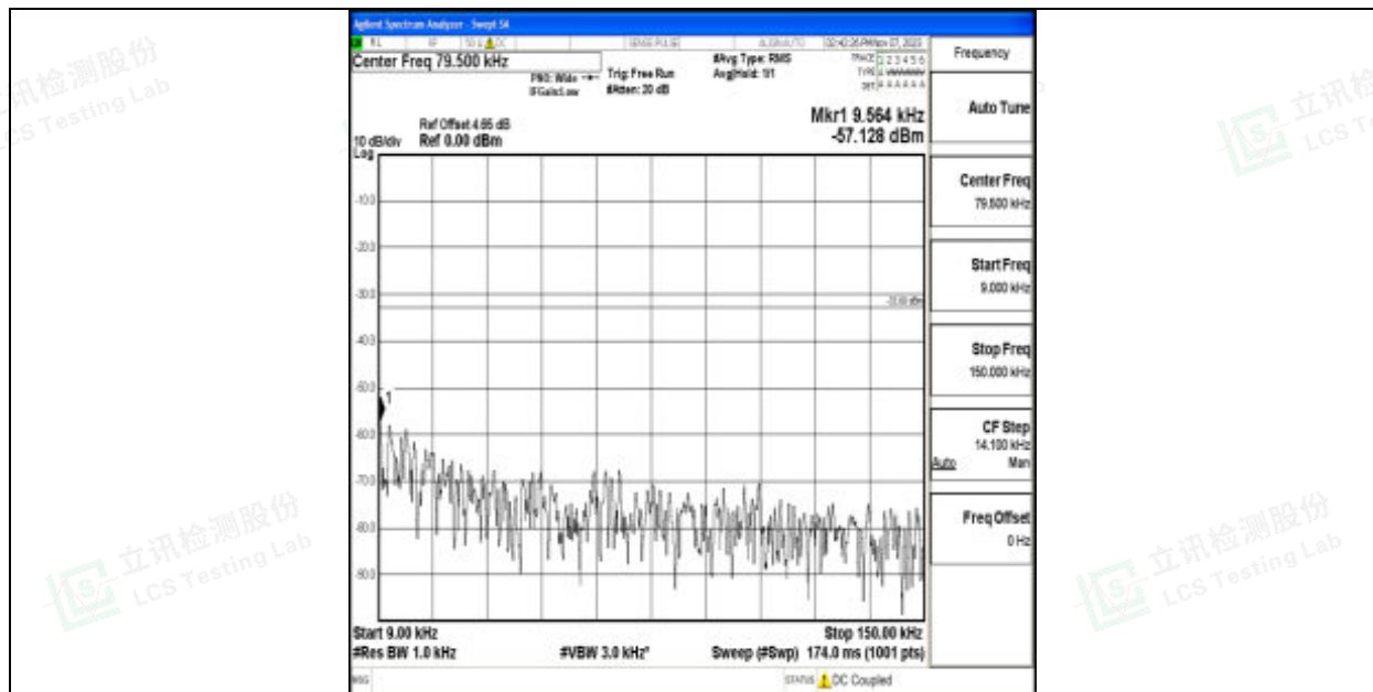
Band12_10MHz_64QAM_23060_1RB#0_0.009~0.15_0.009~0.15
