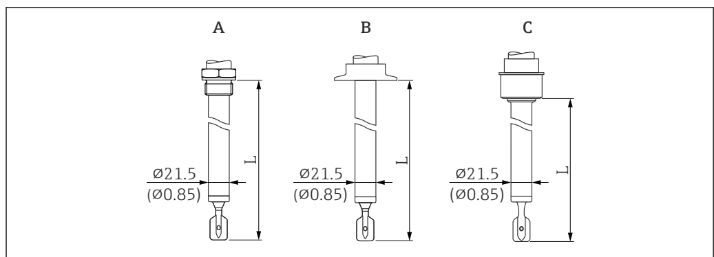
17 Probe designs: pipe extension, short pipe (sensor length L). Unit of measurement mm (in)
