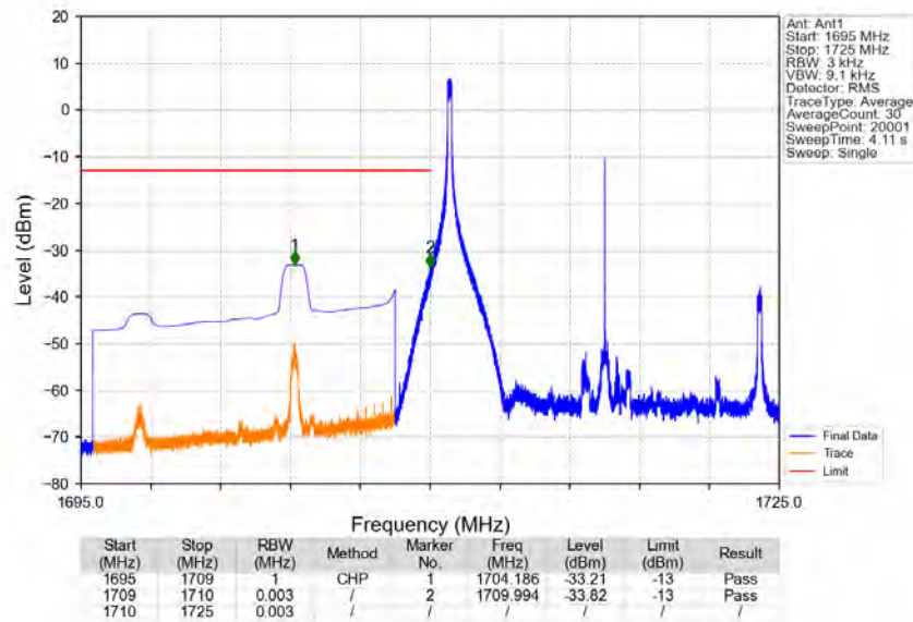
Band66_15MHz_64QAM_LCH_1717.5MHz_RB_1_0_NTNV
