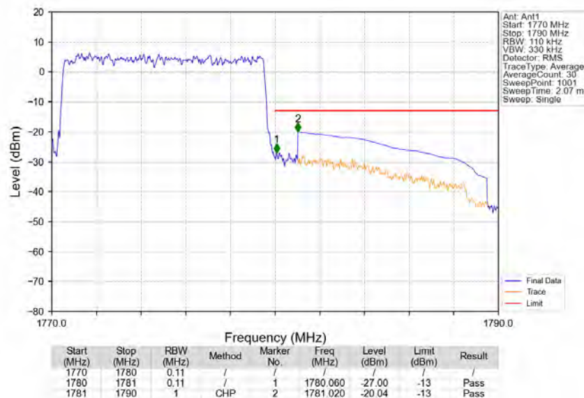
Band66_10MHz_QPSK_HCH_1775MHz_RB_50_0_NTNV
