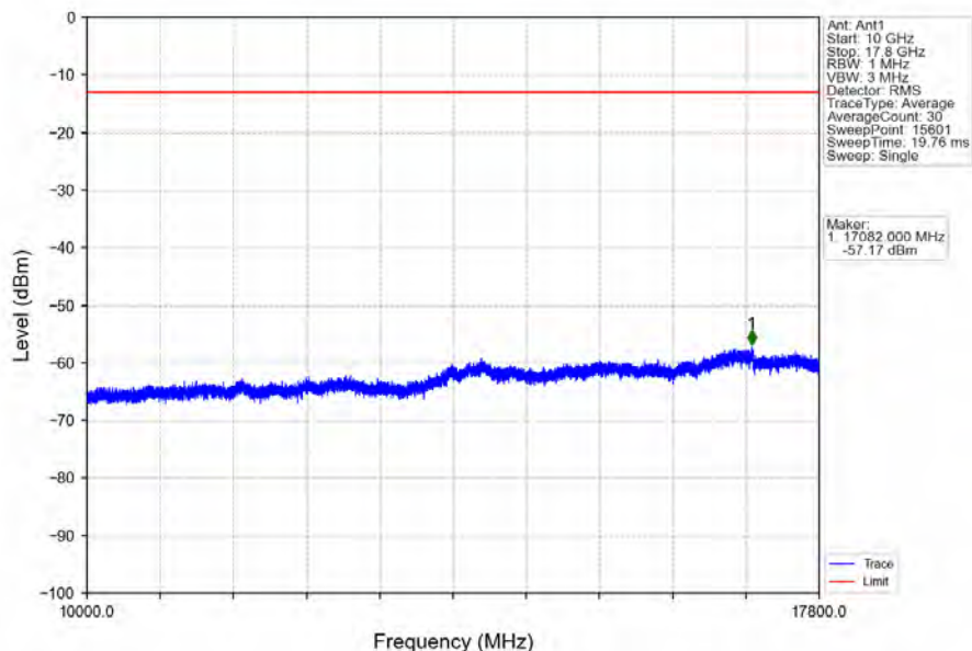
Band66_15MHz_16QAM_MCH_1745MHz_RB_1_0_NTNV
