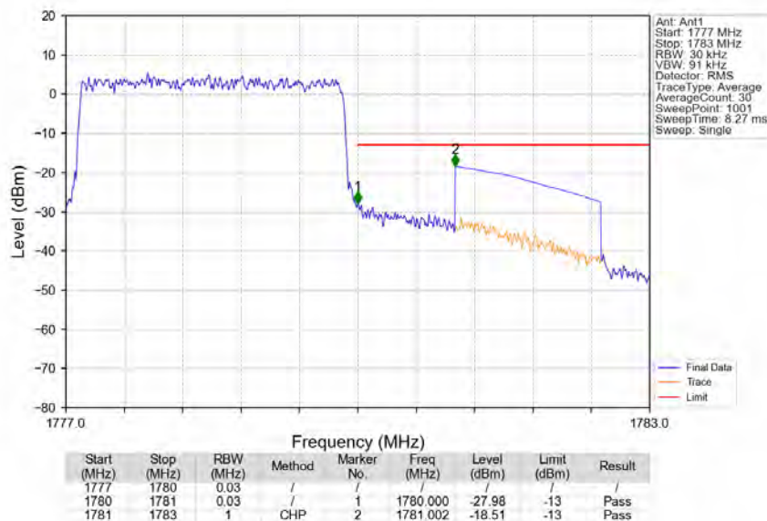
Band66_3MHz_16QAM_HCH_1778.5MHz_RB_15_0_NTNV
