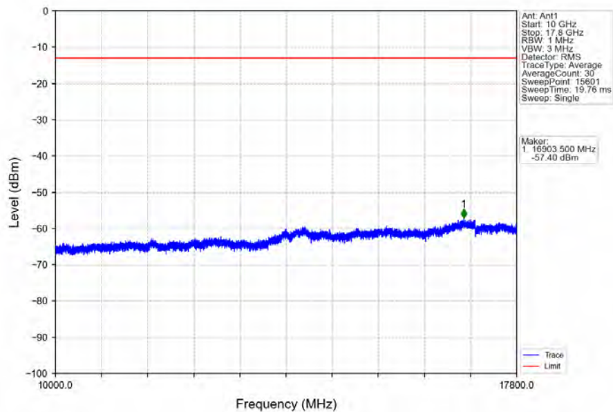
Band66_1.4MHz_64QAM_MCH_1745MHz_RB_1_0_NTNV
