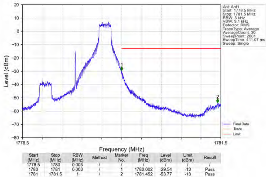
Band66_1.4MHz_64QAM_HCH_1779.3MHz_RB_1_5_NTNV
