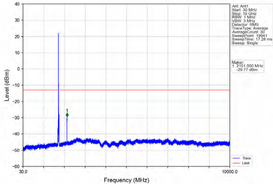
Band66_20MHz_16QAM_MCH_1745MHz_RB_1_0_NTNV
