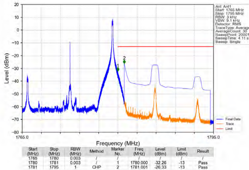
Band66_15MHz_16QAM_HCH_1772.5MHz_RB_1_74_NTNV
