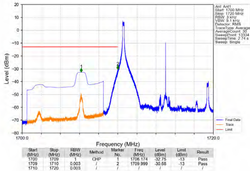
Band66_10MHz_64QAM_LCH_1715MHz_RB_1_0_NTNV
