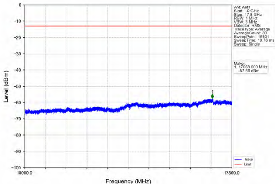
Band66_1.4MHz_64QAM_HCH_1779.3MHz_RB_1_0_NTNV
