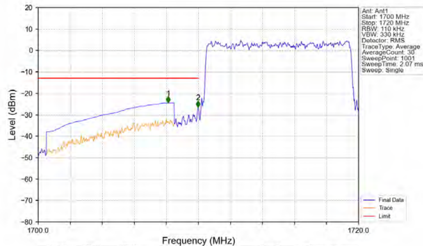
Band66_10MHz_64QAM_LCH_1715MHz_RB_50_0_NTNV
