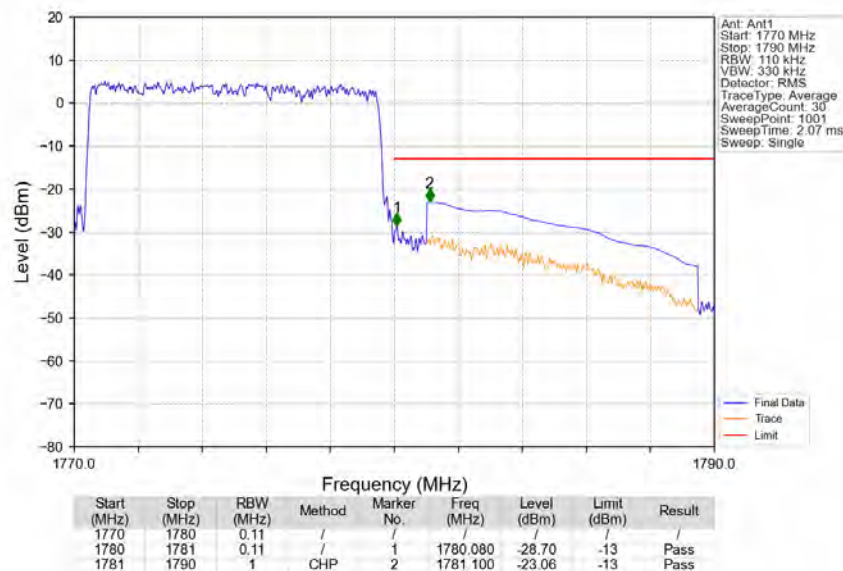
Band66_10MHz_16QAM_HCH_1775MHz_RB_50_0_NTNV
