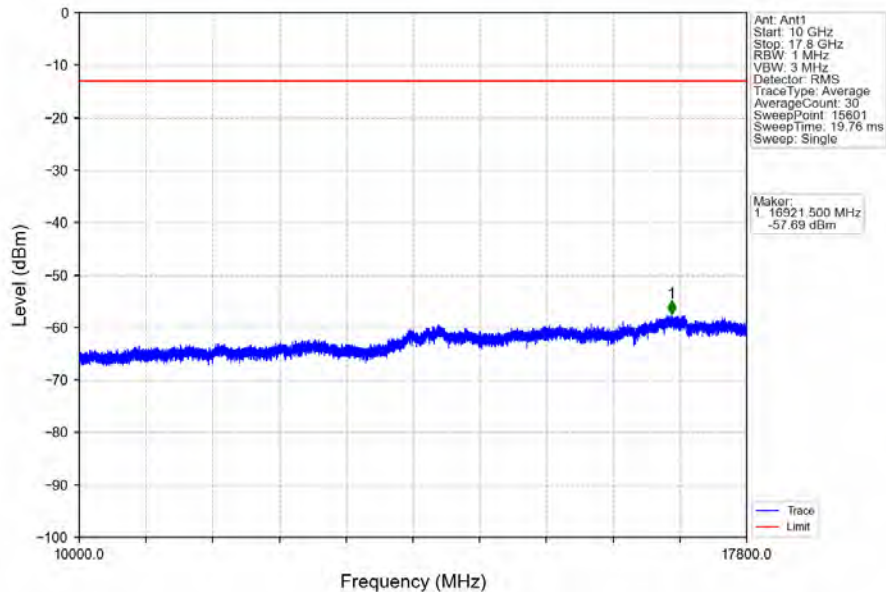
Band66_15MHz_64QAM_LCH_1717.5MHz_RB_75_0_NTNV
