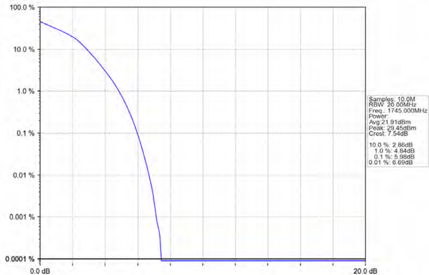
Band66_20MHz_16QAM_MCH_1745MHz_RB_100_0_NTNV
