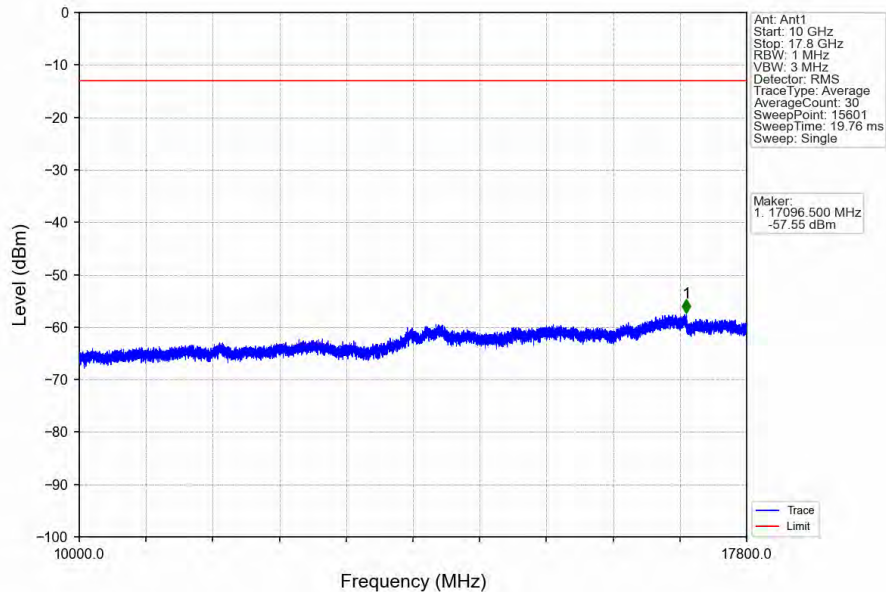
Band66_1.4MHz_QPSK_LCH_1710.7MHz_RB_6_0_NTNV
