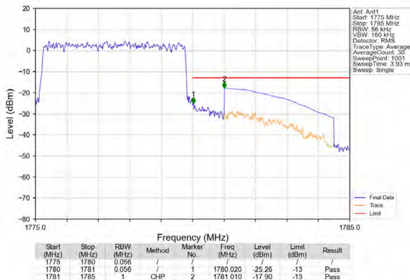
Band66_5MHz_64QAM_HCH_1777.5MHz_RB_25_0_NTNV
