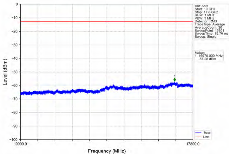
Band66_20MHz_16QAM_MCH_1745MHz_RB_1_0_NTNV
