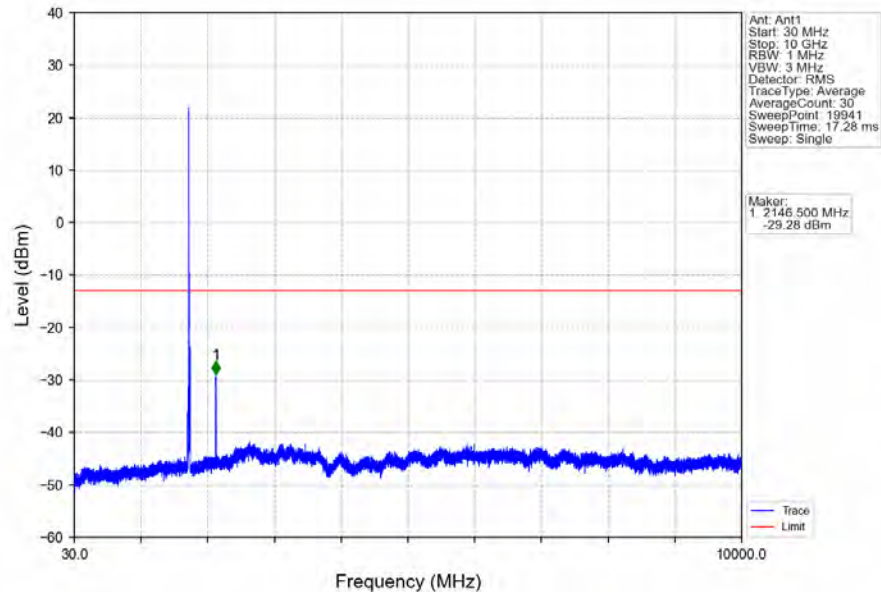
Band66_10MHz_16QAM_MCH_1745MHz_RB_1_0_NTNV
