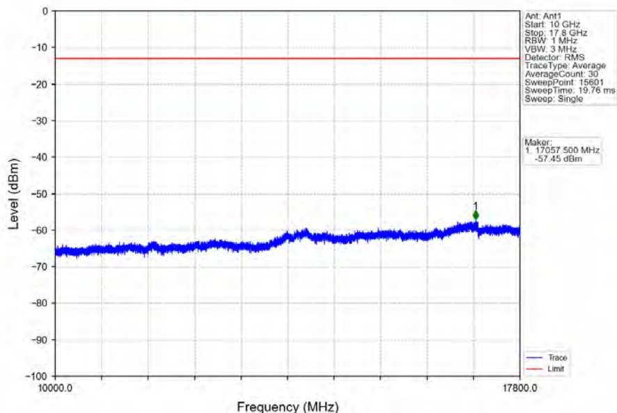
Band66_15MHz_64QAM_HCH_1772.5MHz_RB_1_0_NTNV
