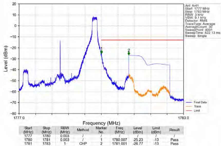
Band66_3MHz_QPSK_HCH_1778.5MHz_RB_1_14_NTNV
