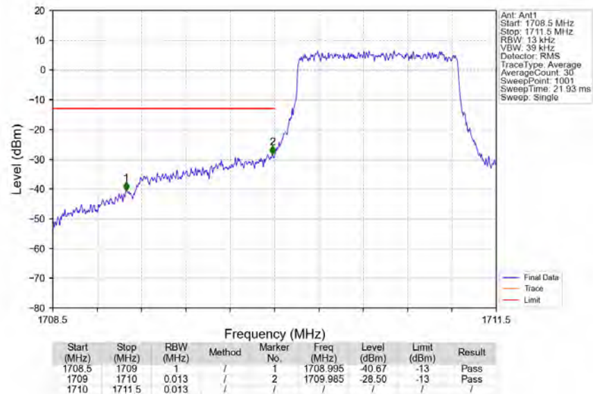
Band66_1.4MHz_QPSK_LCH_1710.7MHz_RB_6_0_NTNV
