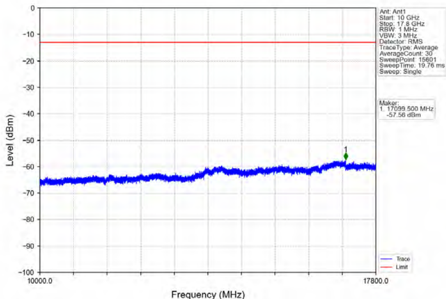
Band66_3MHz_16QAM_MCH_1745MHz_RB_1_0_NTNV
