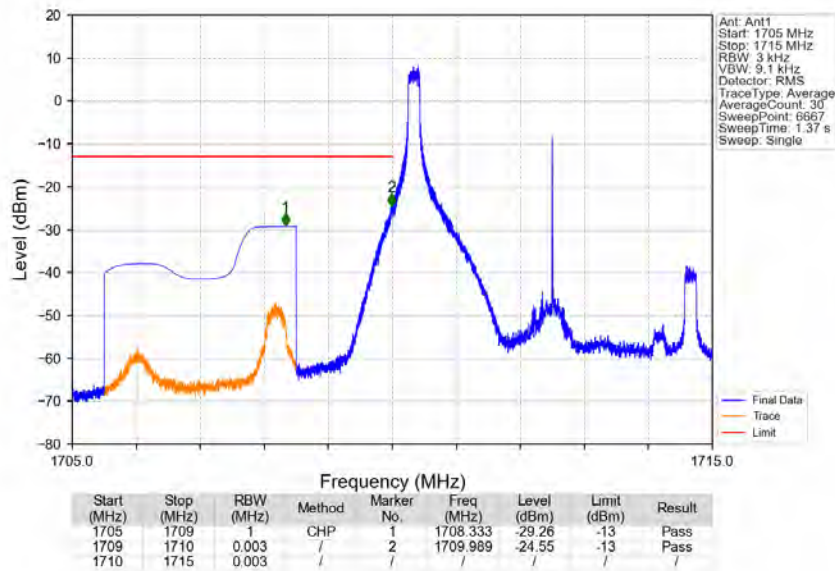
Band66_5MHz_16QAM_LCH_1712.5MHz_RB_1_0_NTNV
