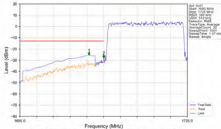
Band66_15MHz_64QAM_LCH_1717.5MHz_RB_75_0_NTNV
