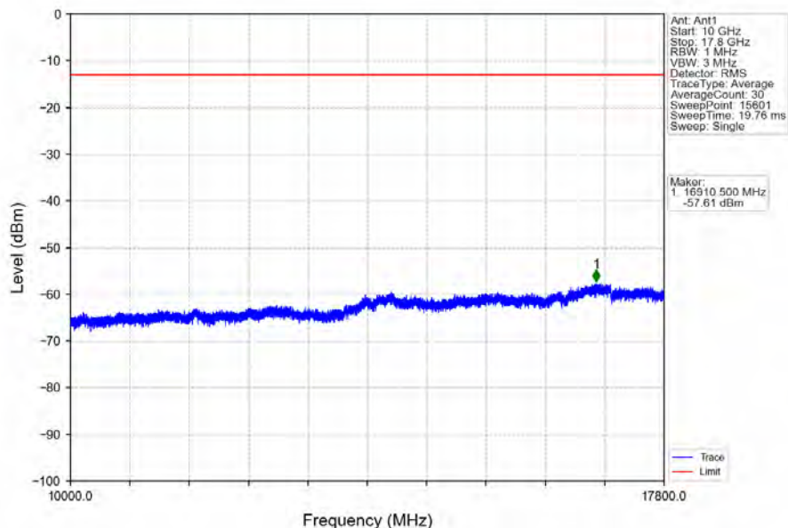
Band66_3MHz_64QAM_HCH_1778.5MHz_RB_1_0_NTNV
