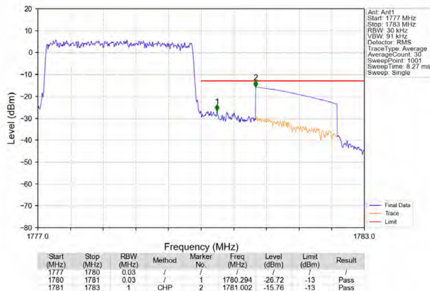
Band66_3MHz_QPSK_HCH_1778.5MHz_RB_15_0_NTNV
