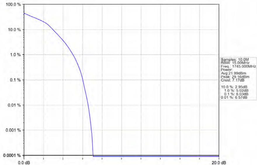
Band66_15MHz_16QAM_MCH_1745MHz_RB_75_0_NTNV
