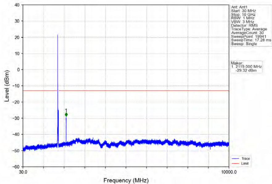
Band66_20MHz_64QAM_LCH_1720MHz_RB_1_0_NTNV
