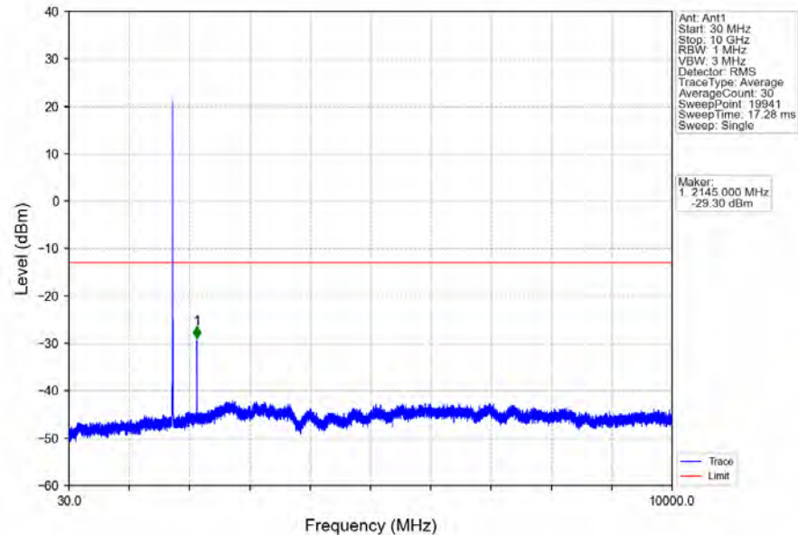
Band66_5MHz_64QAM_MCH_1745MHz_RB_1_0_NTNV
