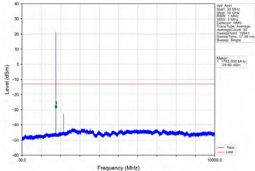
Band66_1.4MHz_64QAM_HCH_1779.3MHz_RB_1_0_NTNV
