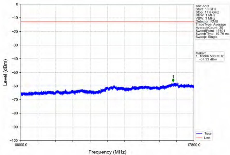
Band66_10MHz_16QAM_HCH_1775MHz_RB_1_0_NTNV
