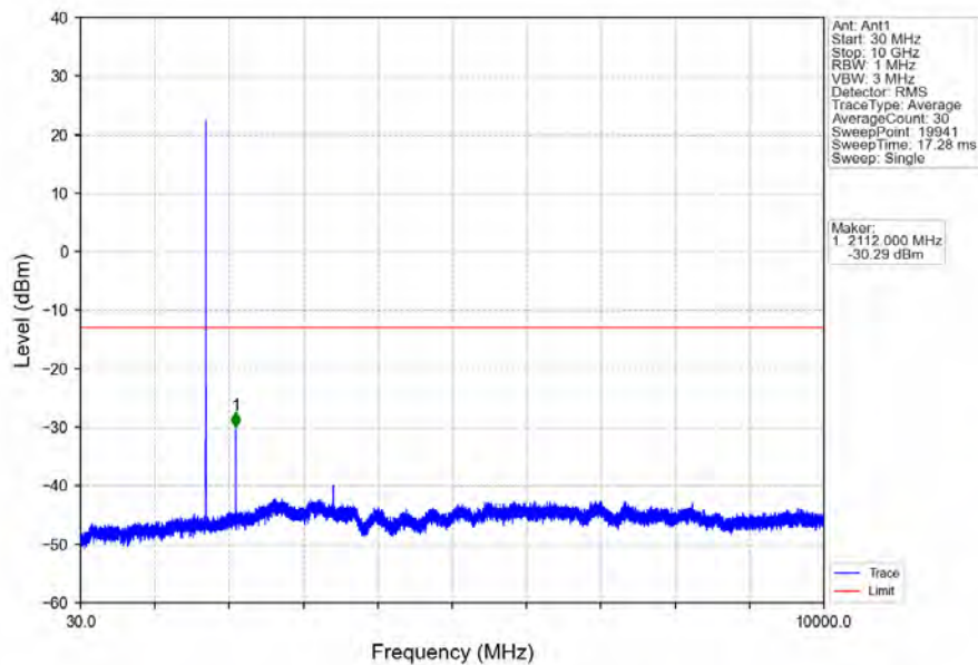
Band66_3MHz_16QAM_LCH_1711.5MHz_RB_1_0_NTNV
