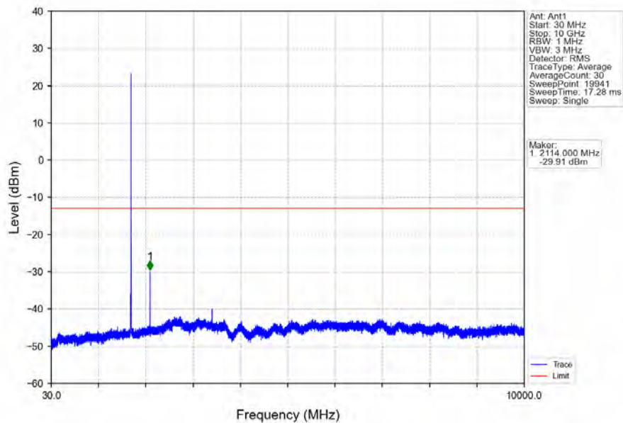
Band66_5MHz_16QAM_LCH_1712.5MHz_RB_1_0_NTNV
