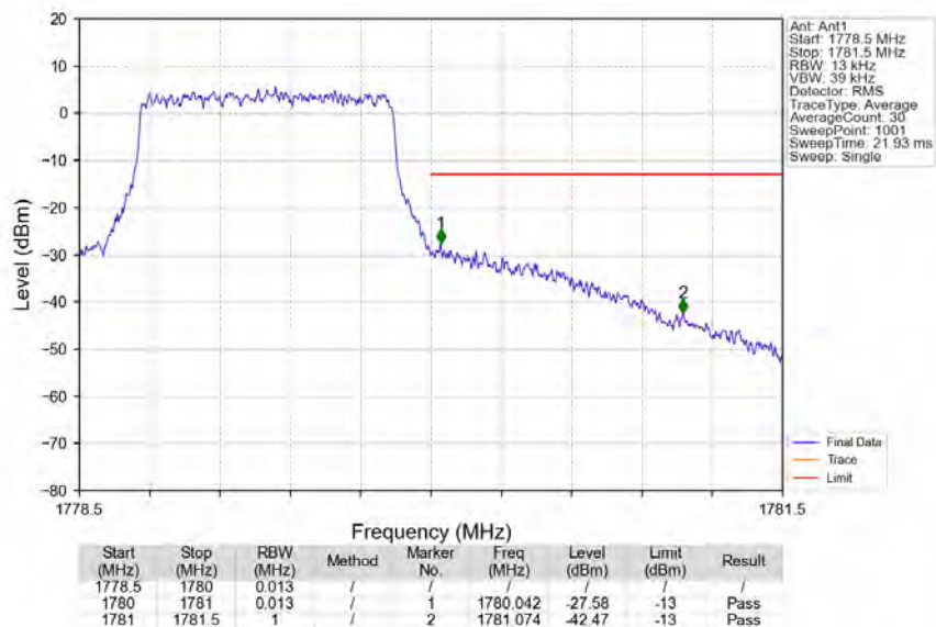
Band66_1.4MHz_16QAM_HCH_1779.3MHz_RB_6_0_NTNV
