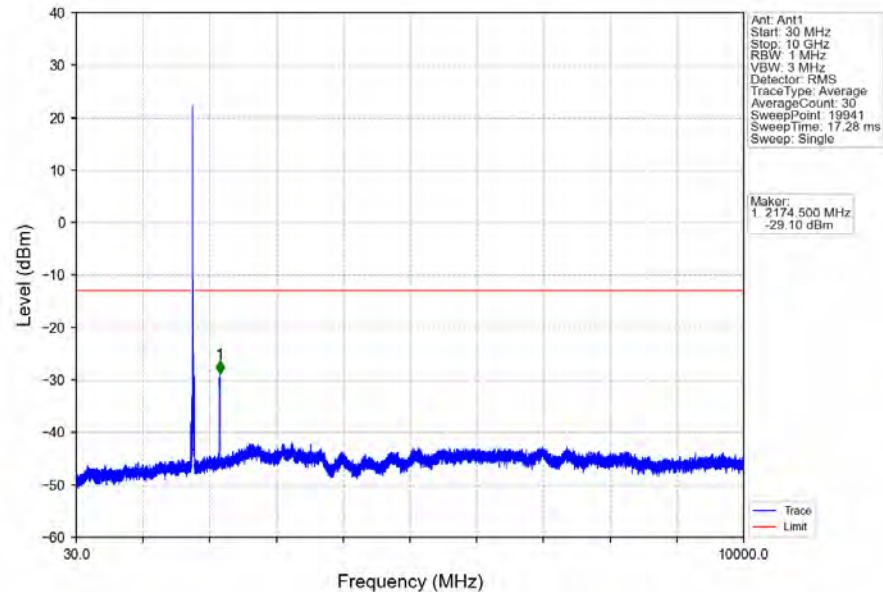
Band66_15MHz_64QAM_HCH_1772.5MHz_RB_1_0_NTNV
