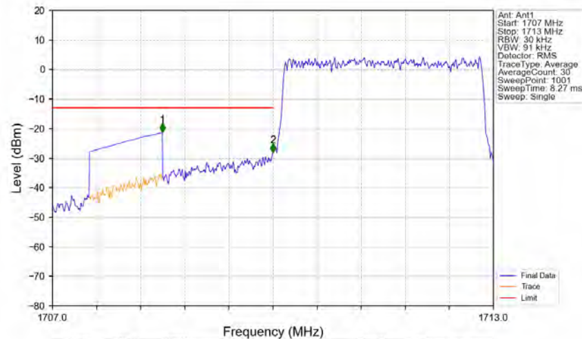
Band66_3MHz_64QAM_LCH_1711.5MHz_RB_15_0_NTNV
