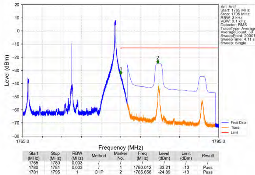
Band66_15MHz_QPSK_HCH_1772.5MHz_RB_1_74_NTNV
