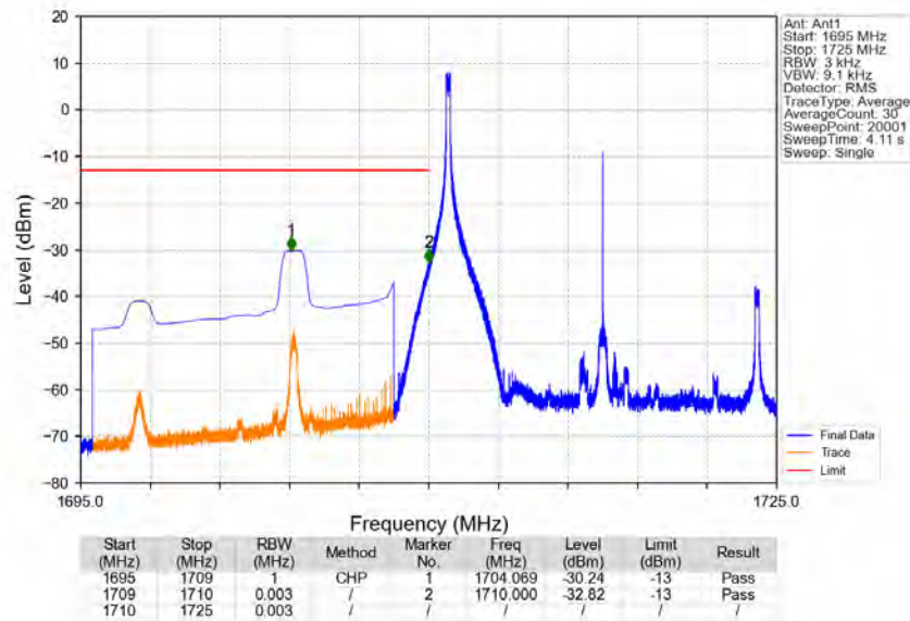
Band66_15MHz_16QAM_LCH_1717.5MHz_RB_1_0_NTNV
