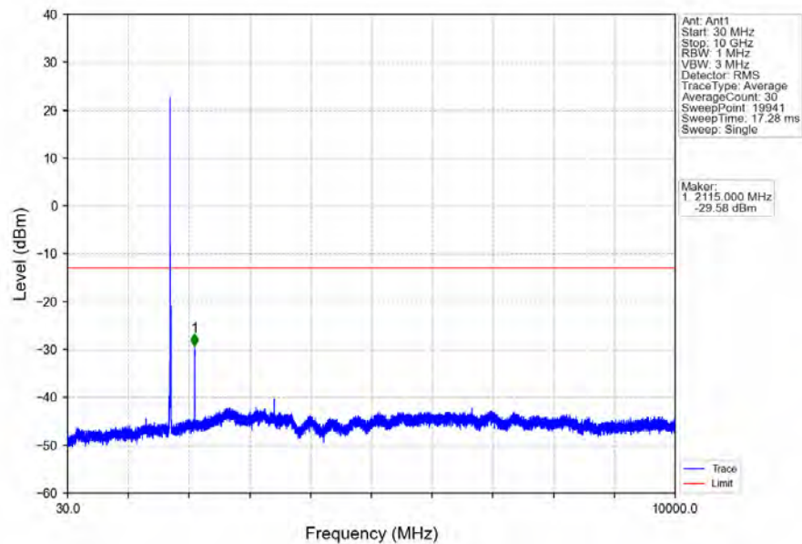
Band66_10MHz_16QAM_LCH_1715MHz_RB_1_0_NTNV
