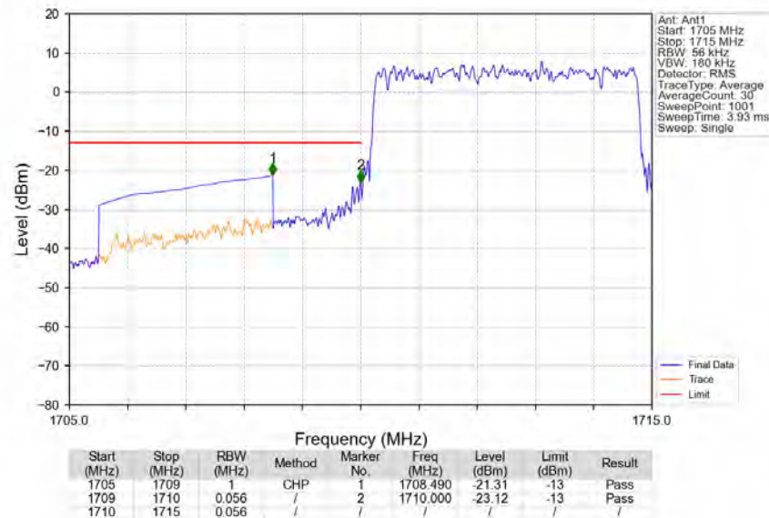
Band66_5MHz_QPSK_LCH_1712.5MHz_RB_25_0_NTNV
