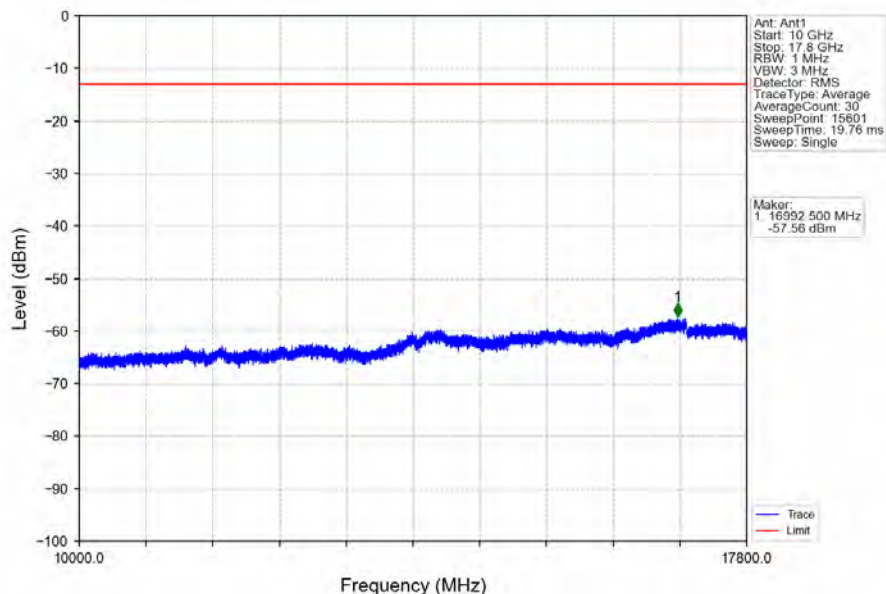
Band66_5MHz_64QAM_HCH_1777.5MHz_RB_1_0_NTNV
