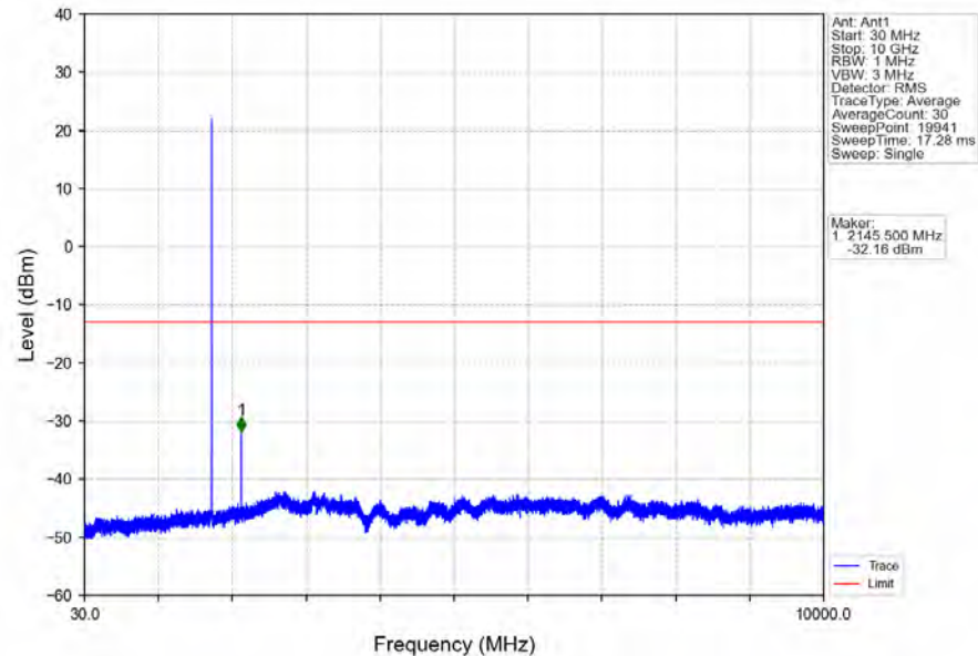
Band66_1.4MHz_64QAM_MCH_1745MHz_RB_1_0_NTNV
