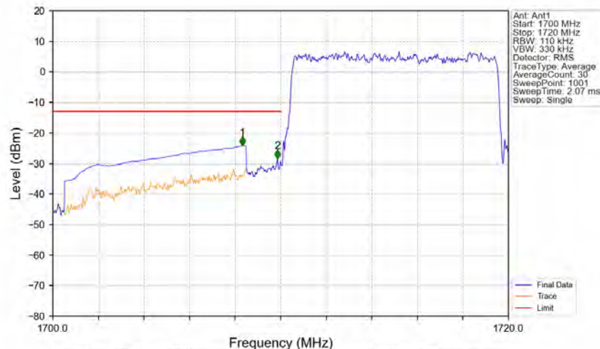
Band66_10MHz_QPSK_LCH_1715MHz_RB_50_0_NTNV
