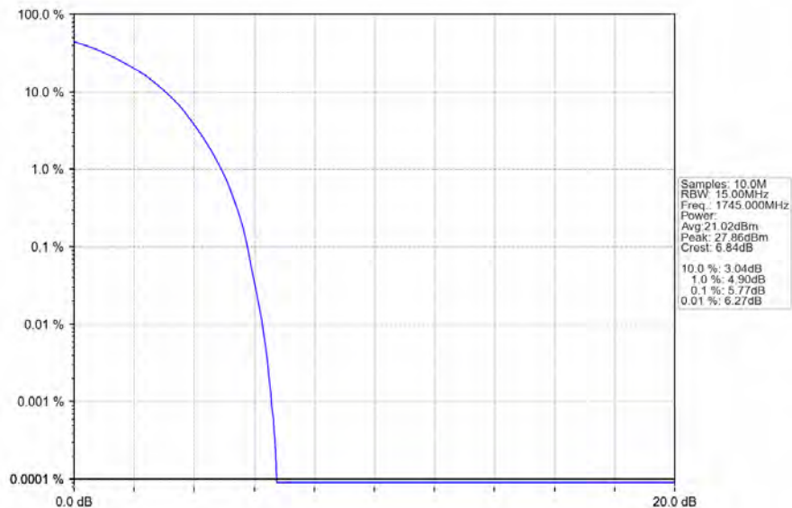
Band66_15MHz_64QAM_MCH_1745MHz_RB_75_0_NTNV
