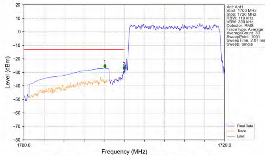
Band66_10MHz_16QAM_LCH_1715MHz_RB_50_0_NTNV
