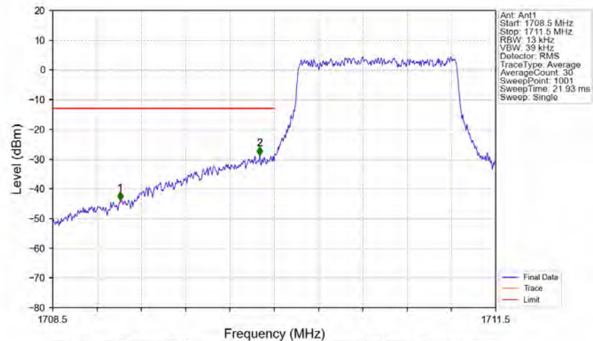
Band66_1.4MHz_64QAM_LCH_1710.7MHz_RB_6_0_NTNV
