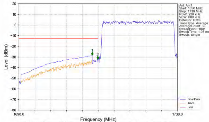
Band66_20MHz_64QAM_LCH_1720MHz_RB_100_0_NTNV
