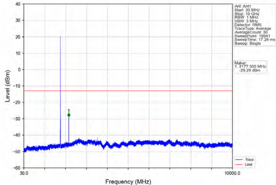
Band66_5MHz_64QAM_HCH_1777.5MHz_RB_1_0_NTNV
