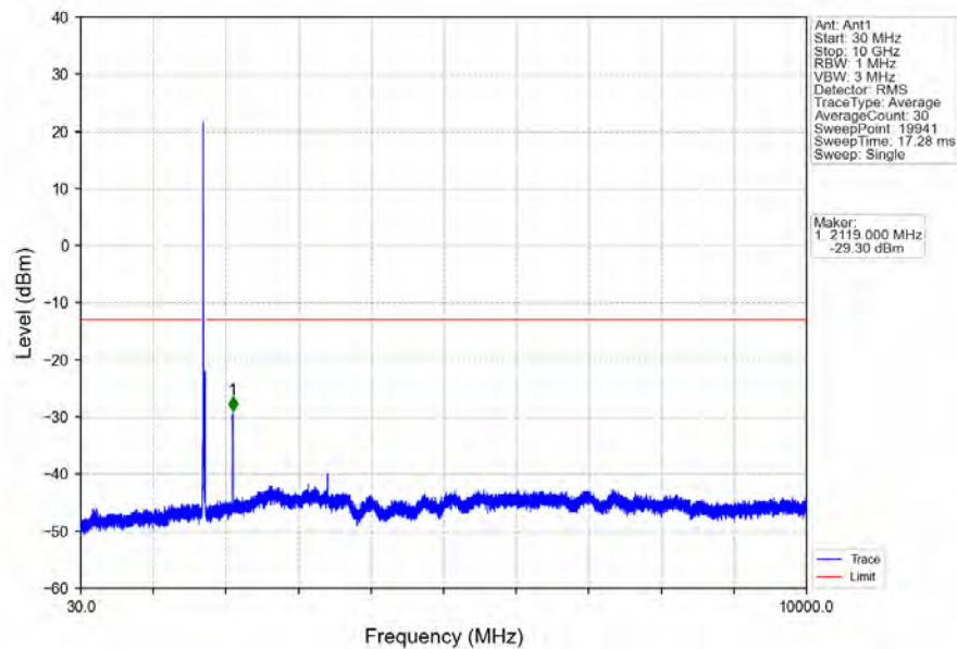
Band66_15MHz_64QAM_LCH_1717.5MHz_RB_1_0_NTNV
