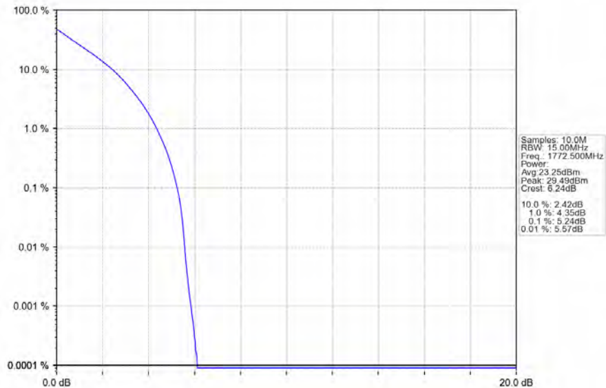
Band66_15MHz_QPSK_HCH_1772.5MHz_RB_75_0_NTNV
