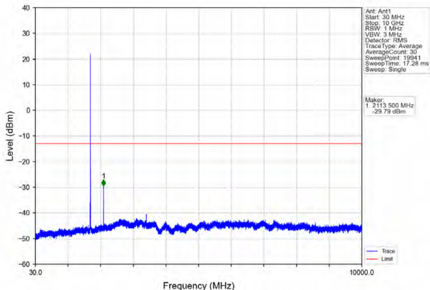
Band66_5MHz_64QAM_LCH_1712.5MHz_RB_1_0_NTNV
