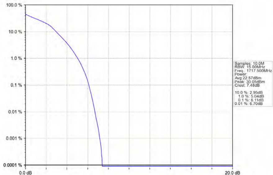
Band66_15MHz_16QAM_LCH_1717.5MHz_RB_75_0_NTNV
