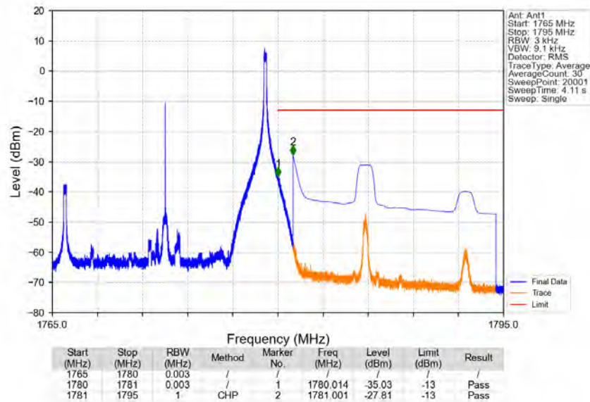
Band66_15MHz_64QAM_HCH_1772.5MHz_RB_1_74_NTNV
