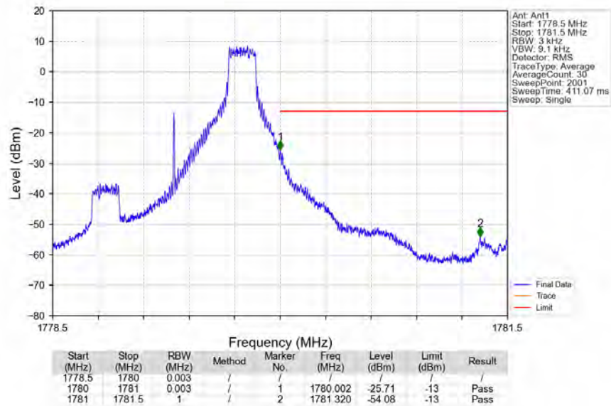
Band66_1.4MHz_QPSK_HCH_1779.3MHz_RB_1_5_NTNV
