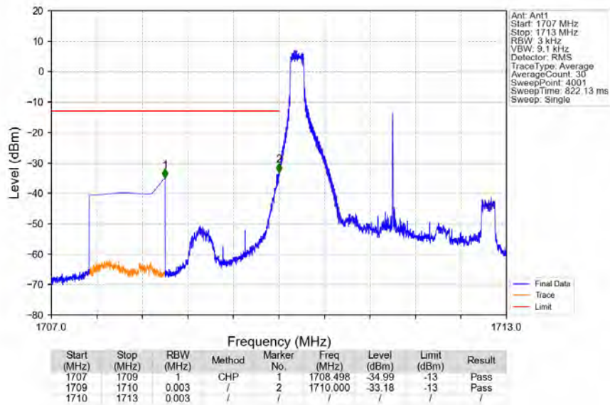
Band66_3MHz_64QAM_LCH_1711.5MHz_RB_1_0_NTNV
