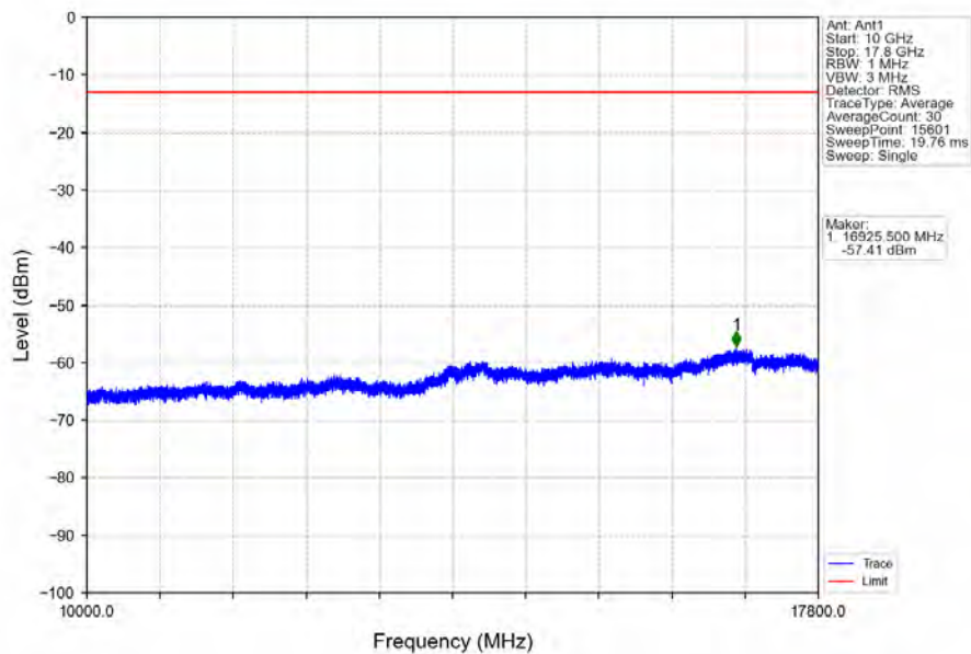
Band66_5MHz_16QAM_HCH_1777.5MHz_RB_1_0_NTNV
