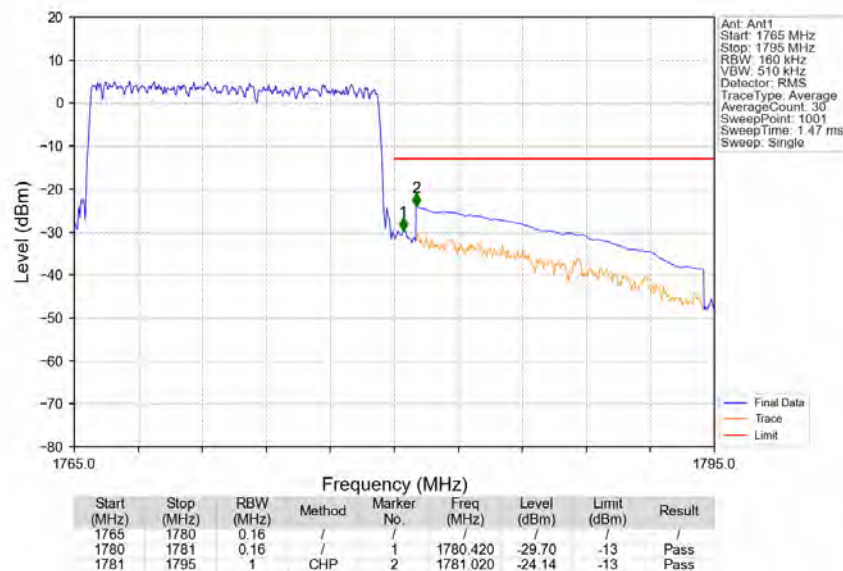
Band66_15MHz_16QAM_HCH_1772.5MHz_RB_75_0_NTNV
