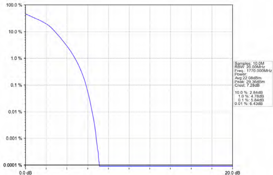
Band66_20MHz_16QAM_HCH_1770MHz_RB_100_0_NTNV
