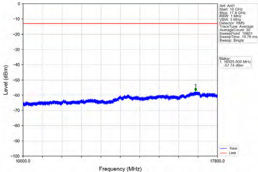
Band66_5MHz_QPSK_LCH_1712.5MHz_RB_25_0_NTNV
