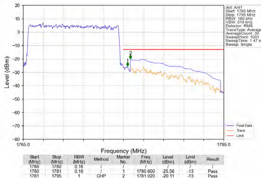
Band66_15MHz_QPSK_HCH_1772.5MHz_RB_75_0_NTNV
