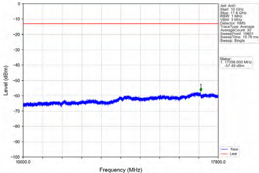
Band66_5MHz_64QAM_LCH_1712.5MHz_RB_25_0_NTNV
