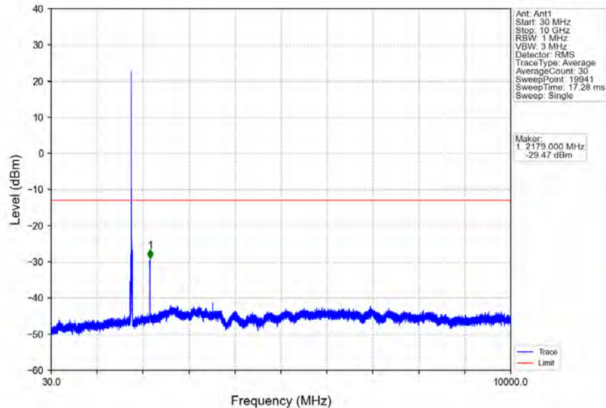
Band66_15MHz_QPSK_HCH_1772.5MHz_RB_1_0_NTNV
