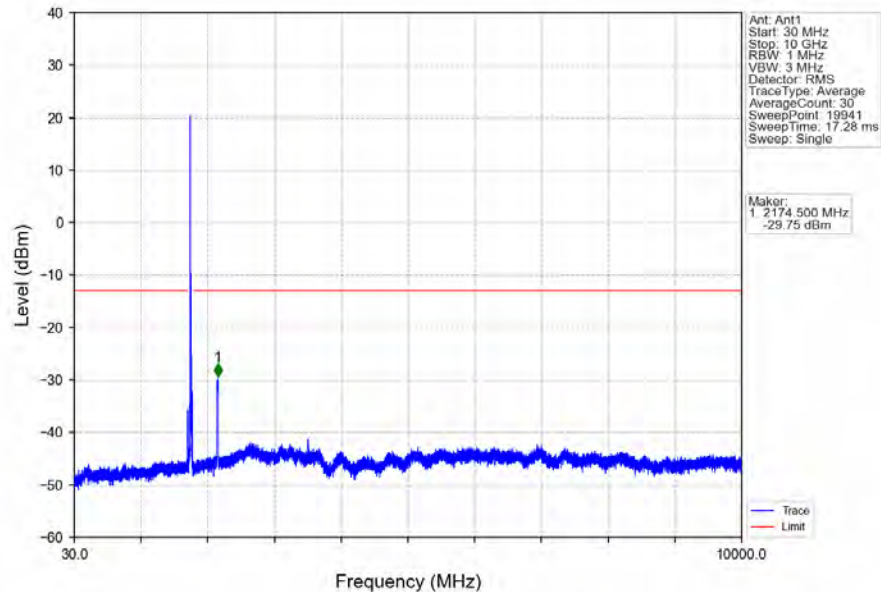
Band66_20MHz_64QAM_HCH_1770MHz_RB_1_0_NTNV
