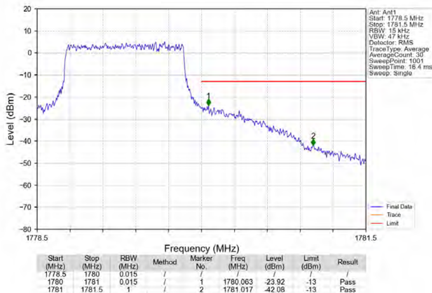
Band66_1.4MHz_64QAM_HCH_1779.3MHz_RB_6_0_NTNV
