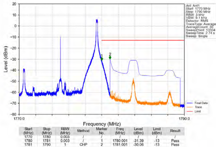
Band66_10MHz_64QAM_HCH_1775MHz_RB_1_49_NTNV
