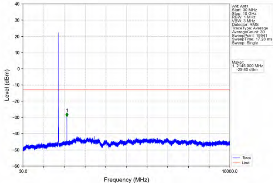
Band66_5MHz_16QAM_MCH_1745MHz_RB_1_0_NTNV
