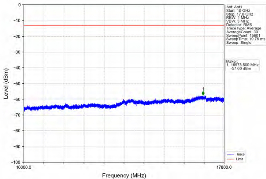
Band66_1.4MHz_16QAM_MCH_1745MHz_RB_1_0_NTNV
