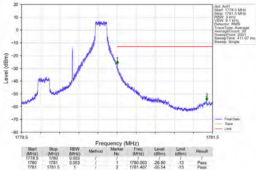
Band66_1.4MHz_16QAM_HCH_1779.3MHz_RB_1_5_NTNV
