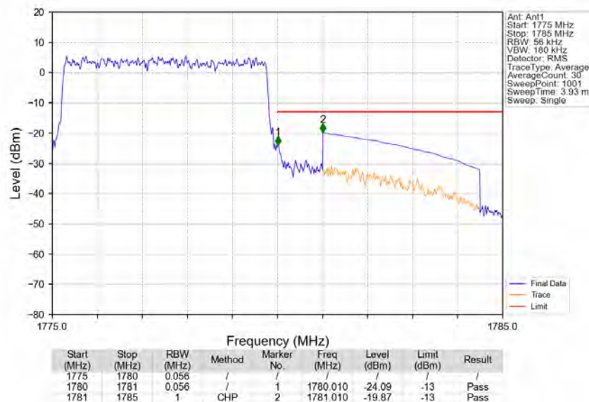
Band66_5MHz_16QAM_HCH_1777.5MHz_RB_25_0_NTNV
