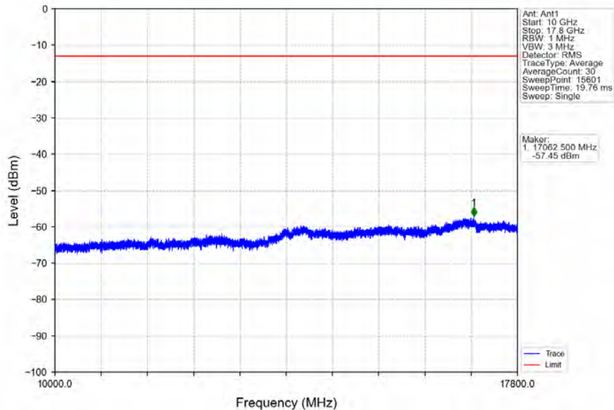
Band66_20MHz_64QAM_LCH_1720MHz_RB_100_0_NTNV
