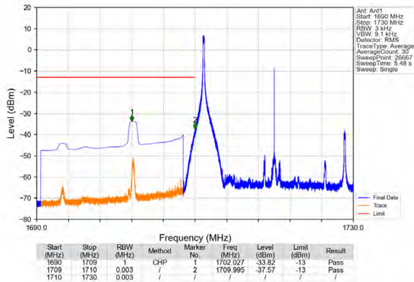
Band66_20MHz_64QAM_LCH_1720MHz_RB_1_0_NTNV
