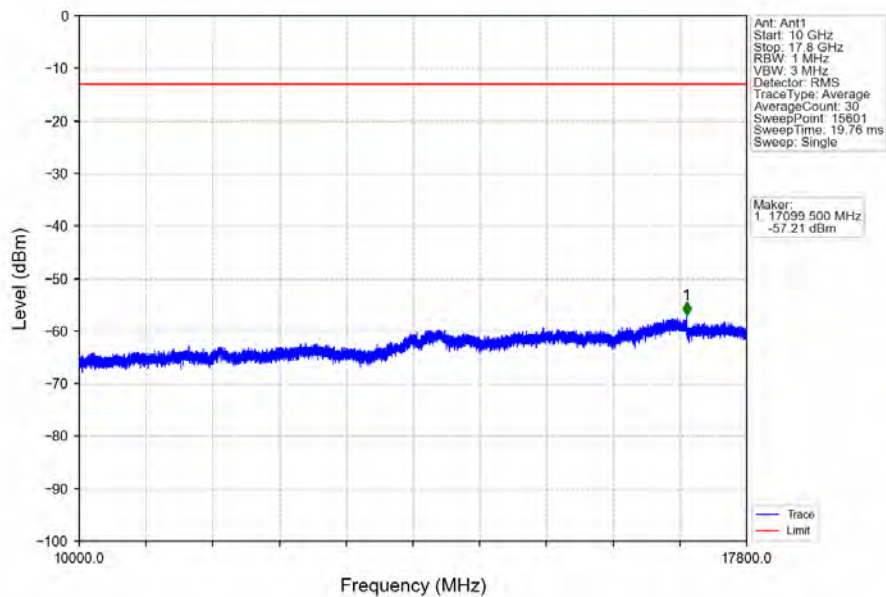
Band66_5MHz_64QAM_MCH_1745MHz_RB_1_0_NTNV
