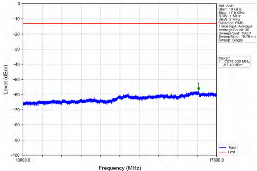
Band66_10MHz_16QAM_LCH_1715MHz_RB_50_0_NTNV
