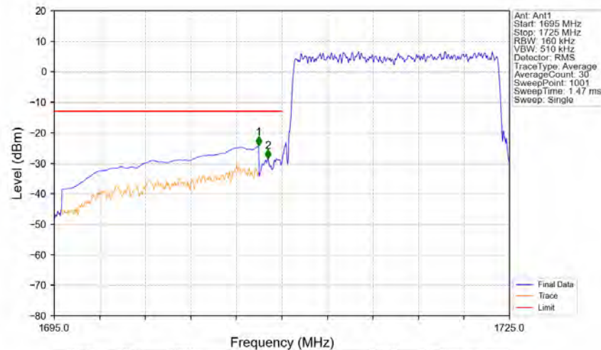
Band66_15MHz_QPSK_LCH_1717.5MHz_RB_75_0_NTNV
