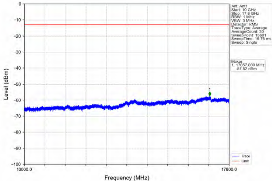
Band66_3MHz_64QAM_LCH_1711.5MHz_RB_15_0_NTNV
