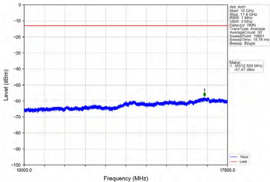
Band66_20MHz_16QAM_HCH_1770MHz_RB_1_0_NTNV
