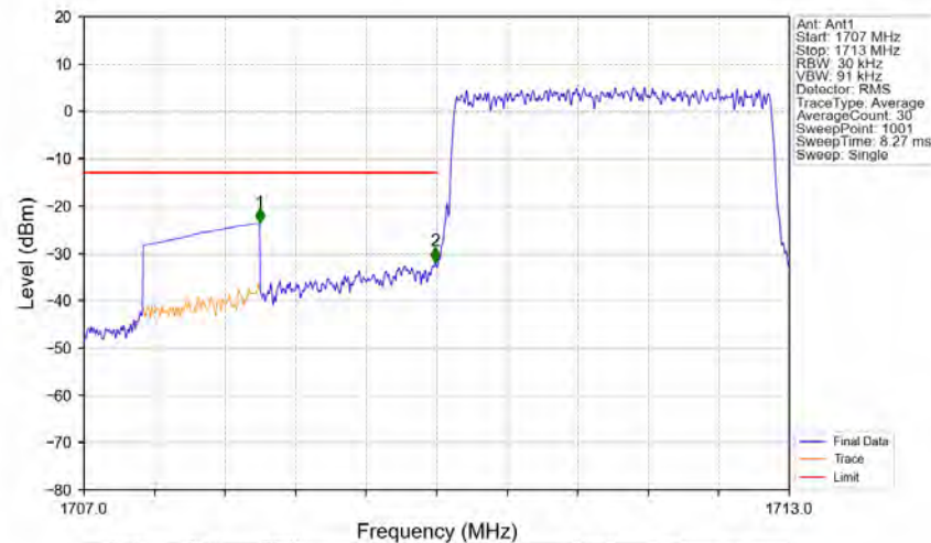
Band66_3MHz_16QAM_LCH_1711.5MHz_RB_15_0_NTNV
