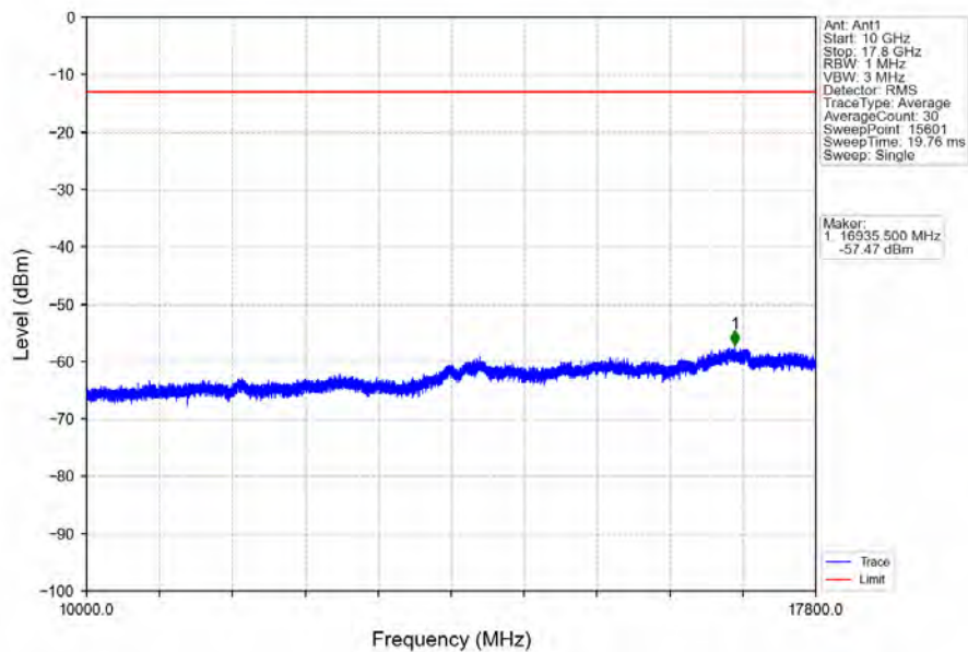
Band66_10MHz_64QAM_HCH_1775MHz_RB_1_0_NTNV
