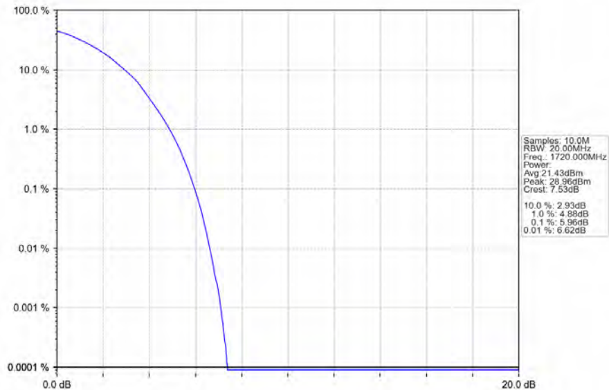
Band66_20MHz_64QAM_LCH_1720MHz_RB_100_0_NTNV
