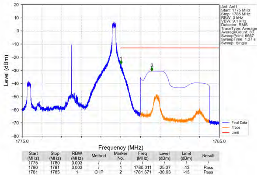
Band66_5MHz_64QAM_HCH_1777.5MHz_RB_1_24_NTNV
