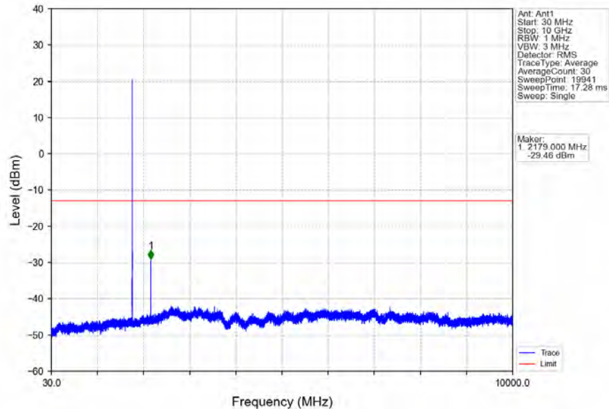
Band66_3MHz_64QAM_HCH_1778.5MHz_RB_1_0_NTNV
