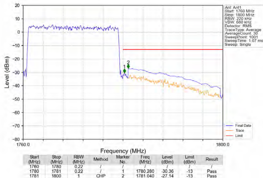
Band66_20MHz_16QAM_HCH_1770MHz_RB_100_0_NTNV
