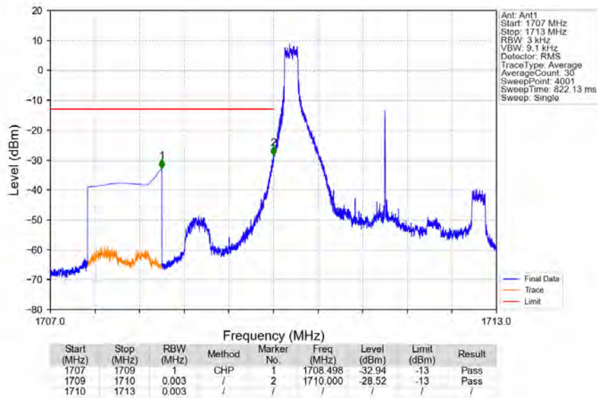
Band66_3MHz_16QAM_LCH_1711.5MHz_RB_1_0_NTNV
