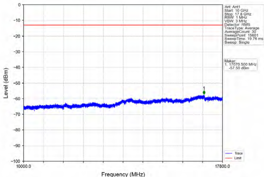
Band66_3MHz_64QAM_MCH_1745MHz_RB_1_0_NTNV
