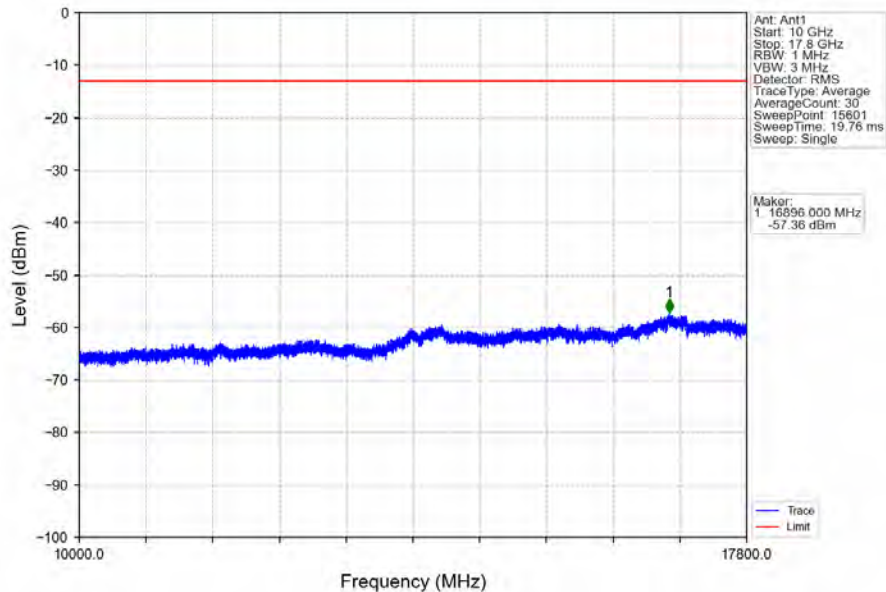
Band66_3MHz_QPSK_LCH_1711.5MHz_RB_15_0_NTNV
