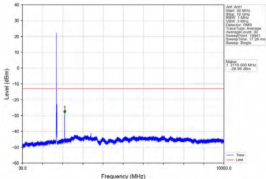
Band66_15MHz_16QAM_LCH_1717.5MHz_RB_1_0_NTNV
