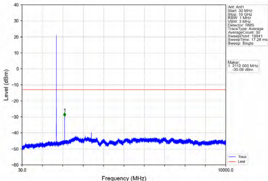
Band66_3MHz_64QAM_LCH_1711.5MHz_RB_1_0_NTNV
