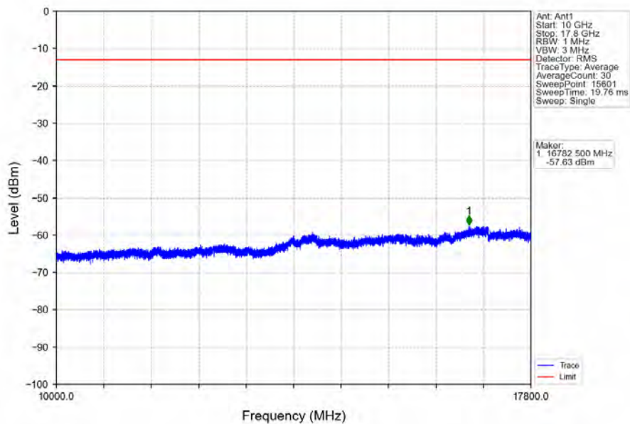
Band66_10MHz_16QAM_MCH_1745MHz_RB_1_0_NTNV
