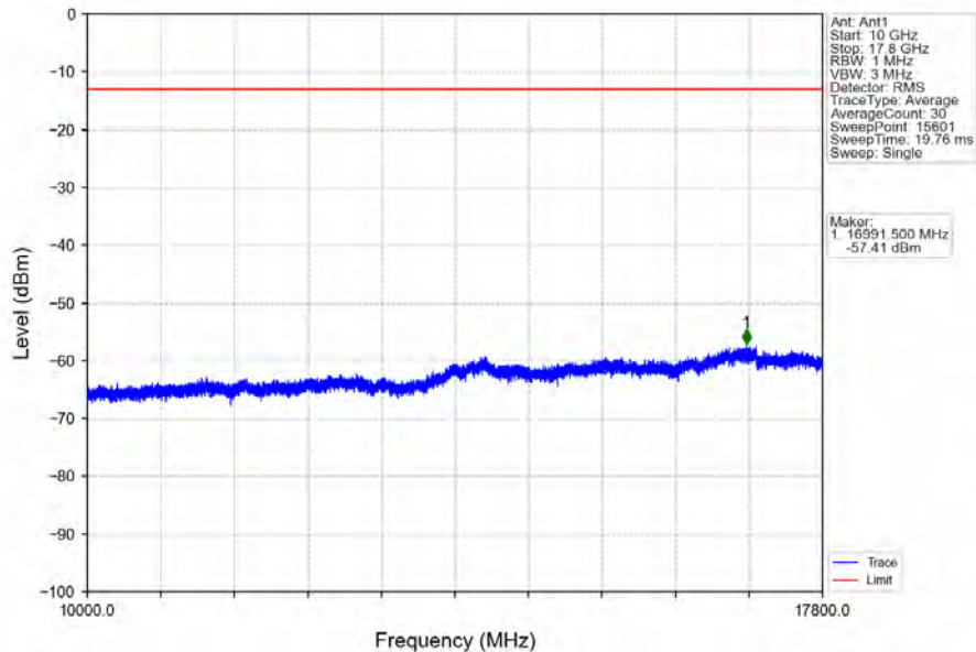
Band66_10MHz_QPSK_LCH_1715MHz_RB_50_0_NTNV
