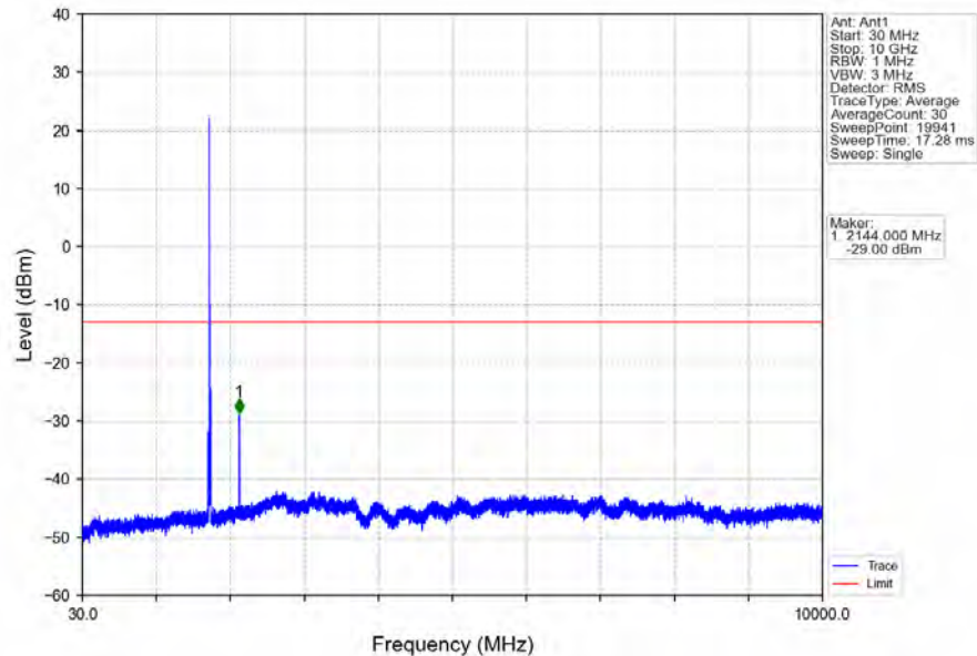
Band66_10MHz_64QAM_MCH_1745MHz_RB_1_0_NTNV
