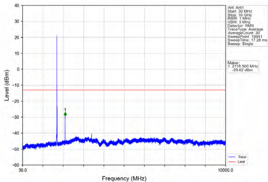
Band66_10MHz_64QAM_LCH_1715MHz_RB_1_0_NTNV
