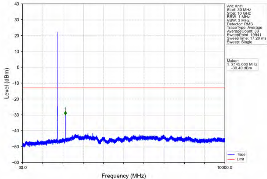
Band66_3MHz_16QAM_MCH_1745MHz_RB_1_0_NTNV
