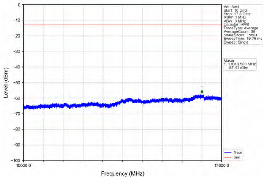
Band66_10MHz_QPSK_MCH_1745MHz_RB_1_0_NTNV
