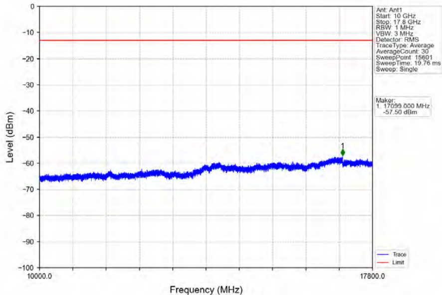
Band66_3MHz_16QAM_LCH_1711.5MHz_RB_15_0_NTNV
