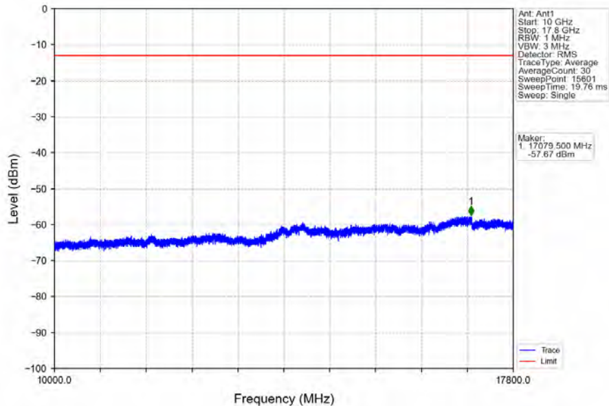
Band66_15MHz_QPSK_LCH_1717.5MHz_RB_75_0_NTNV
