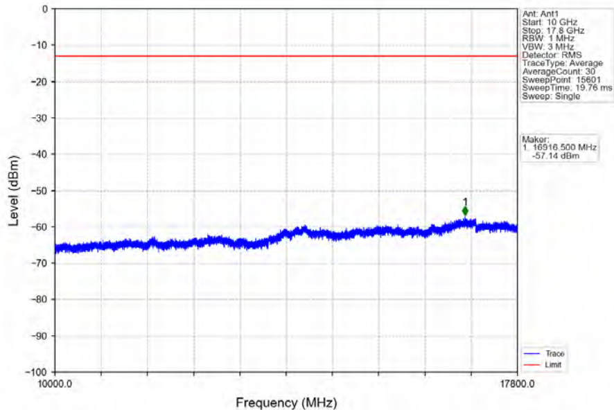
Band66_1.4MHz_16QAM_LCH_1710.7MHz_RB_6_0_NTNV
