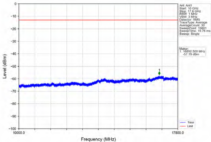
Band66_20MHz_64QAM_HCH_1770MHz_RB_1_0_NTNV
