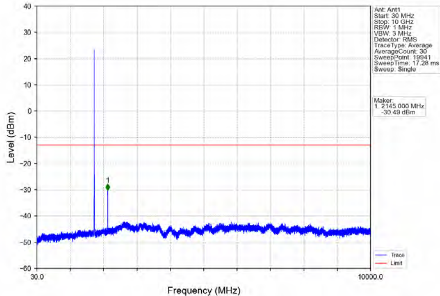
Band66_5MHz_QPSK_MCH_1745MHz_RB_1_0_NTNV
