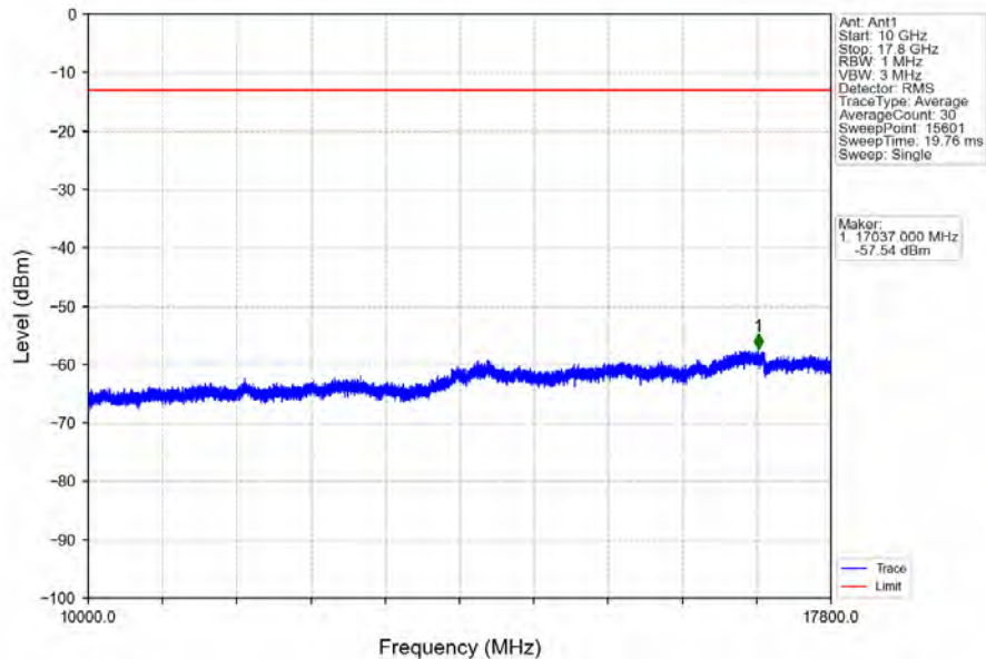
Band66_1.4MHz_64QAM_LCH_1710.7MHz_RB_6_0_NTNV
