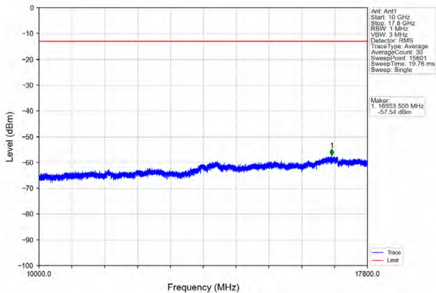
Band66_10MHz_64QAM_MCH_1745MHz_RB_1_0_NTNV
