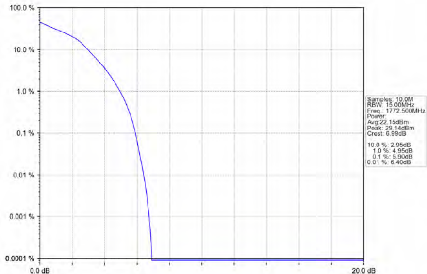
Band66_15MHz_16QAM_HCH_1772.5MHz_RB_75_0_NTNV
