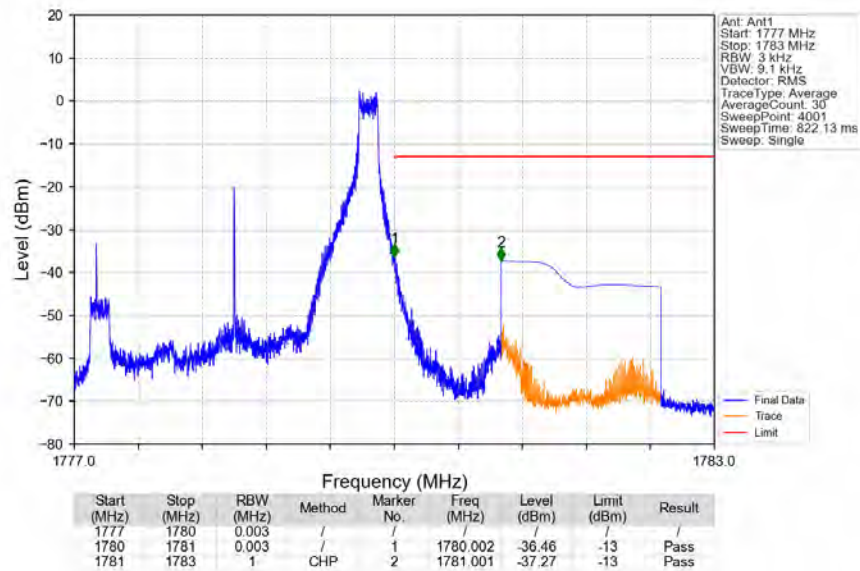
Band66_3MHz_64QAM_HCH_1778.5MHz_RB_1_14_NTNV
