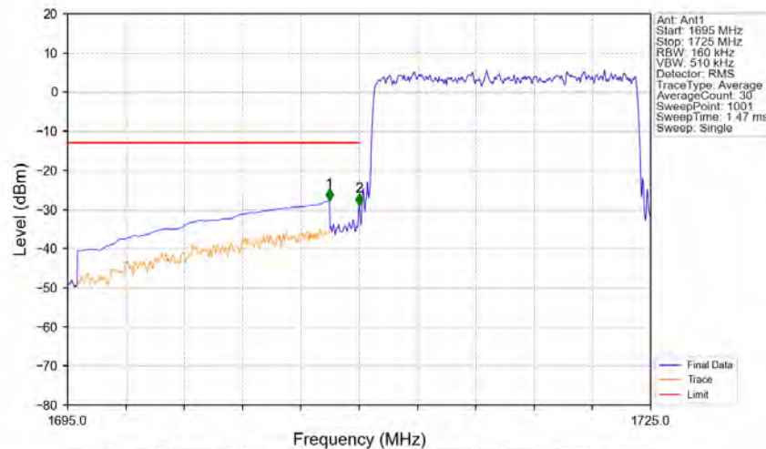
Band66_15MHz_16QAM_LCH_1717.5MHz_RB_75_0_NTNV
