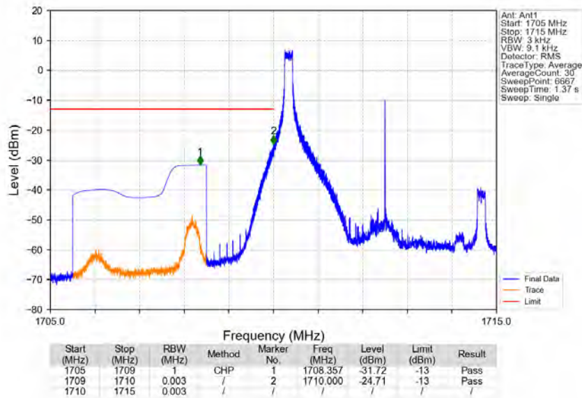
Band66_5MHz_64QAM_LCH_1712.5MHz_RB_1_0_NTNV
