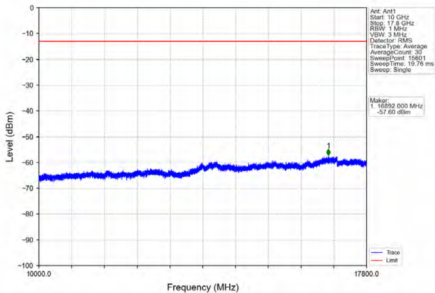
Band66_15MHz_16QAM_HCH_1772.5MHz_RB_1_0_NTNV
