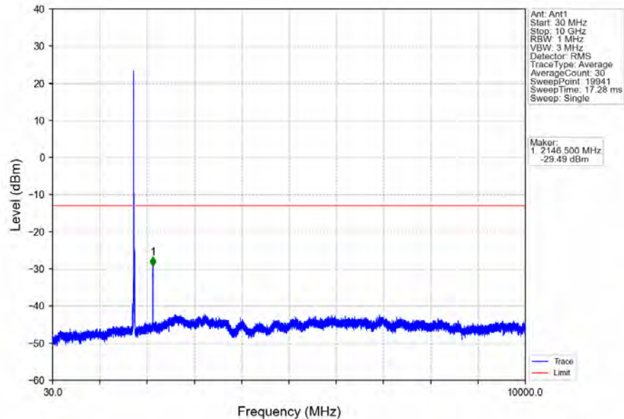
Band66_15MHz_16QAM_MCH_1745MHz_RB_1_0_NTNV
