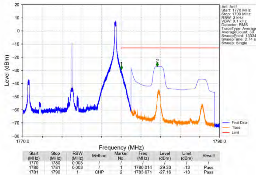
Band66_10MHz_16QAM_HCH_1775MHz_RB_1_49_NTNV
