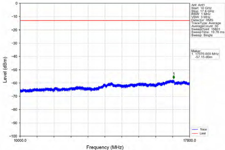
Band66_5MHz_16QAM_LCH_1712.5MHz_RB_25_0_NTNV
