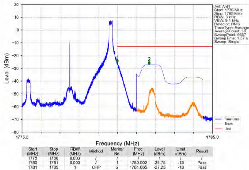
Band66_5MHz_16QAM_HCH_1777.5MHz_RB_1_24_NTNV
