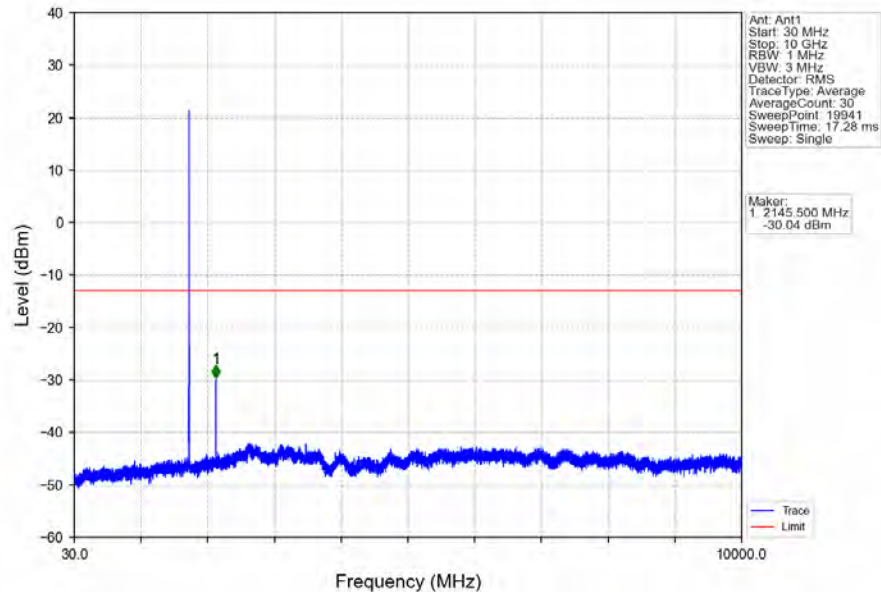
Band66_3MHz_64QAM_MCH_1745MHz_RB_1_0_NTNV
