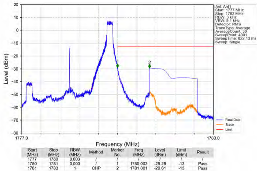
Band66_3MHz_16QAM_HCH_1778.5MHz_RB_1_14_NTNV
