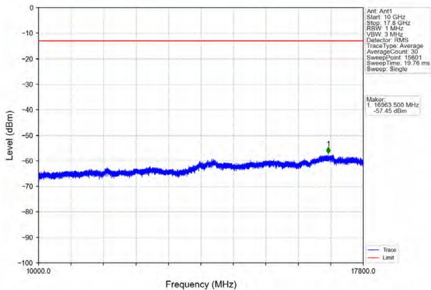
Band66_3MHz_16QAM_HCH_1778.5MHz_RB_1_0_NTNV
