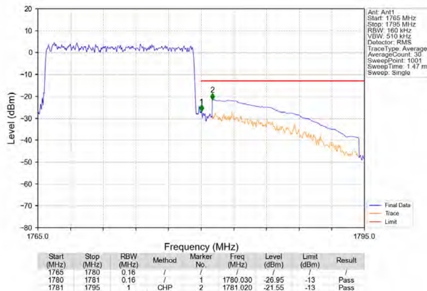
Band66_15MHz_64QAM_HCH_1772.5MHz_RB_75_0_NTNV
