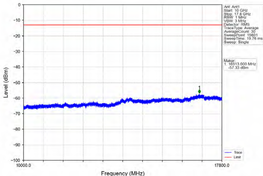
Band66_15MHz_QPSK_HCH_1772.5MHz_RB_1_0_NTNV
