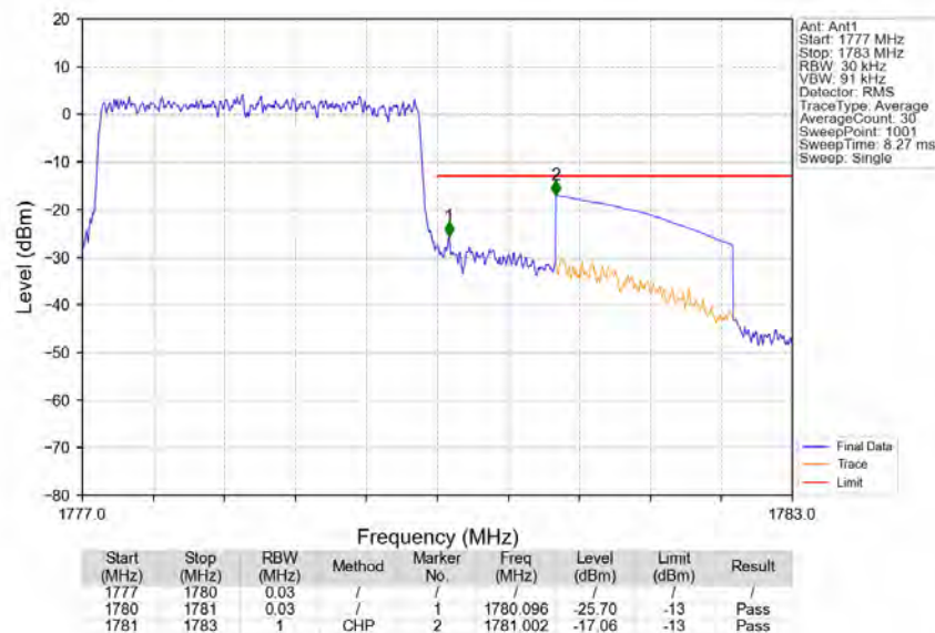
Band66_3MHz_64QAM_HCH_1778.5MHz_RB_15_0_NTNV
