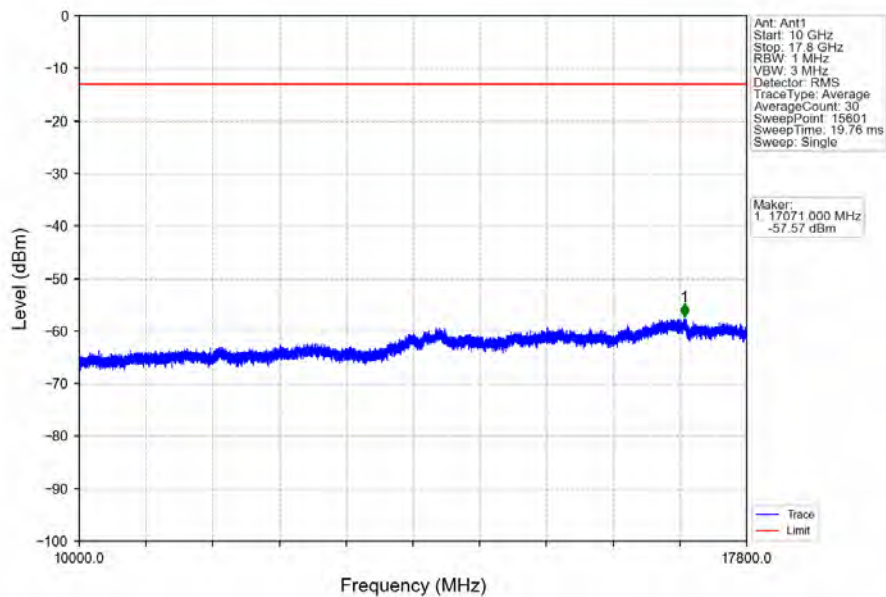
Band66_15MHz_64QAM_MCH_1745MHz_RB_1_0_NTNV
