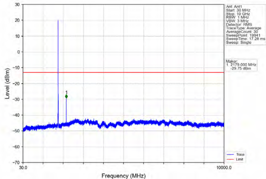
Band66_10MHz_64QAM_HCH_1775MHz_RB_1_0_NTNV
