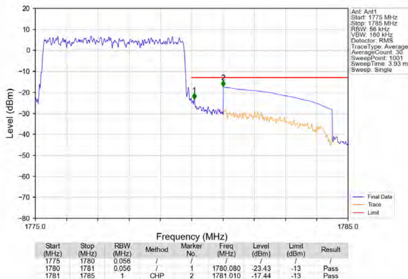
Band66_5MHz_QPSK_HCH_1777.5MHz_RB_25_0_NTNV
