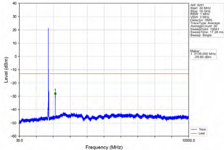
Band66_20MHz_64QAM_MCH_1745MHz_RB_1_0_NTNV
