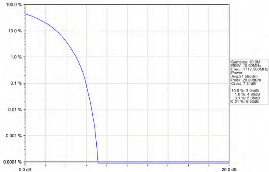
Band66_15MHz_64QAM_LCH_1717.5MHz_RB_75_0_NTNV
