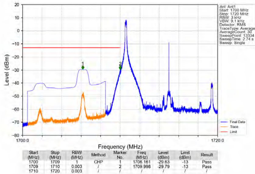
Band66_10MHz_16QAM_LCH_1715MHz_RB_1_0_NTNV
