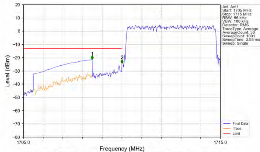
Band66_5MHz_64QAM_LCH_1712.5MHz_RB_25_0_NTNV
