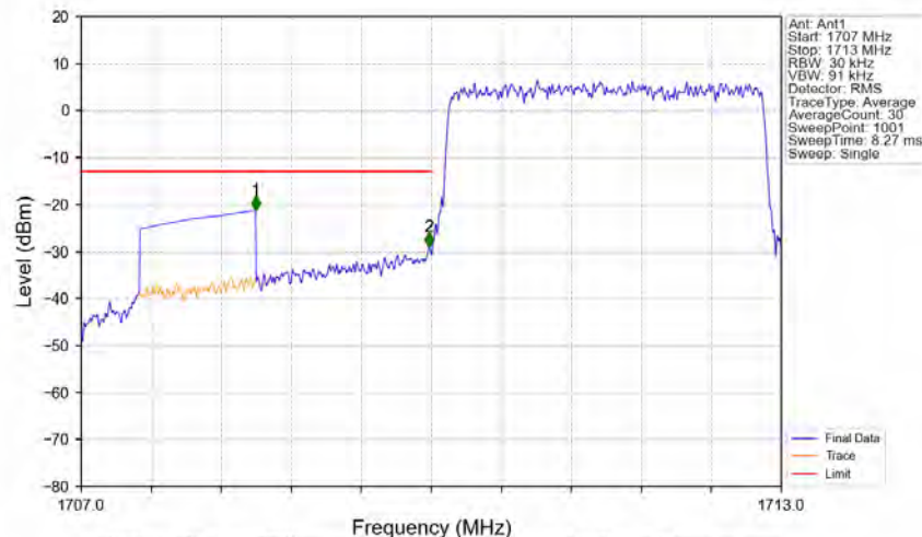
Band66_3MHz_QPSK_LCH_1711.5MHz_RB_15_0_NTNV
