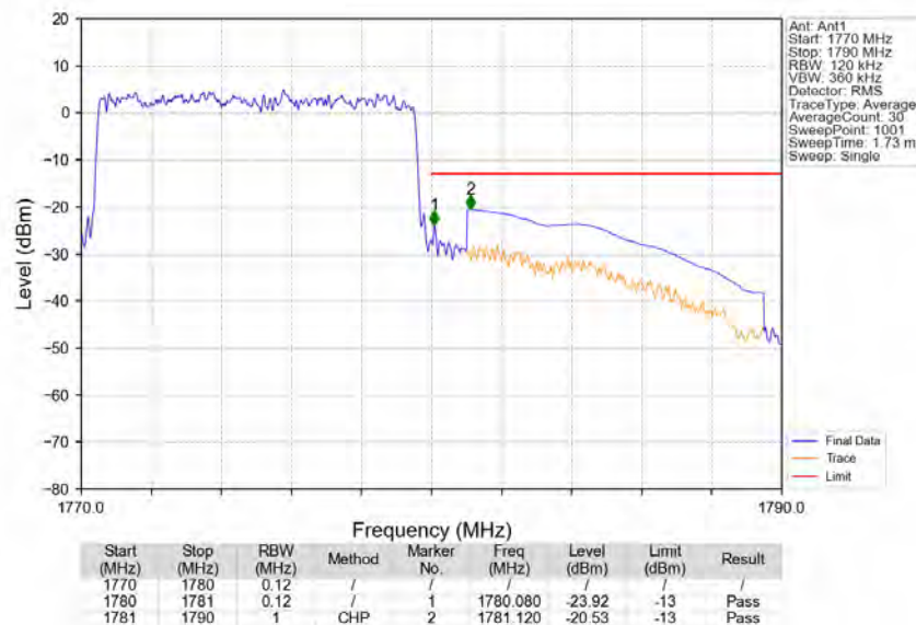
Band66_10MHz_64QAM_HCH_1775MHz_RB_50_0_NTNV
