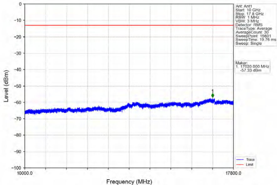
Band66_10MHz_64QAM_LCH_1715MHz_RB_50_0_NTNV
