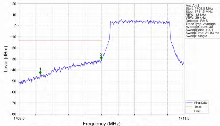
Band66_1.4MHz_16QAM_LCH_1710.7MHz_RB_6_0_NTNV
