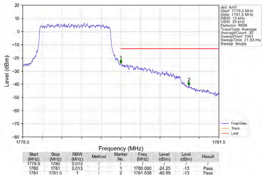
Band66_1.4MHz_QPSK_HCH_1779.3MHz_RB_6_0_NTNV
