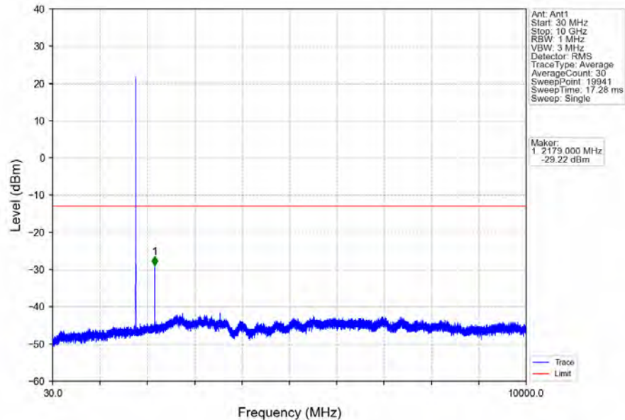
Band66_3MHz_16QAM_HCH_1778.5MHz_RB_1_0_NTNV
