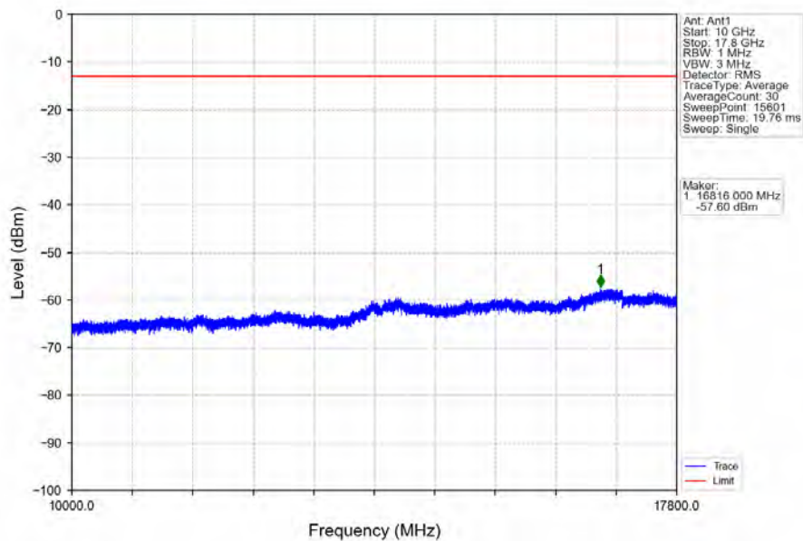
Band66_5MHz_16QAM_MCH_1745MHz_RB_1_0_NTNV
