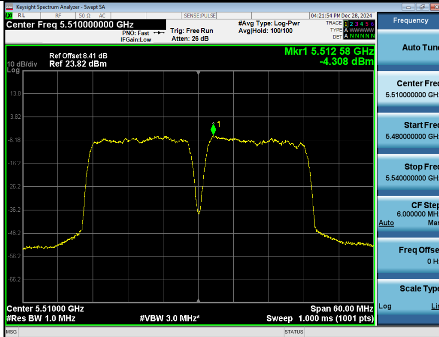
Power Spectral Density NVNT_ANT1_802_11n(HT40)_5510
