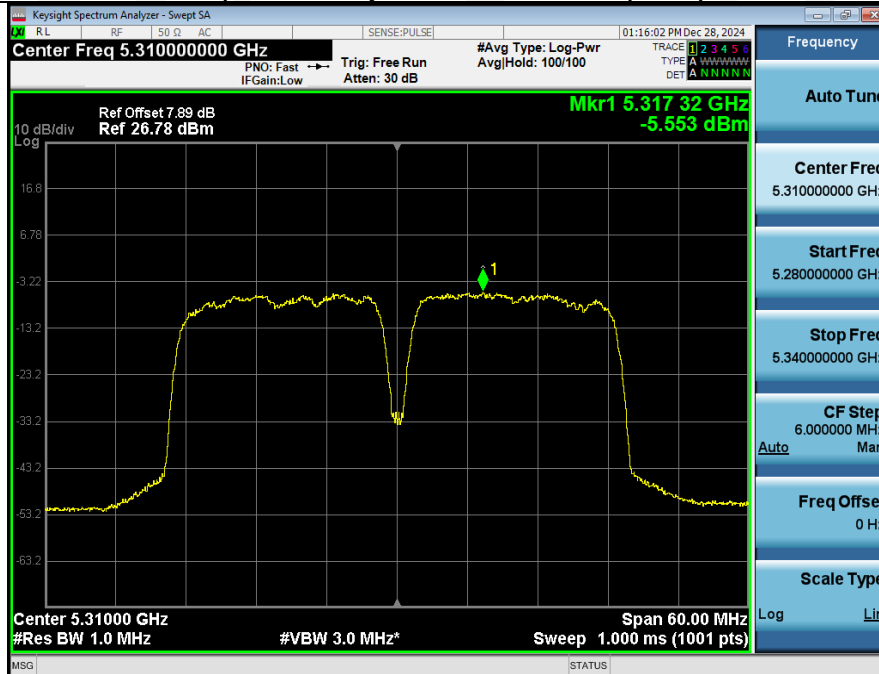
Power Spectral Density_NVNT_ANT2_802_11ac(VHT40)_5310
