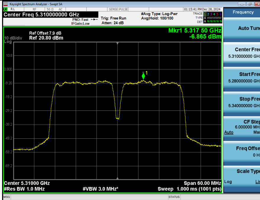
Power Spectral Density_NVNT_ANT1_802_11ac(VHT40)_5310
