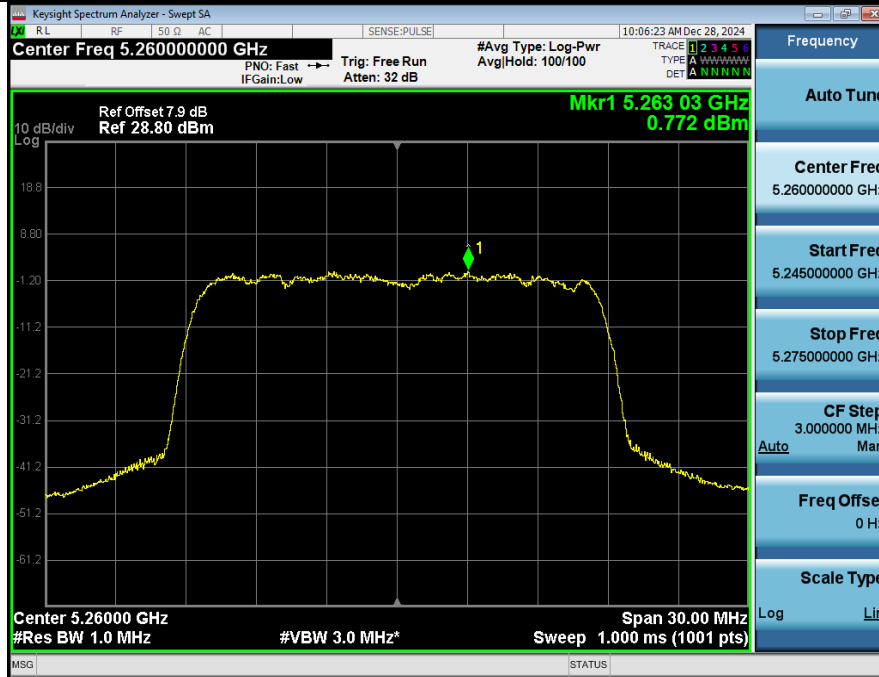
Power_Spectral_Density_NVNT_ANT2_802_11a_5260
