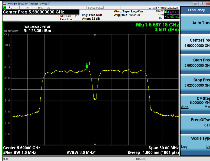
Power Spectral Density NVNT_ANT2_802_11ac(VHT40)_5590
