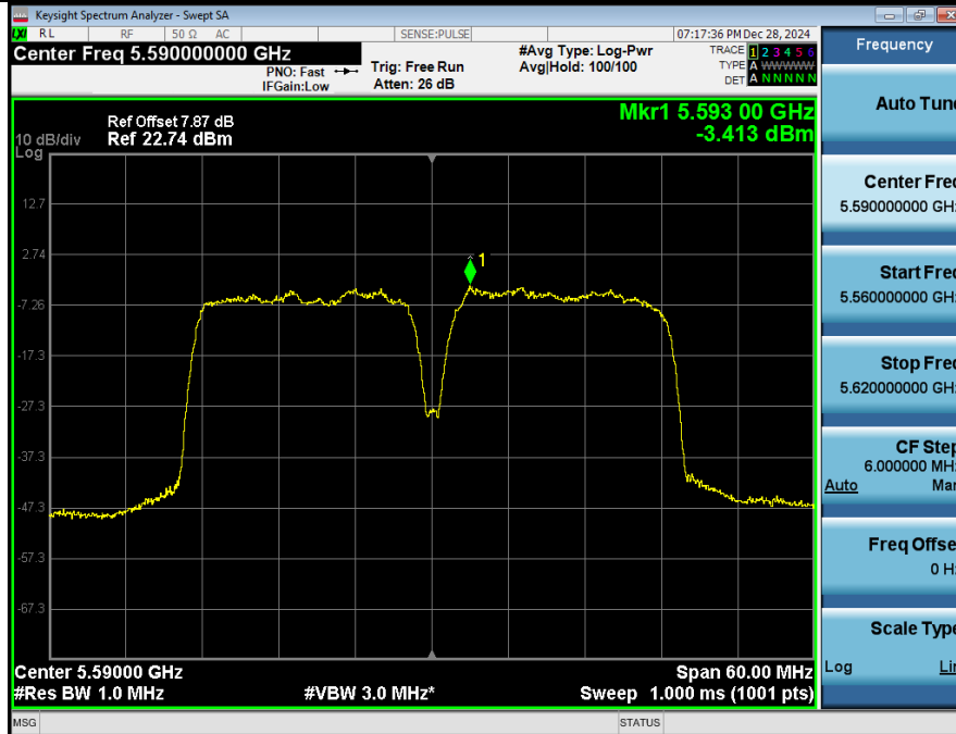
Power Spectral Density NVNT_ANT1_802_11ac(VHT40)_5590
