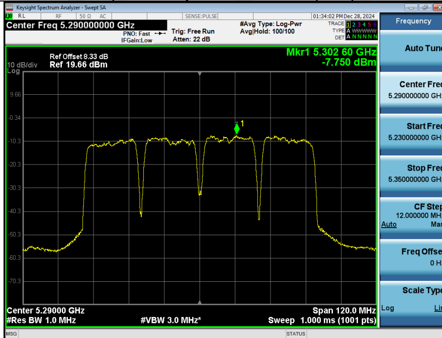
Power Spectral Density_NVNT_ANT2_802_11ac(VHT80)_5290
