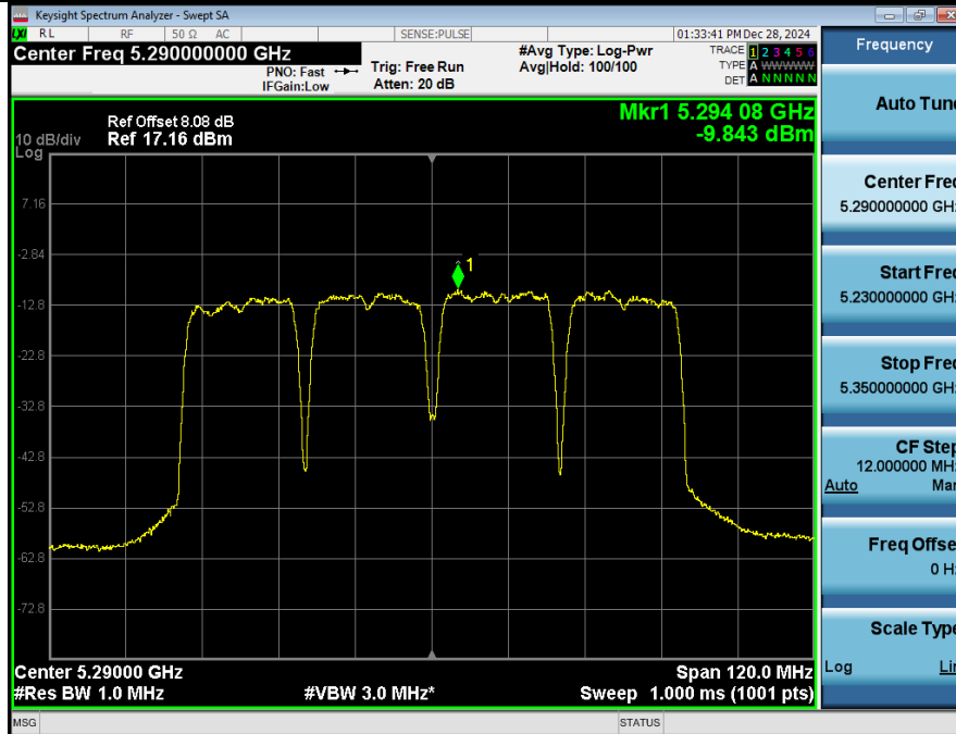
Power Spectral Density_NVNT_ANT1_802_11ac(VHT80)_5290
