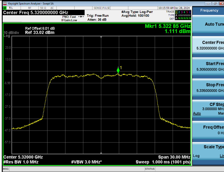
Power_Spectral_Density_NVNT_ANT2_802_11a_5320
