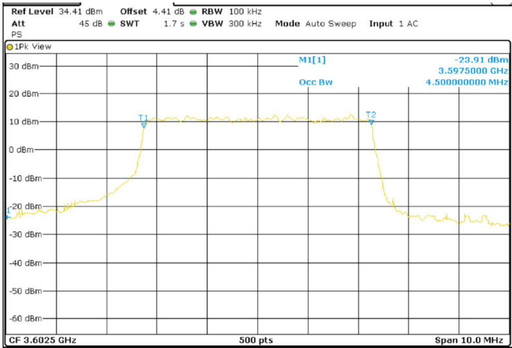
Band 43_BW5M_16QAM_Low Channel
