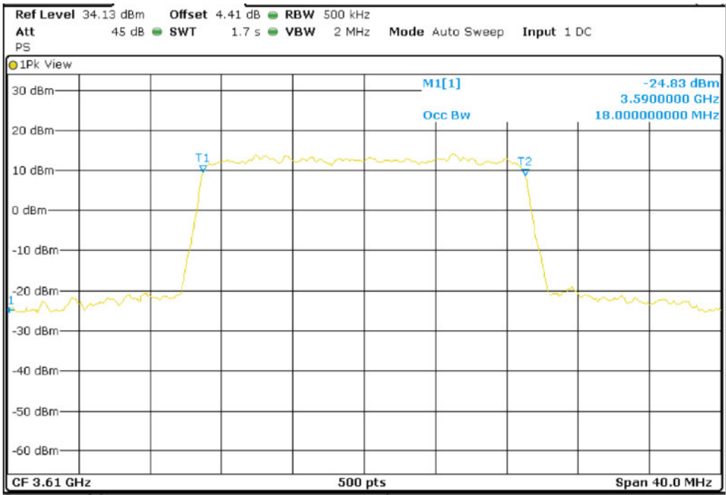
Band 43_BW20M_16QAM_Low Channel
