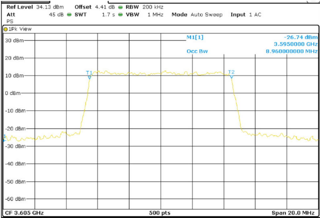
Band 43_BW10M_16QAM_Low Channel
