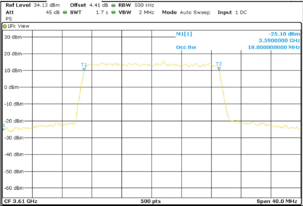
Band 43_BW20M_QPSK_Low Channel
