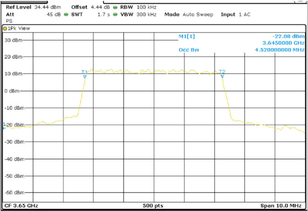
Band 43_BW5M_16QAM_Middle Channel
