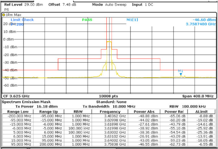
Band 48_BW10M_Middle Channel
