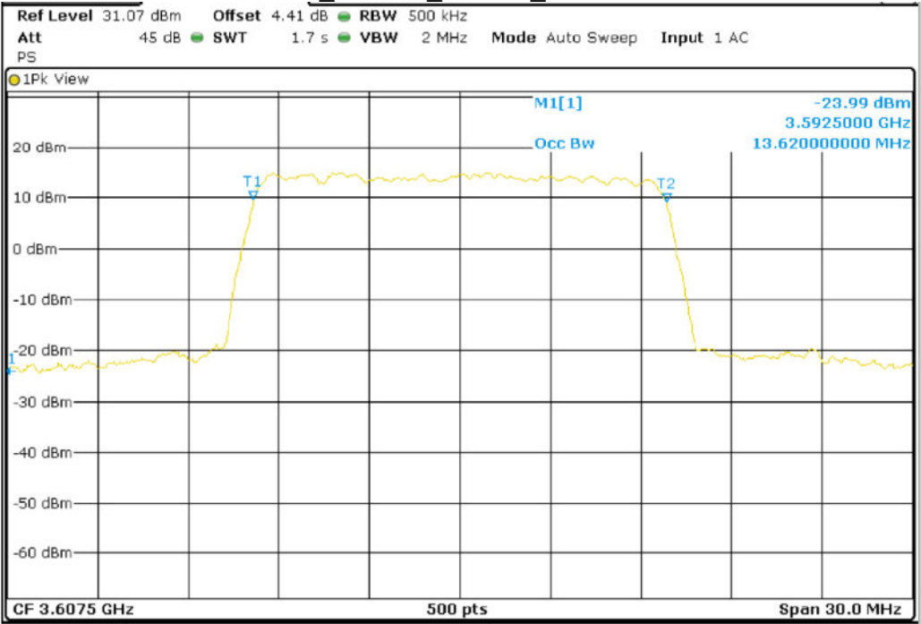
Band 43_BW15M_16QAM_Low Channel
