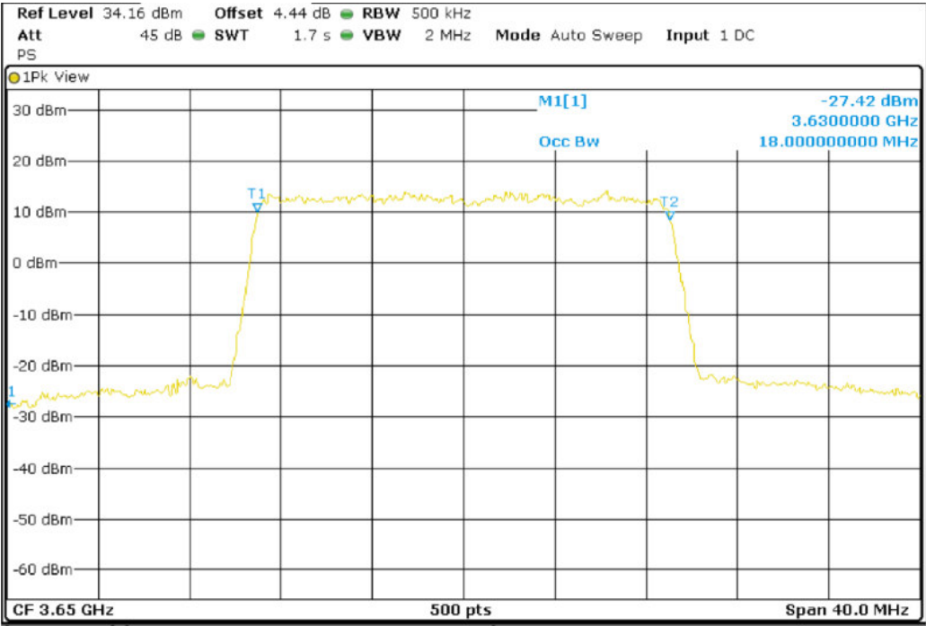
Band 43_BW20M_16QAM_Middle Channel
