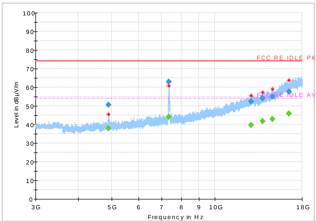
Fig.76 Radiated Spurious Emission (802.11 n-40MHz,Ch9,3GHz~18GHz)
