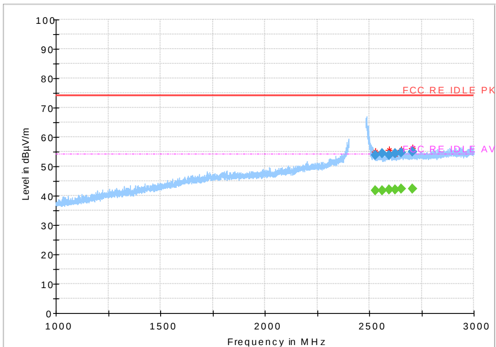
Fig.75 Radiated Spurious Emission (802.11 n-40MHz,Ch9,1GHz~3GHz)
