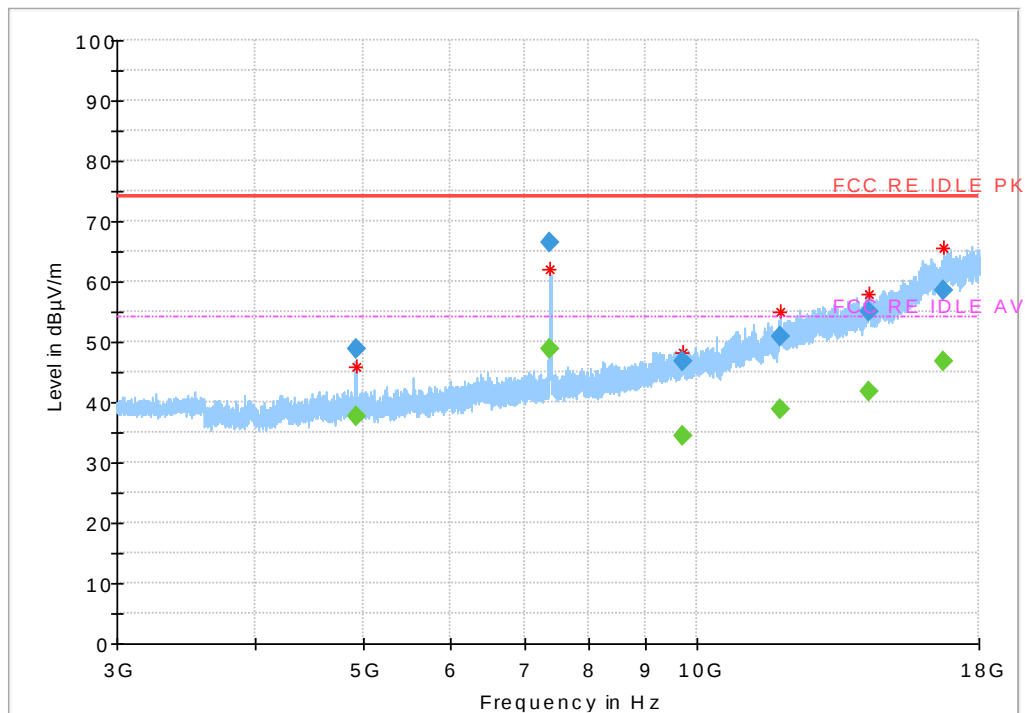
Fig. 71 Radiated Spurious Emission (802.11 n-20MHz,Ch11,3GHz~18GHz)
