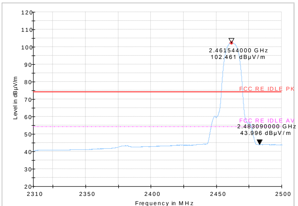
Fig.58 Radiated emission (Power): 802.11b, high channel
