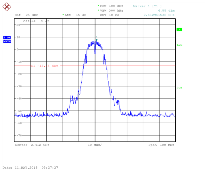
Fig.33 Conducted Spurious Emission (802.11b, Ch1)
