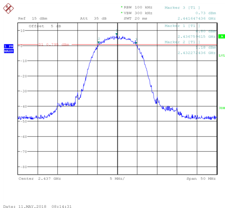
Fig.14 Occupied 6dB Bandwidth (802.11b, Ch6)
