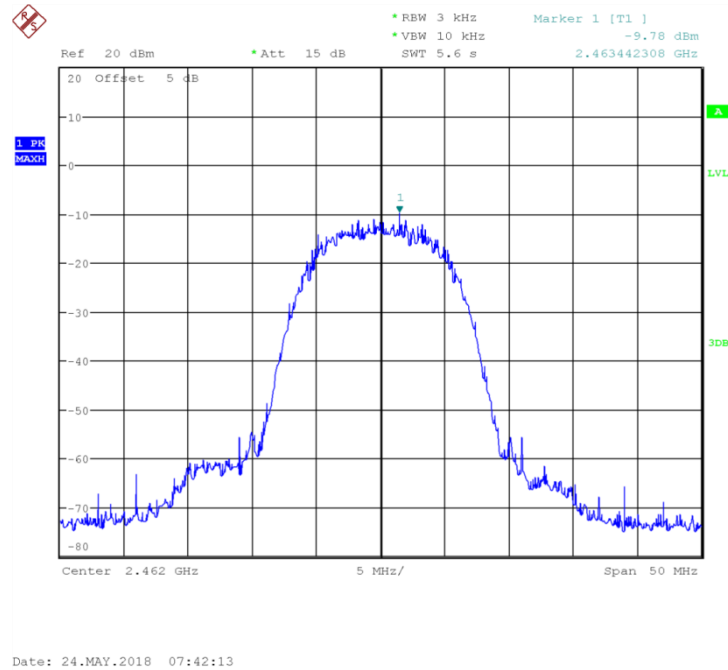
Fig 3. Power Spectral Density (802.1b,Ch11)
