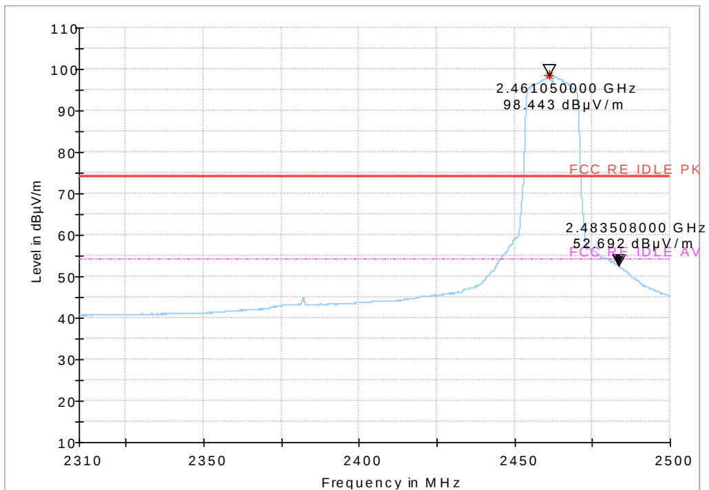
Fig.63 Radiated emission (Power): 802.11g, high channel
