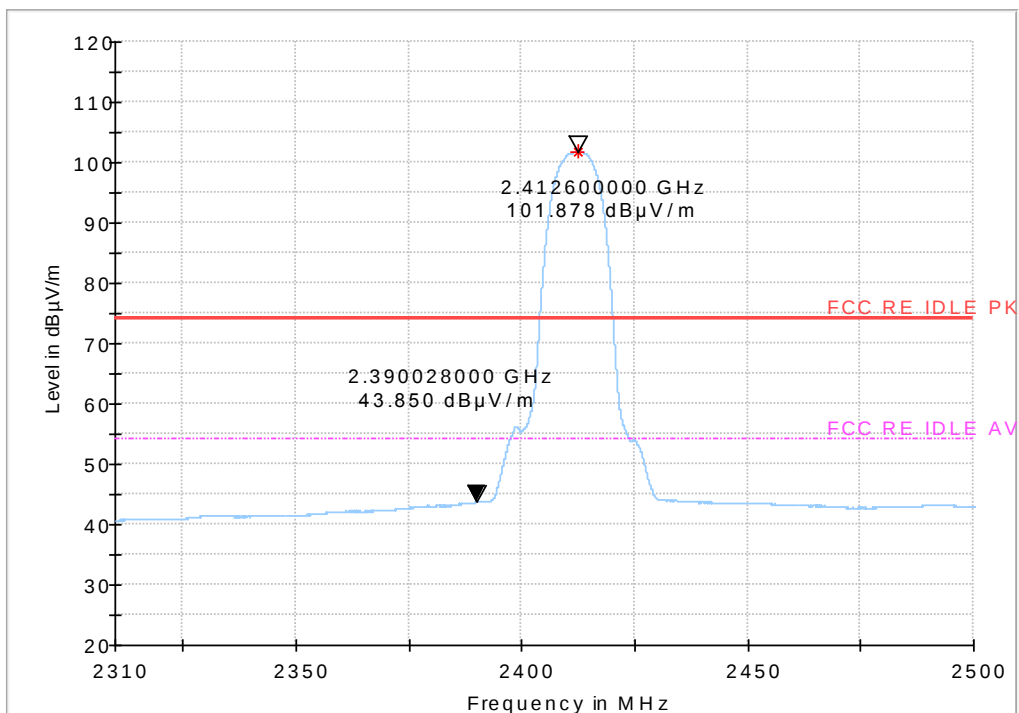
Fig.57 Radiated emission (Power): 802.11b, low channel
