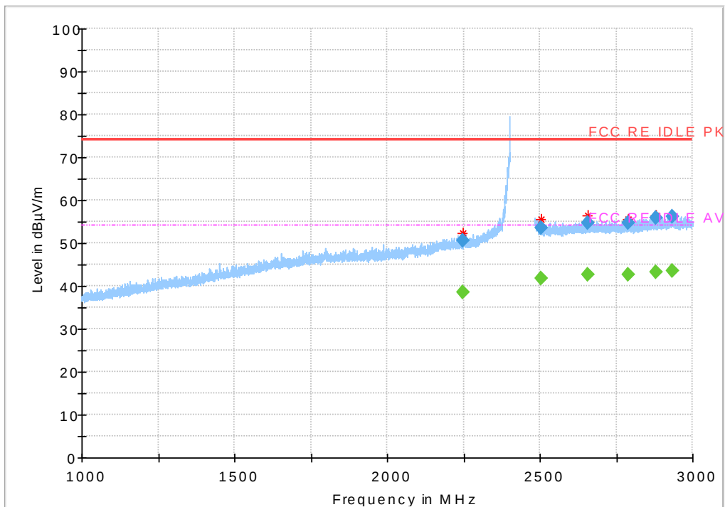
Fig.65 Radiated Spurious Emission (802.11g,Ch1,1GHz~3GHz)
