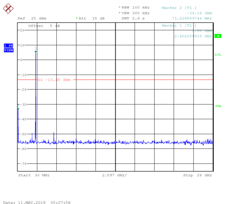
Fig.34 Conducted Spurious Emission (802.11b, Ch1, 30MHz~26GHz)
