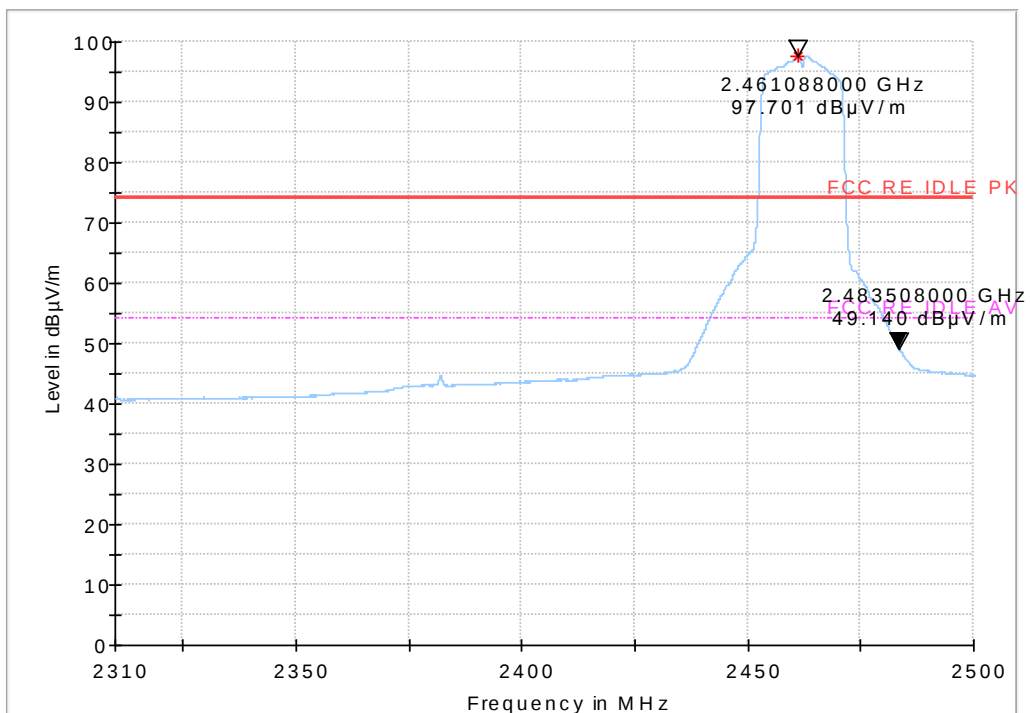
Fig.68 Radiated emission (Power): 802.11n, high channel
