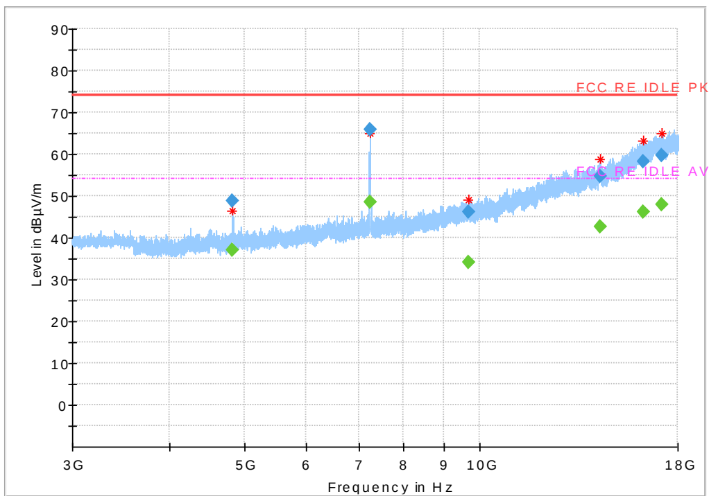
Fig.66 Radiated Spurious Emission (802.11g,Ch1,3GHz~18GHz)
