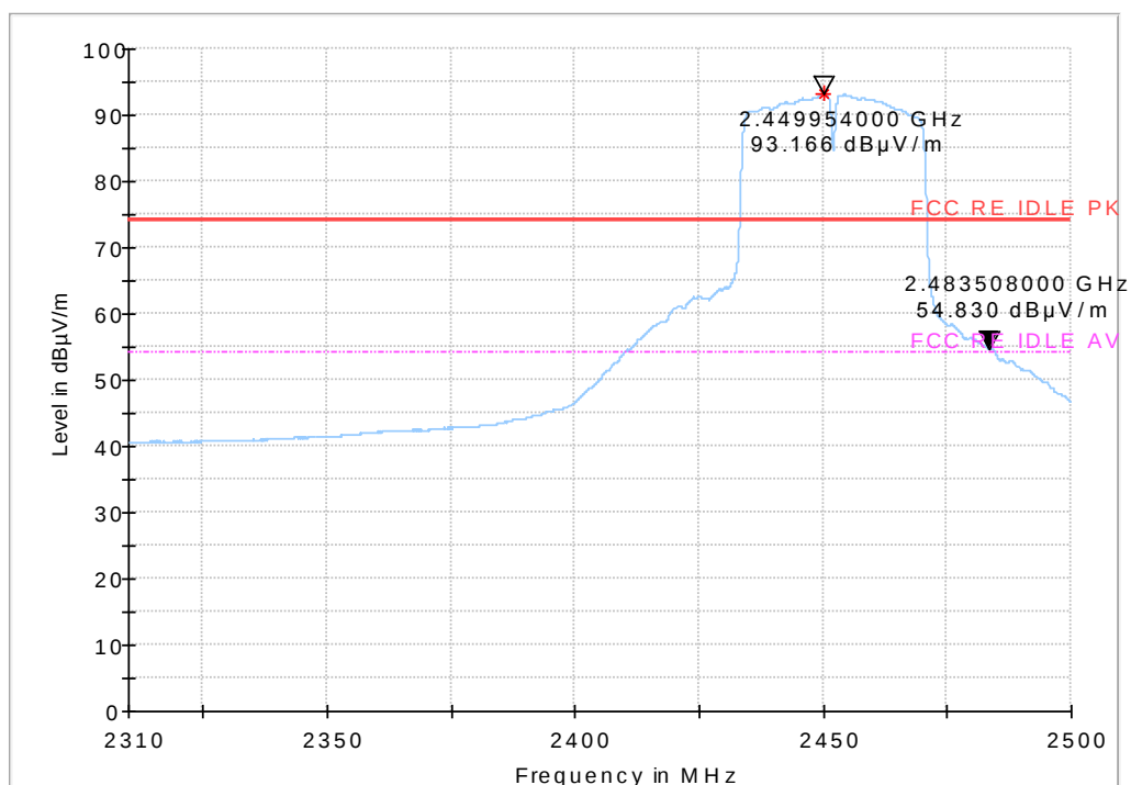
Fig.73 Radiated emission (Power): 802.11n (40M) , high channel
