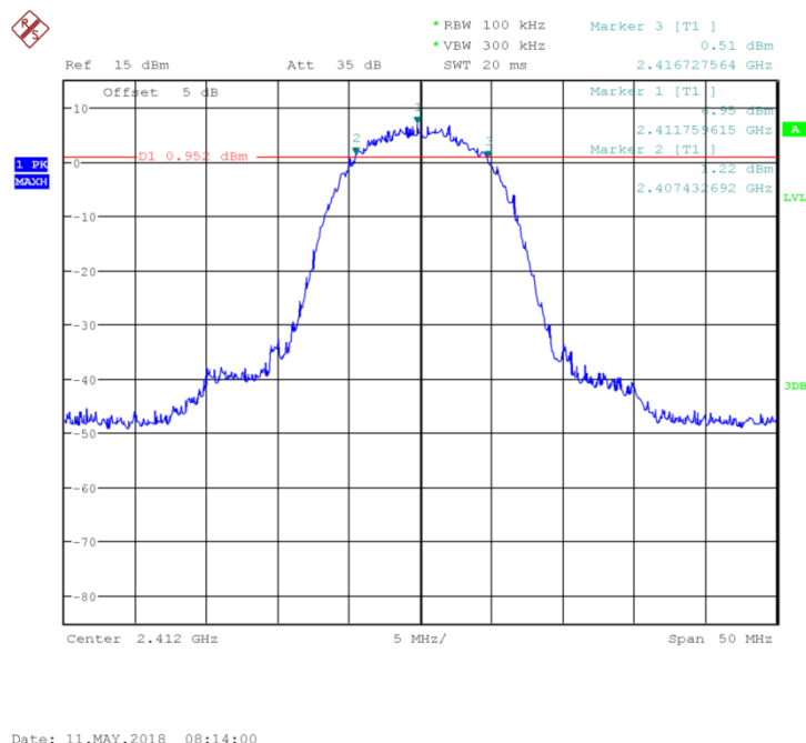
Fig.13 Occupied 6dB Bandwidth (802.11b, Ch1)
