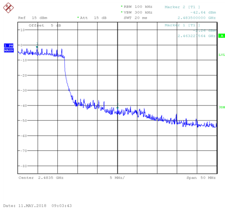
Fig.32 Band Edges (802.11b-40MHz, Ch9)
