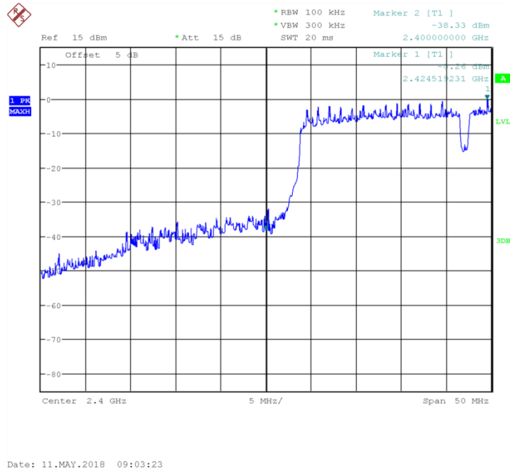
Fig.31 Band Edges (802.11n-40MHz, Ch3)
