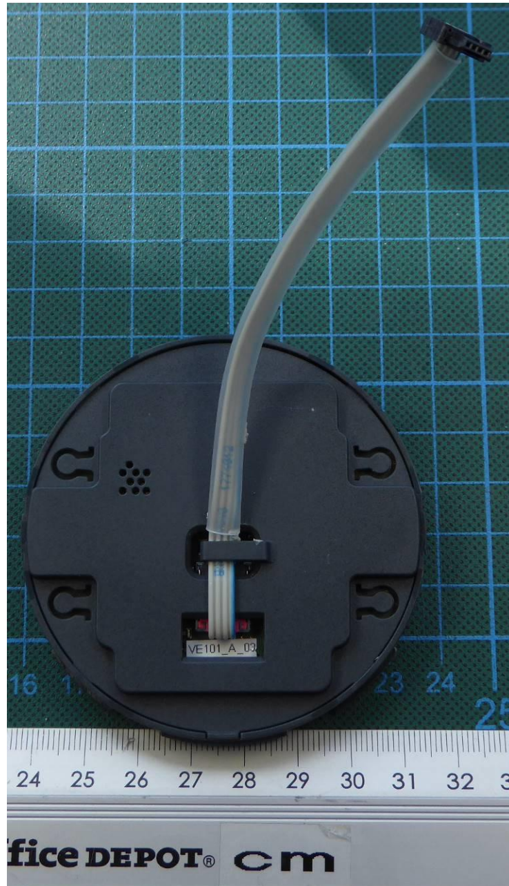
EUT VE101_A_03 – bottom view
