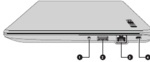
Figure 3-3 The right side of the computer (CL10-B/L10-B)
