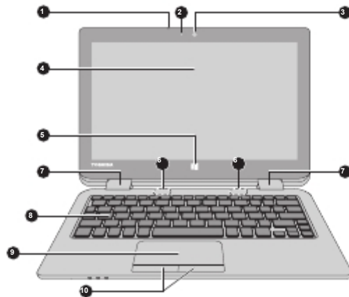
Figure 3-13 The front of the computer with the display panel open (L10W-B)
