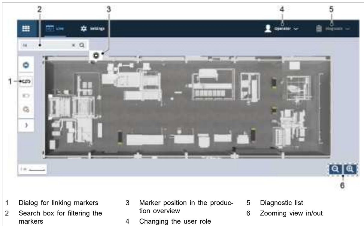
User interface
