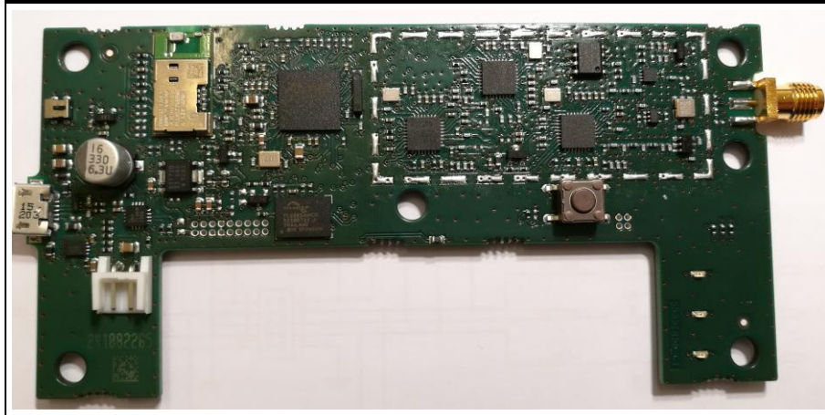
PCB without shielding
