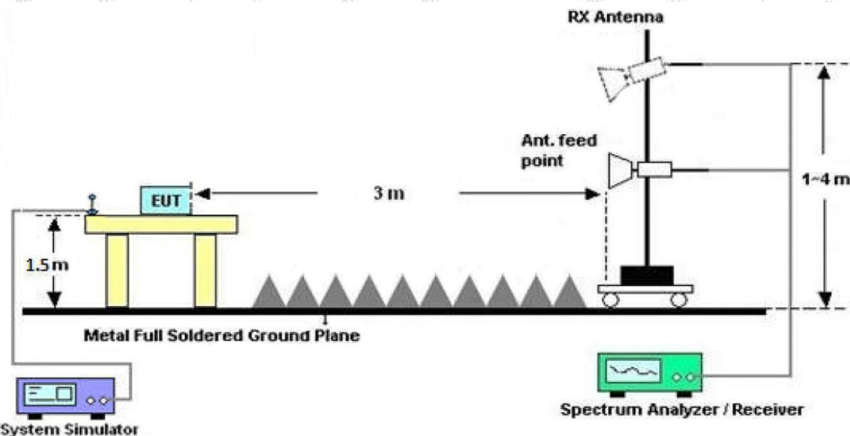
Figure 3. Above 1 GHz
