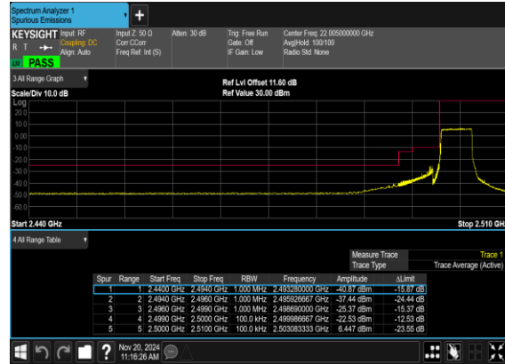
N7(5M)_CP- OFDM_QPSK_Outer_Full_Low_CH
