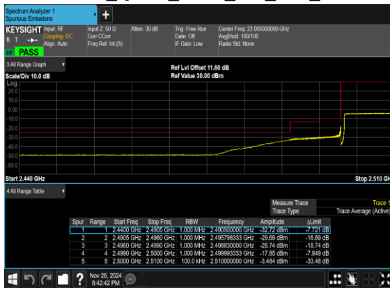
N7(50M)_CP- OFDM_QPSK_Outer_Full_Low_CH
