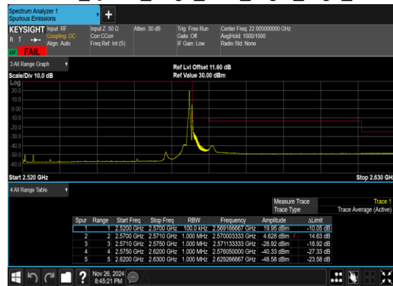
N7(50M)_CP- OFDM_QPSK_Edge_1RB_Right_High_CH
