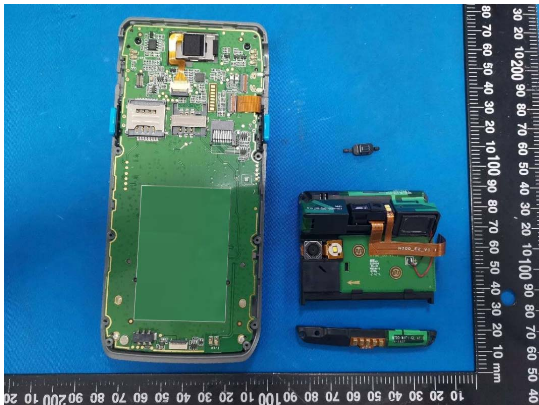
WiFi/BLE Antenna
