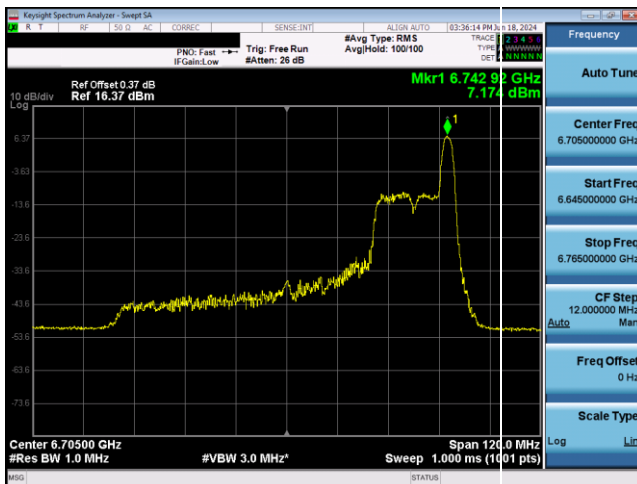
Plot 7-437. SP Power Spectral Density Plot Antenna 3b (80MHz 802.11ax RU26 (UNII Band 7) – Ch. 151)
