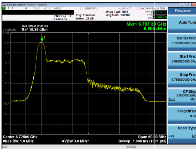
Plot 7-463. SP Power Spectral Density Plot Antenna 1b (40MHz 802.11ax RU26 (UNII Band 7) - Ch. 155)
