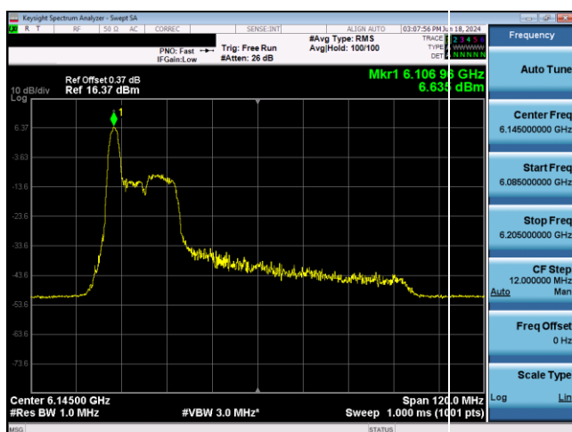
Plot 7-419. SP Power Spectral Density Plot Antenna 3b (80MHz 802.11ax RU26 (UNII Band 5) – Ch. 39)
