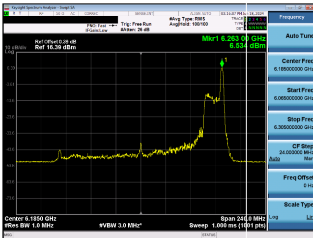
Plot 7-425. SP Power Spectral Density Plot Antenna 3b (160MHz 802.11ax RU26 (UNII Band 5) – Ch. 47)
