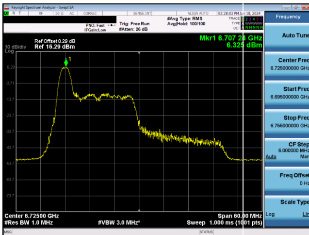
Plot 7-431. SP Power Spectral Density Plot Antenna 3b (40MHz 802.11ax RU26 (UNII Band 7) - Ch. 155)
