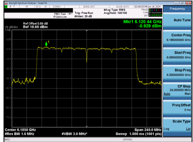
Plot 7-426. SP Power Spectral Density Plot Antenna 3b (160MHz 802.11ax RU996x2 (UNII Band 5) – Ch. 47)
