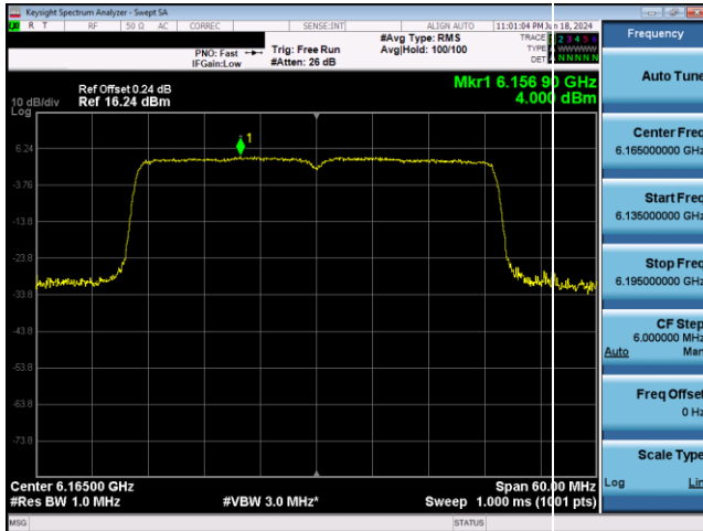
Plot 7-450. SP Power Spectral Density Plot Antenna 1b (40MHz 802.11ax RU484 (UNII Band 5) – Ch. 43)
