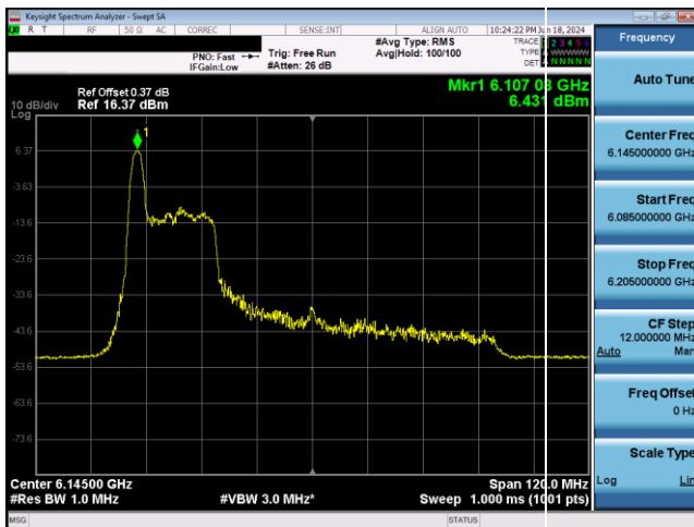
Plot 7-451. SP Power Spectral Density Plot Antenna 1b (80MHz 802.11ax RU26 (UNII Band 5) – Ch. 39)
