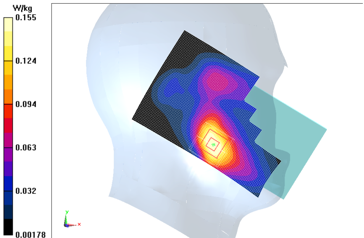
Fig.3 1900 MHz CH512
