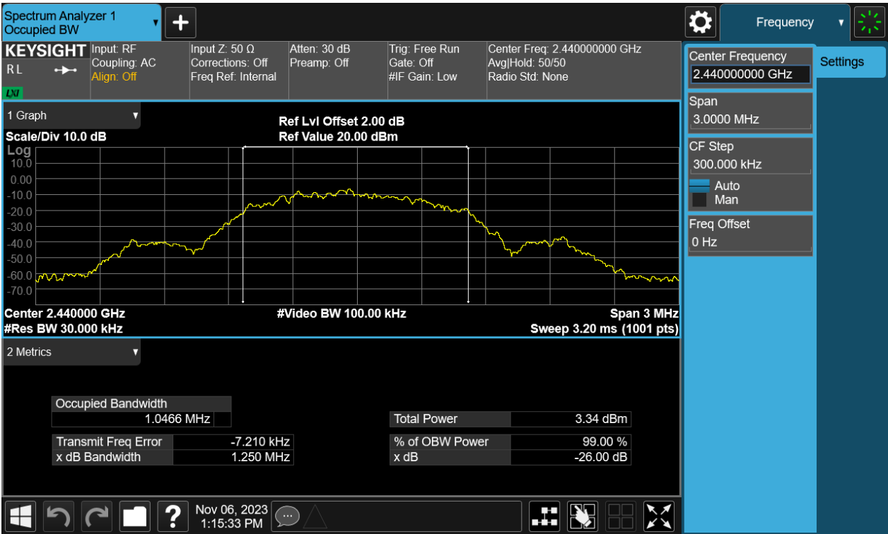
99% Bandwidth, 2440MHz
