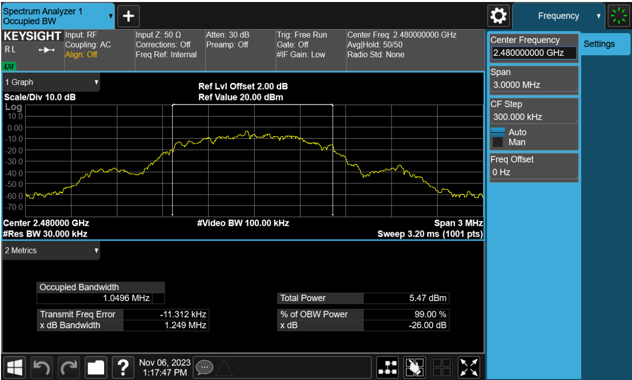
99% Bandwidth, 2480MHz
