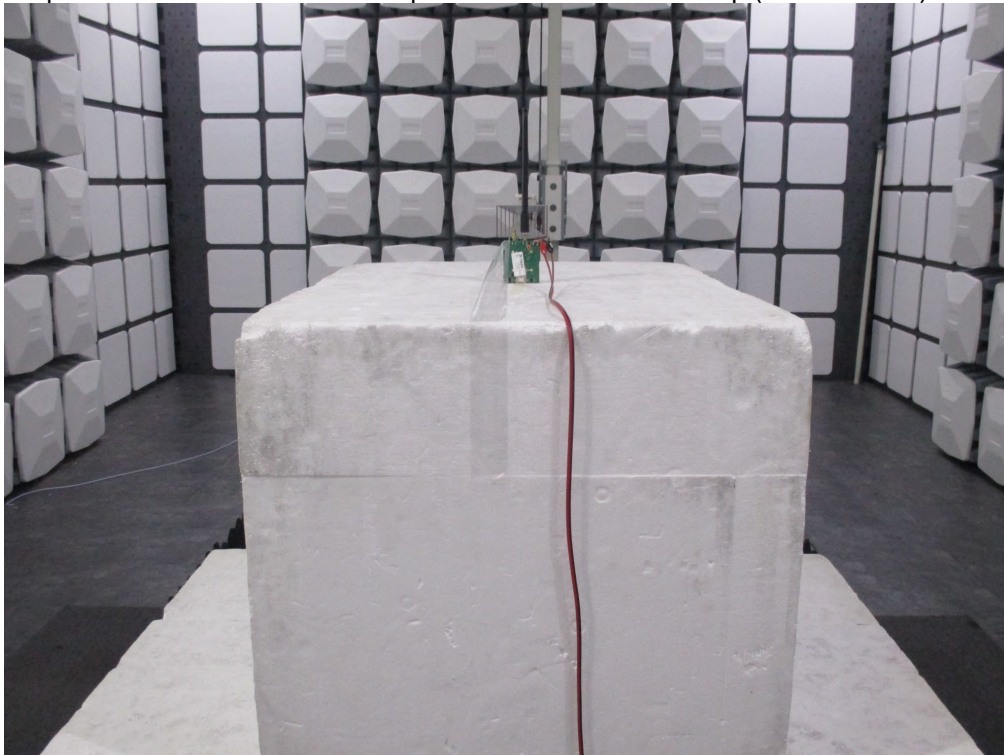
Description: Rear View of Radiated Spurious Emission Test Setup (above 1 GHz)
