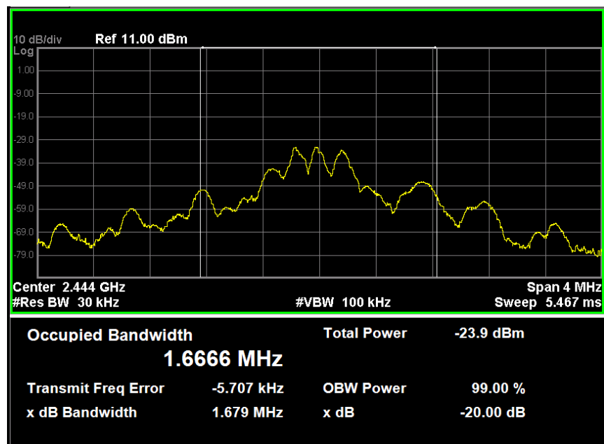
Mid Channel – Bandwidth 1.679 MHz
