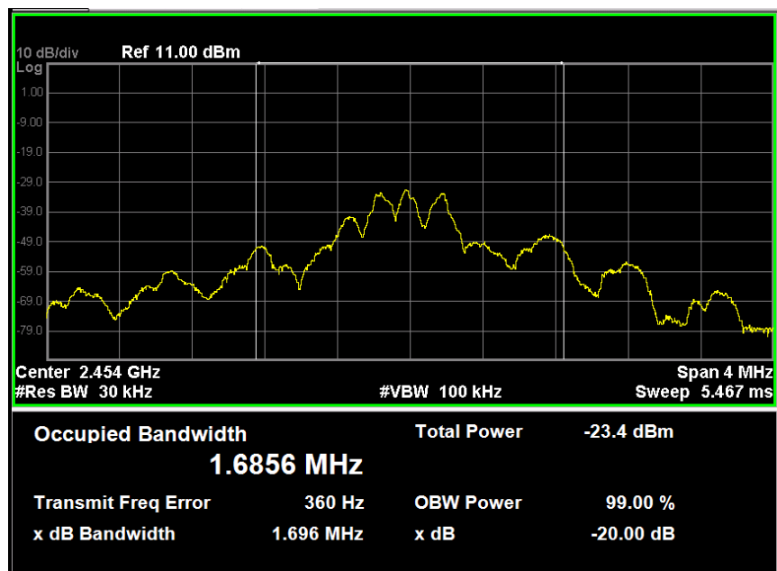
Last Channel – Bandwidth 1.696 MHz
