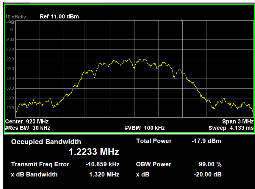
Low Channel – Bandwidth 1.320 MHz
