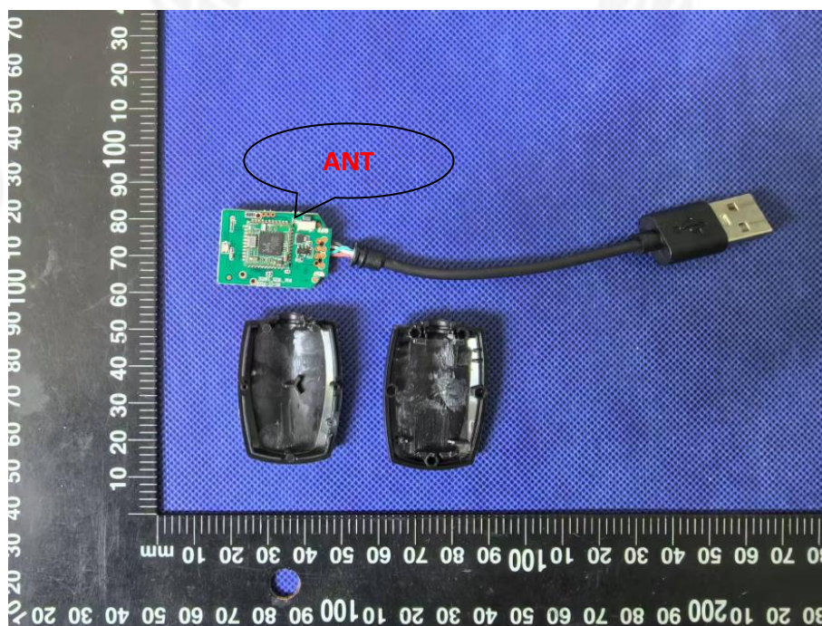
PCB view
