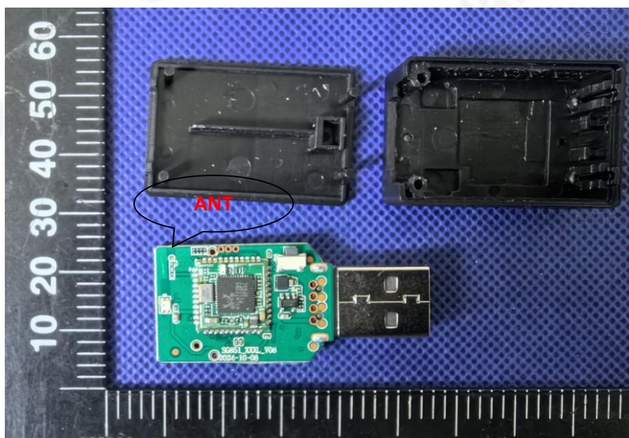
PCB view
