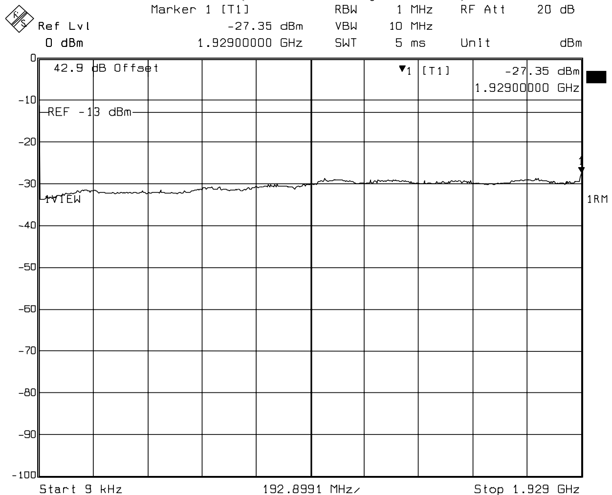
Figure 44 : Conducted Spurious Emissions - 3 Carrier, Channels 325, 350, 375, IS-856, 16-QAM Mode (9kHz -:- Lower Adjacent 1 MHz)
