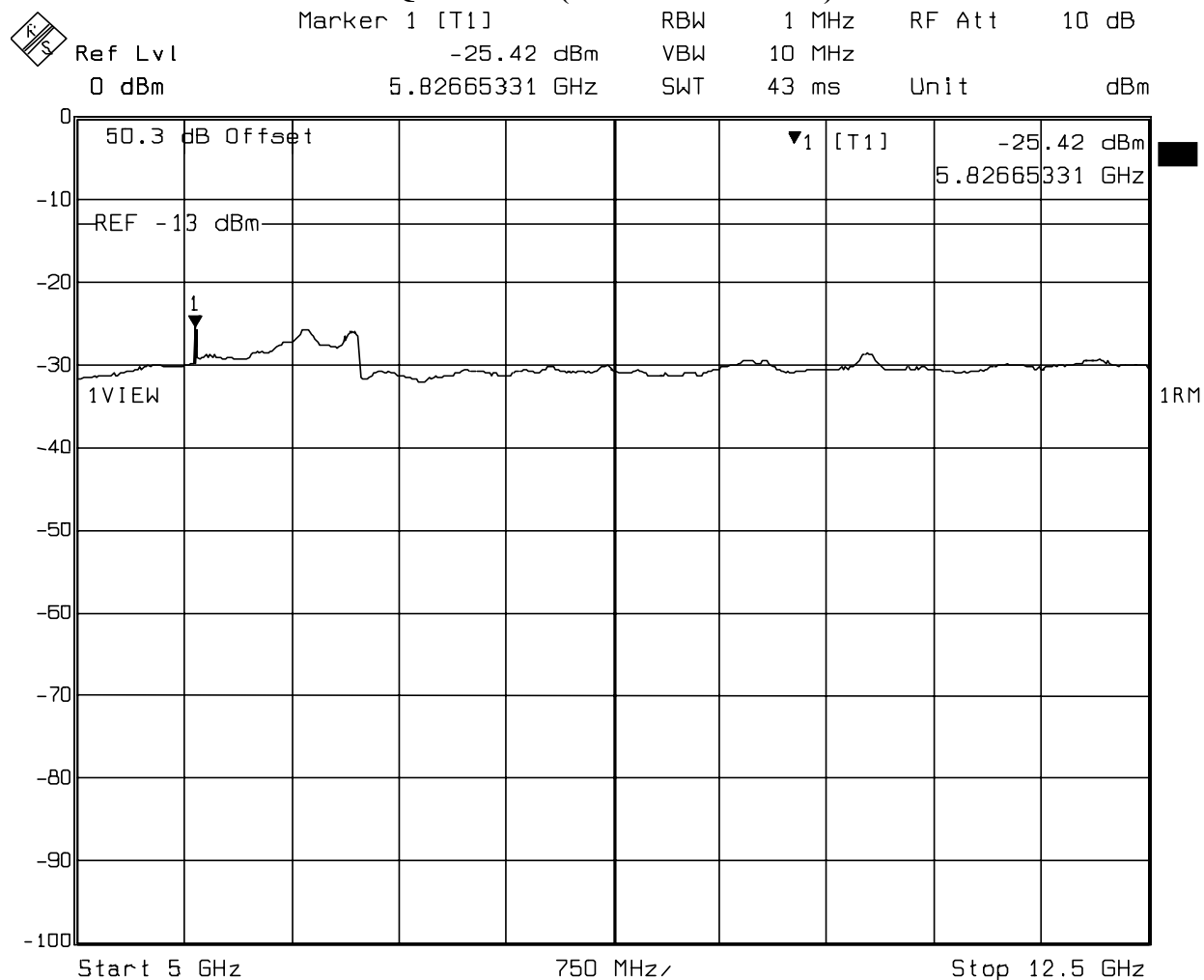
Figure 48 : Conducted Spurious Emissions - 3 Carrier, Channels 325, 350, 375, IS-856, 16-QAM Mode (5 GHz :- 12.5 GHz)
