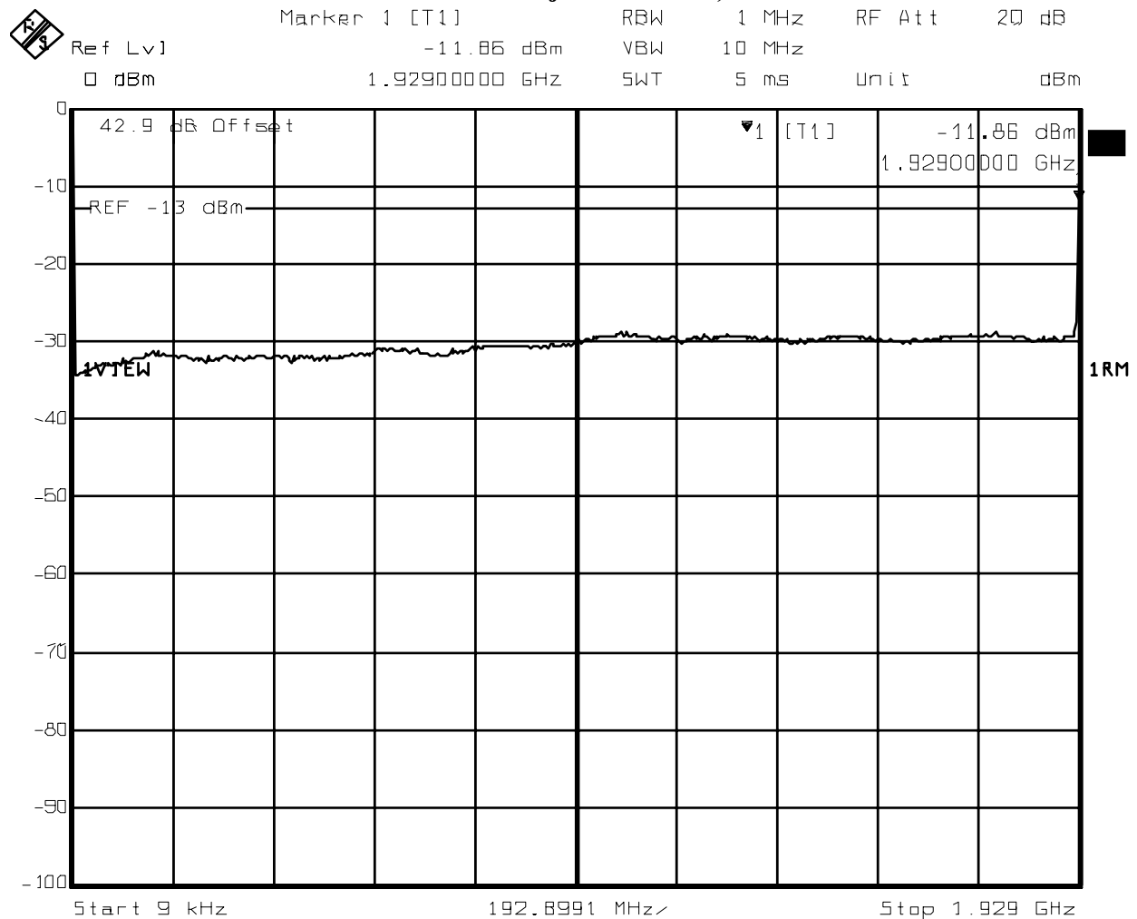
Figure 28 : Conducted Spurious Emissions - 2 Carrier, Channels 25, 50, IS-95 (9kHz -:- Lower Adjacent 1 MHz)
