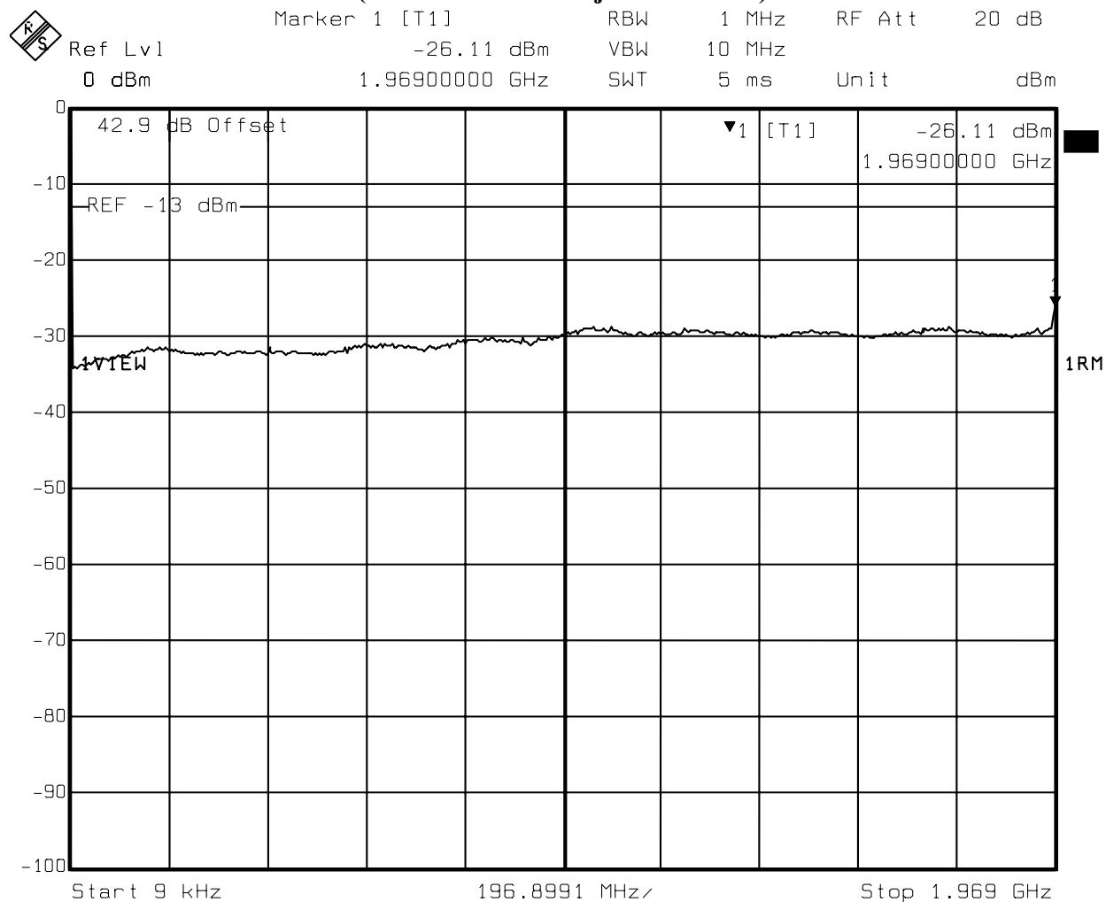
Figure 36 : Conducted Spurious Emissions - 3 Carrier, Channels 1125, 1150, 1175, IS-95 (9kHz :- Lower Adjacent 1 MHz)
