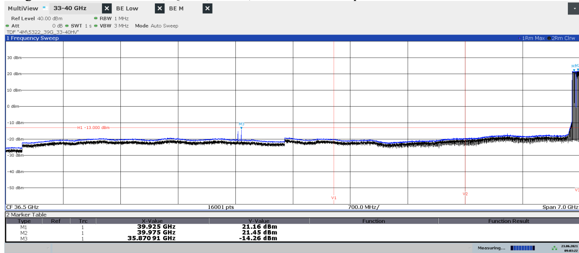
Diagram 2.5a: 33 – 40 GHz, QPSK, TH 250 , EIRP Horizontal polarization
