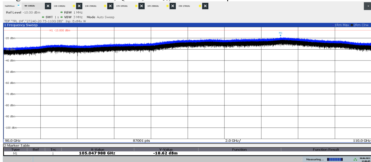
Diagram 2.16b: 90 – 110 GHz, QPSK, BL 250 , EIRP Vertical polarization
