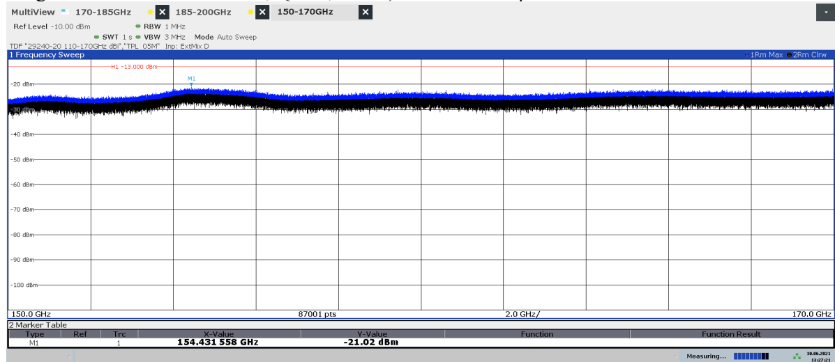
Diagram 2.19b: 150 – 170 GHz, QPSK, BL2 50 , EIRP Vertical polarization
