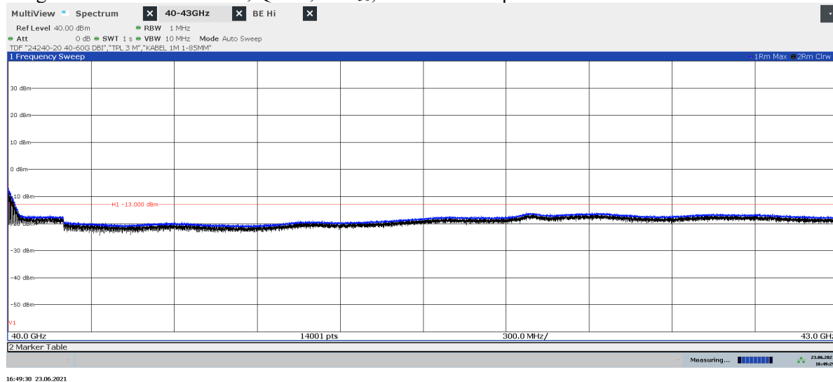
Diagram 2.10b: 40 – 43 GHz, QPSK, TH2 50 , EIRP Vertical polarization
