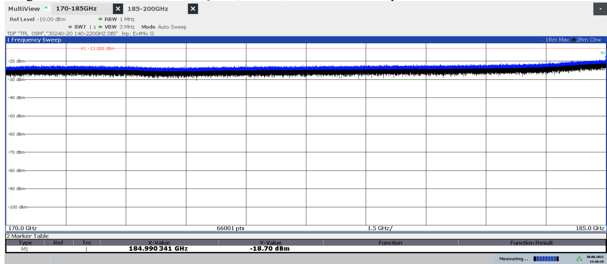
Diagram 2.20a: 170 – 185 GHz, QPSK, BL 250 , EIRP Horizontal polarization
