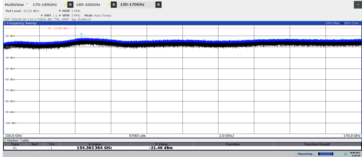
Diagram 2.19a: 150 – 170 GHz, QPSK, BL2 50 , EIRP Horizontal polarization
