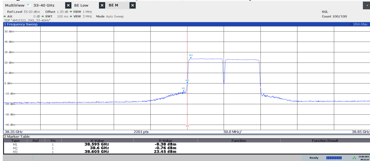
Diagram 2.9a: 38.35 – 38.85 GHz, QPSK, BH2 50 , EIRP Horizontal polarization
