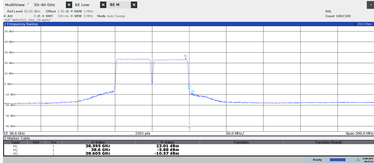
Diagram 2.8a: 38.35 – 38.85 GHz, QPSK, TL2 50 , EIRP Horizontal polarization
