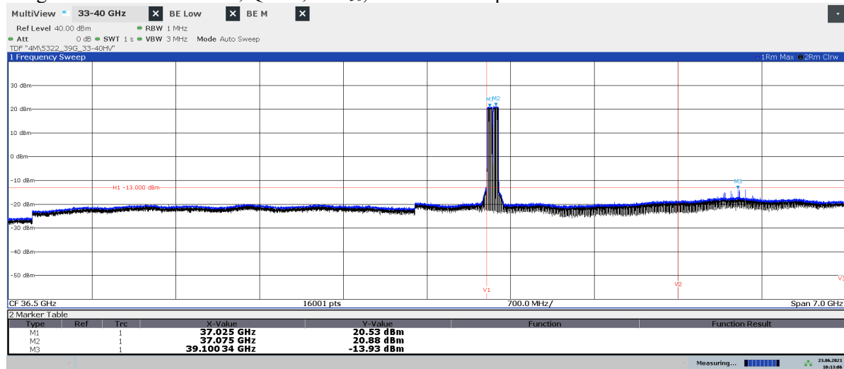
Diagram 2.6b: 33 – 40 GHz, QPSK, BL 250 , EIRP Vertical polarization
