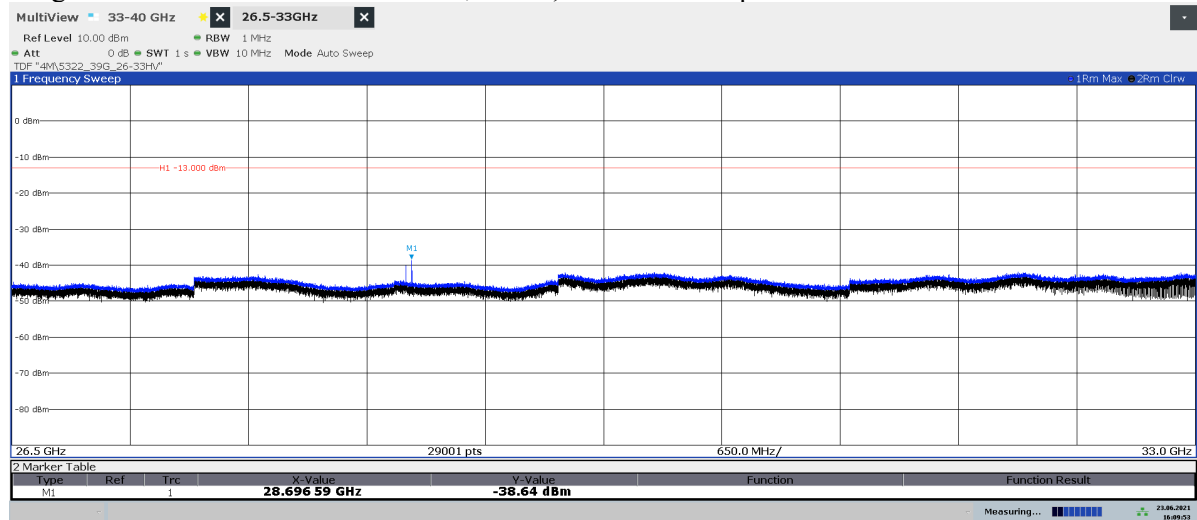
Diagram 2.4b: Pre scan 26.5 – 33 GHz, TH 250 , EIRP Vertical polarization
