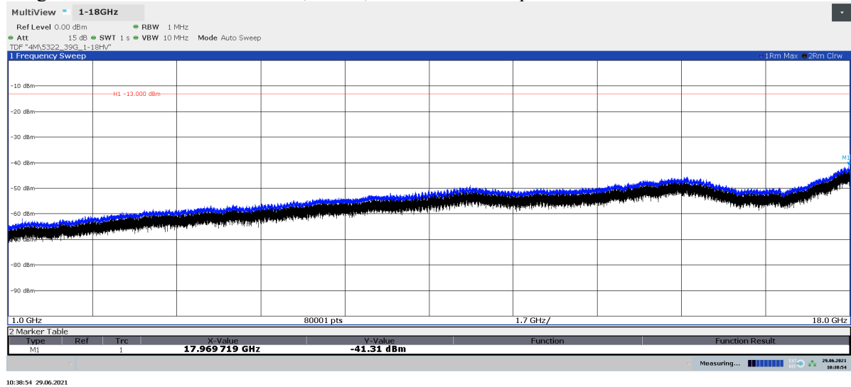
Diagram 2.2a: Pre scan 1 – 18 GHz, BL2 50 , EIRP Horizontal polarization
