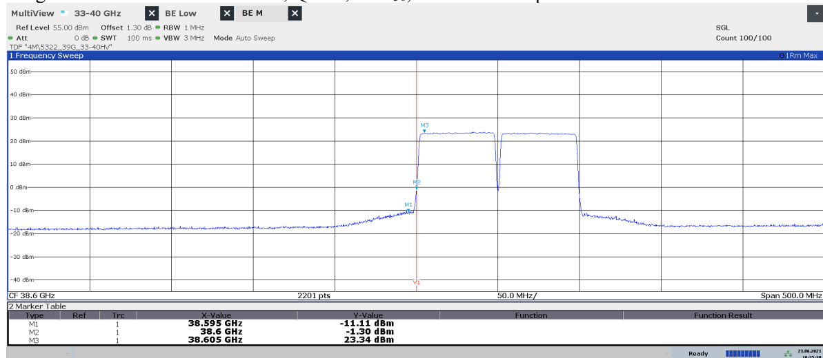
Diagram 2.9b: 38.35 – 38.85 GHz, QPSK, BH2 50 , EIRP Vertical polarization
