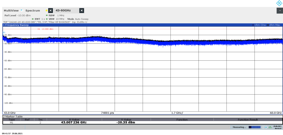
Diagram 2.13a: 43 – 60 GHz, QPSK, BL 250 , EIRP Horizontal polarization
