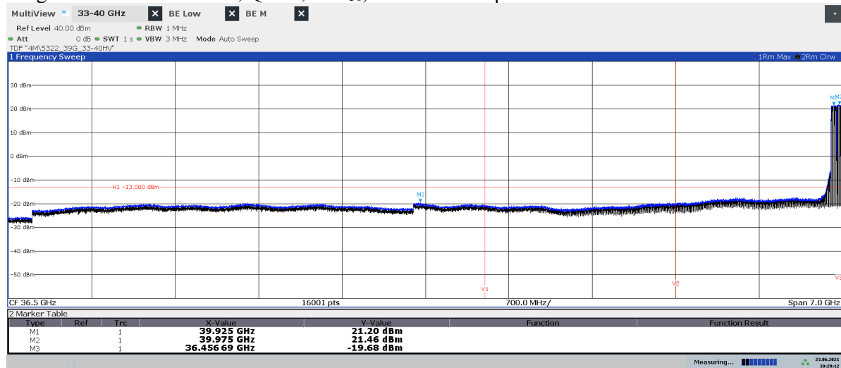
Diagram 2.5b: 33 – 40 GHz, QPSK, TH 250 , EIRP Vertical polarization
