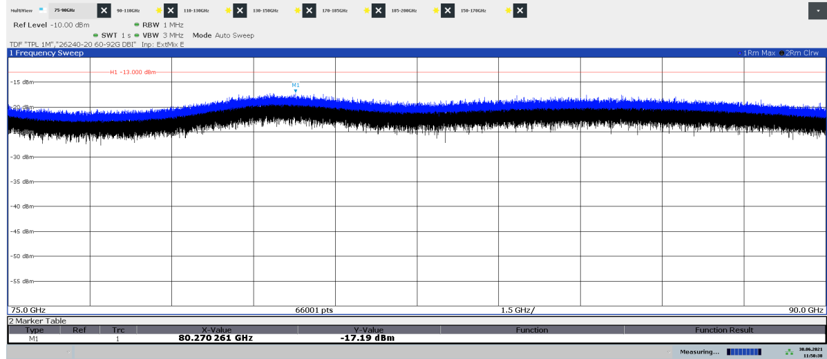
Diagram 2.15a: 75 – 90 GHz, QPSK, BL2 50 , EIRP Horizontal polarization
