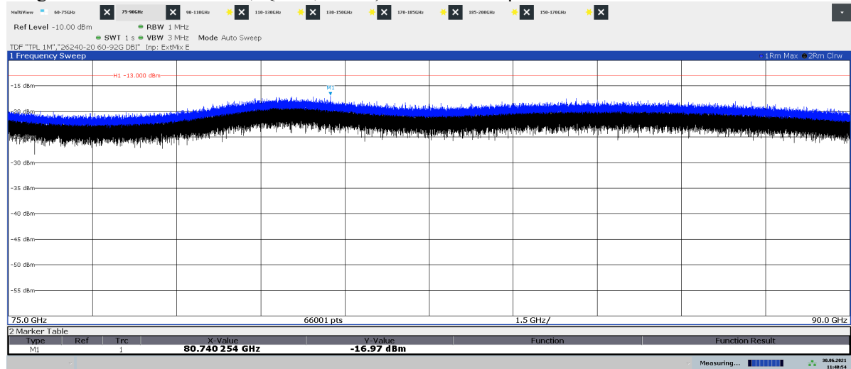
Diagram 2.15b: 75 – 90 GHz, QPSK, BL2 50 , EIRP Vertical polarization
