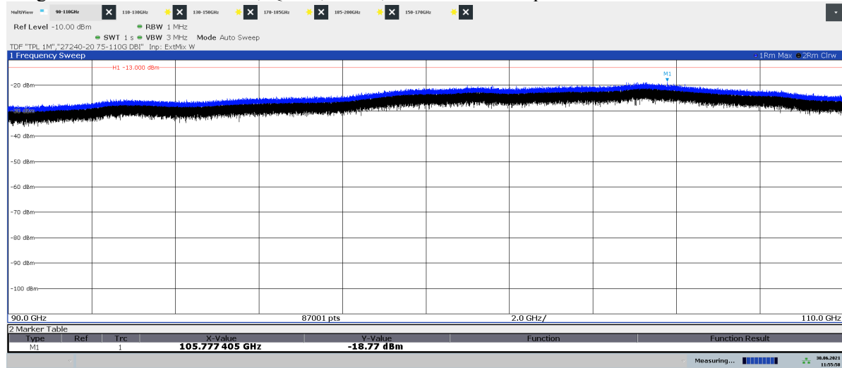
Diagram 2.16a: 90 – 110 GHz, QPSK, BL 250 , EIRP Horizontal polarization
