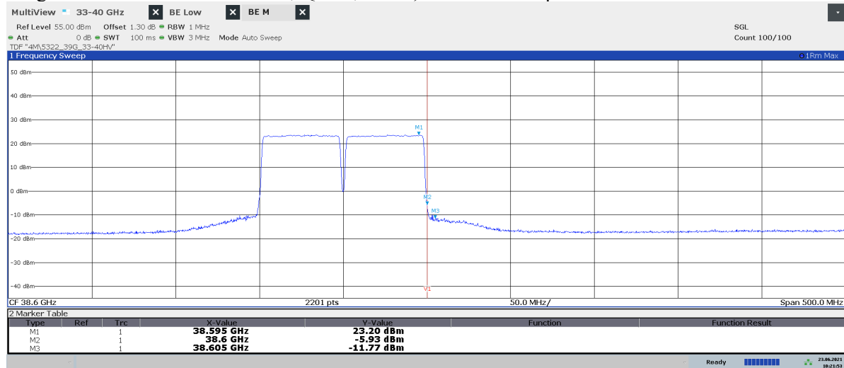
Diagram 2.8b: 38.35 – 38.85 GHz, QPSK, TL2 50 , EIRP Vertical polarization
