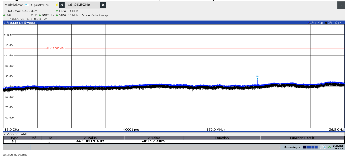
Diagram 2.3b: Pre scan 18 – 26.5 GHz, BL 250 , EIRP Vertical polarization
