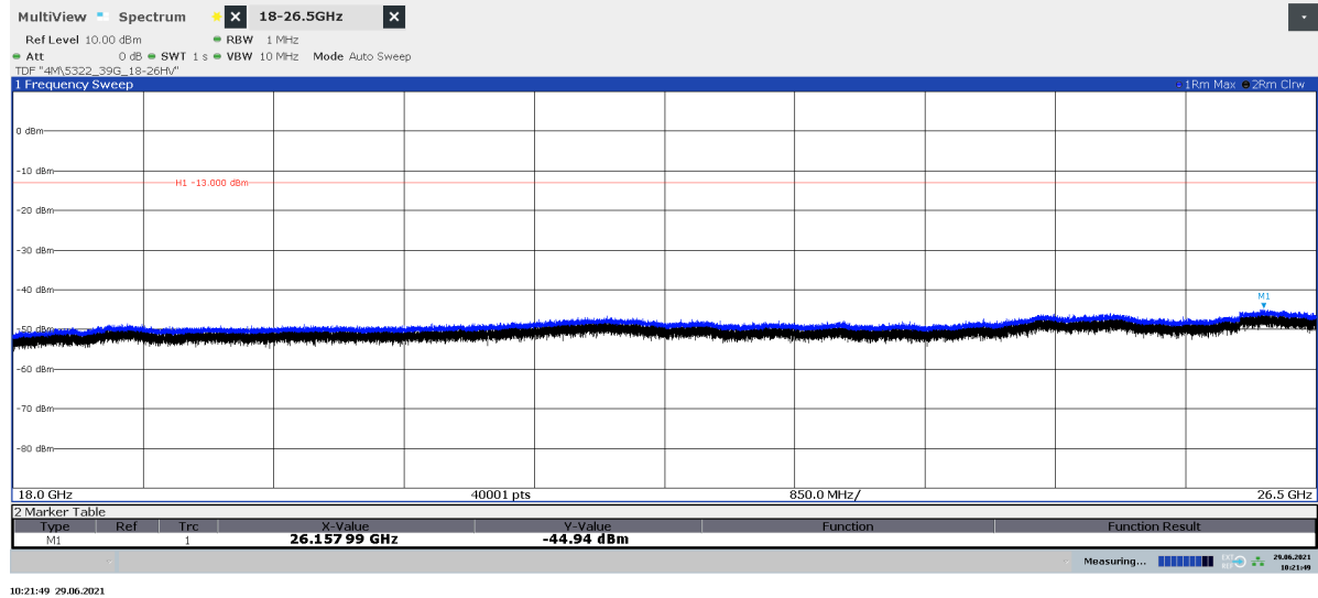
Diagram 2.3a: Pre scan 18 – 26.5 GHz, BL 250 , EIRP Horizontal polarization
