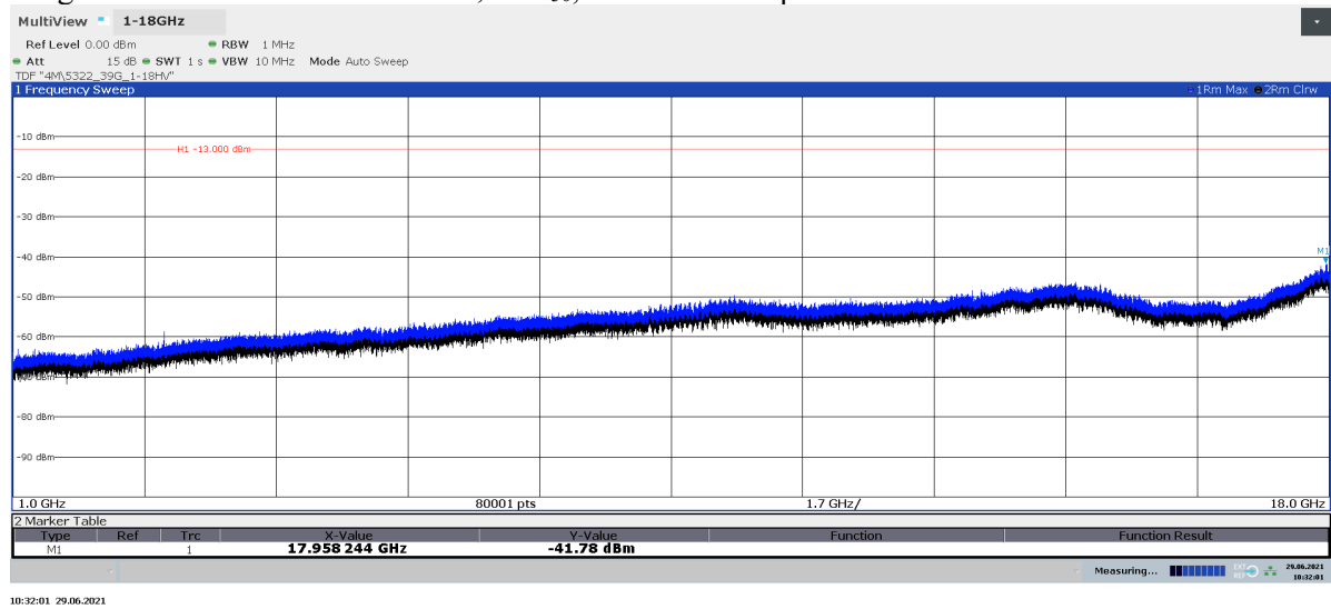
Diagram 2.2b: Pre scan 1 – 18 GHz, BL2 50 , EIRP Vertical polarization
