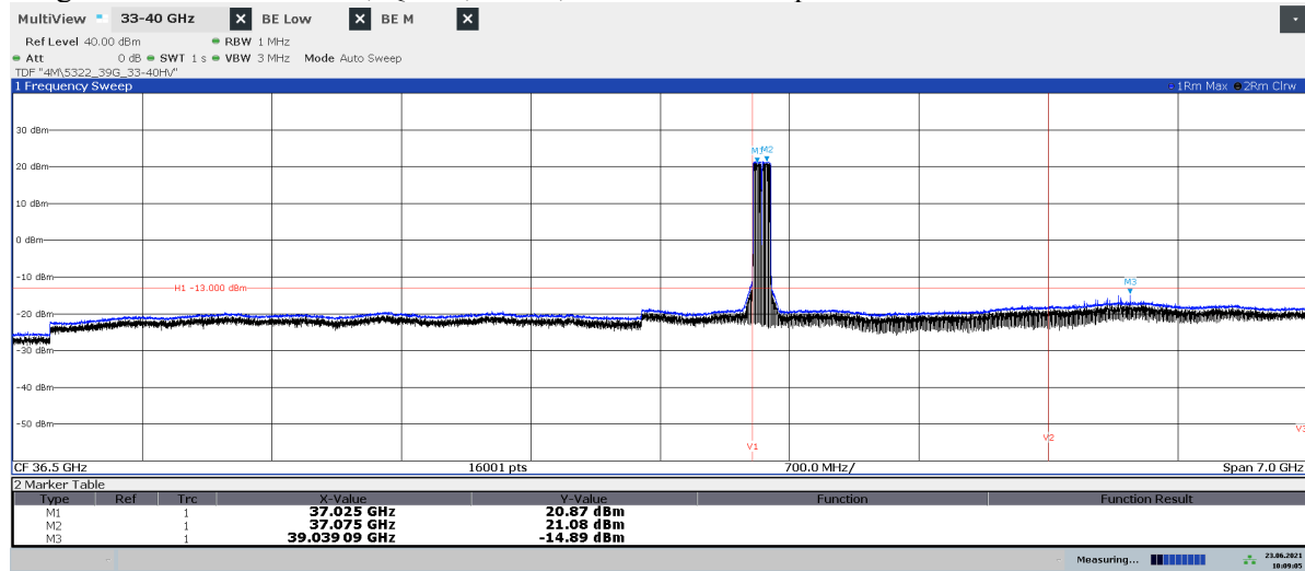
Diagram 2.6a: 33 – 40 GHz, QPSK, BL 250 , EIRP Horizontal polarization
