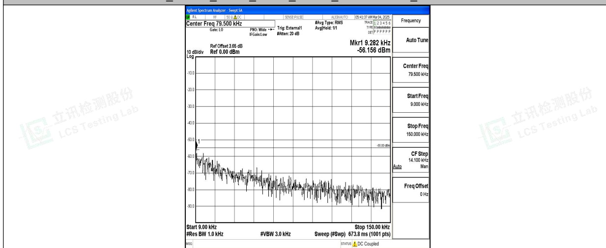
Band38 15MHz 16QAM 37825 1RB#0 0.009~0.15 0.009~0.15
