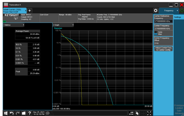
5G NR n77_CH649668_90M_1RB_16-QAM_Ratio
