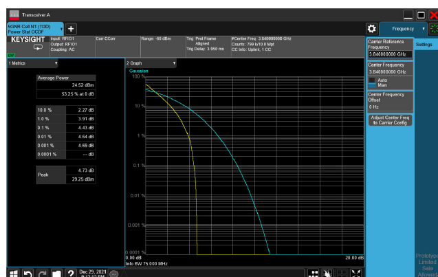
5G NR n77 CH656000 70M 1RB 16-QAM Ratio
