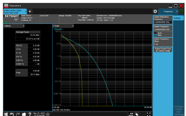
5G NR n77_CH656000_90M_1RB_16-QAM_Ratio
