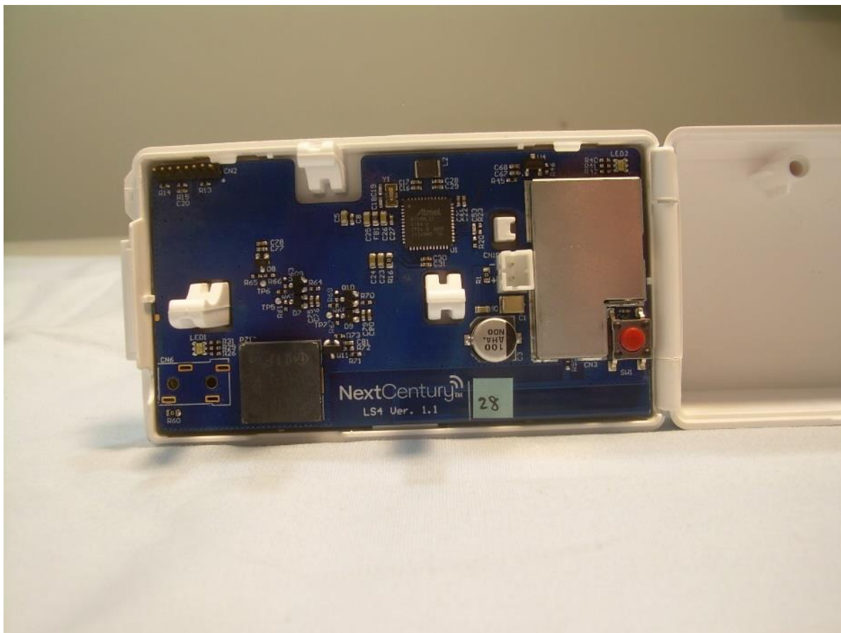
Photograph 4 – View of PCB in Housing
