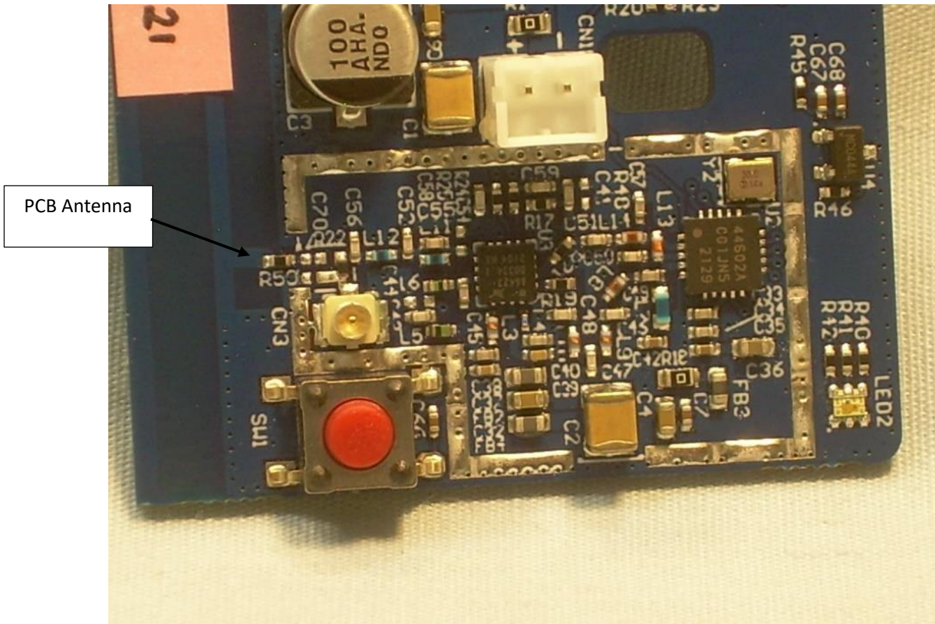
Photograph 3 – View of Circuitry Under the RF Shield
