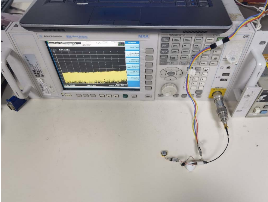
RF Conducted Test setup (BT/BLE)
