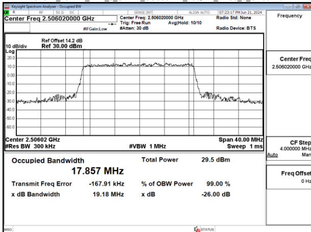
Band41_20MHz_DFT_s_OFDM_SCS30kHz_16QAM_RB50_0_CH501204
