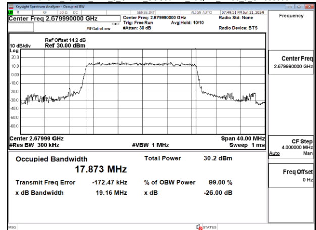
Band41_20MHz_DFT_s_OFDM_SCS30kHz_16QAM_RB50_0_CH535998
