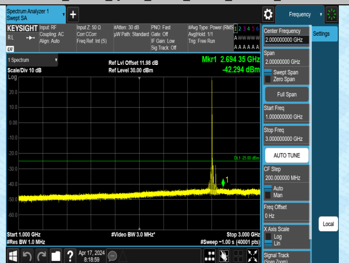
Band38_20MHz_QPSK_38150_1RB#0_1000~3000_1000~3000
