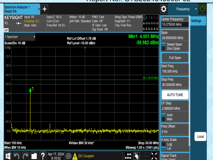
Band38_20MHz_QPSK_38150_1RB#0_0.15~30_0.15~30
