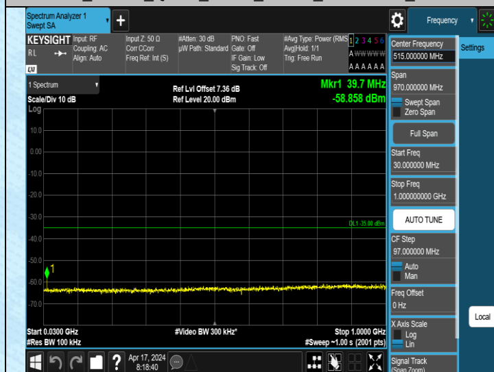
Band38_20MHz_QPSK_38150_1RB#0_30~1000_30~1000
