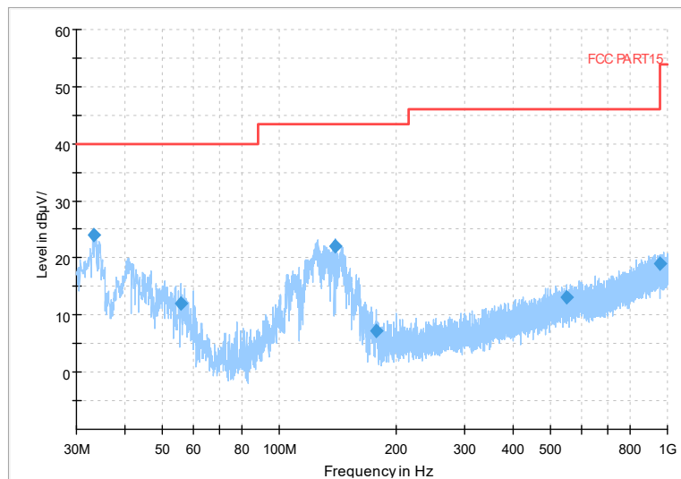
Frequency Range: 30MHz-1000 MHz Detector: QP mode
