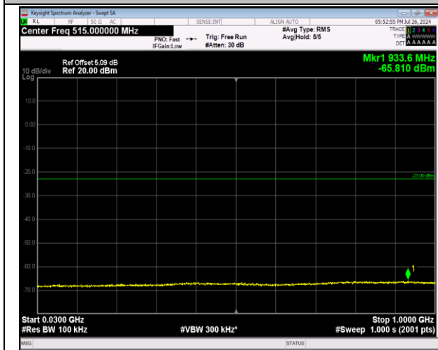
2-2-5MHz-20MHz-64QAM-64QAM-18808-18925-1RB#0- 0RB#0-30~1000MHz-PASS
