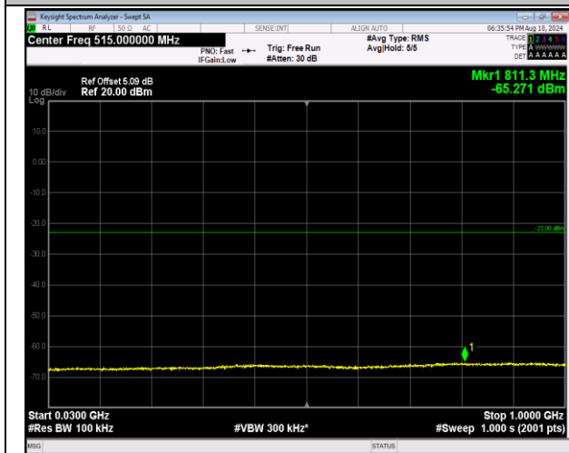
2-2-5MHz-20MHz-16QAM-16QAM-18808-18925-1RB#24-0RB#0-30~1000MHz-PASS
