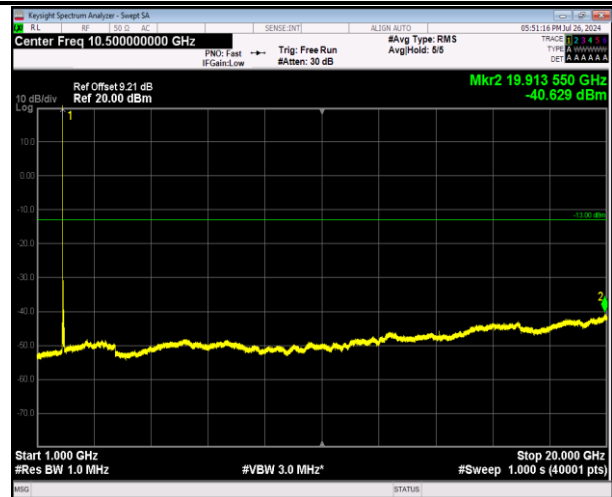
2-2-5MHz-20MHz-64QAM-64QAM-18633-18750-1RB#24-0 RB#0-1000~20000MHz-PASS
