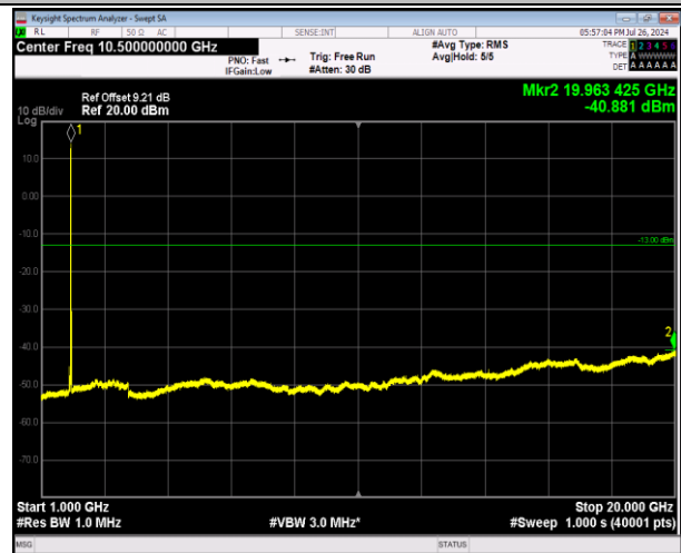
2-2-5MHz-20MHz-64QAM-64QAM-18983-19100-1RB#0-1R B#99-1000~20000MHz-PASS
