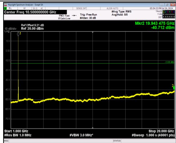
2-2-5MHz-20MHz-64QAM-64QAM-18808-18925-1RB#0-1R B#99-1000~20000MHz-PASS
