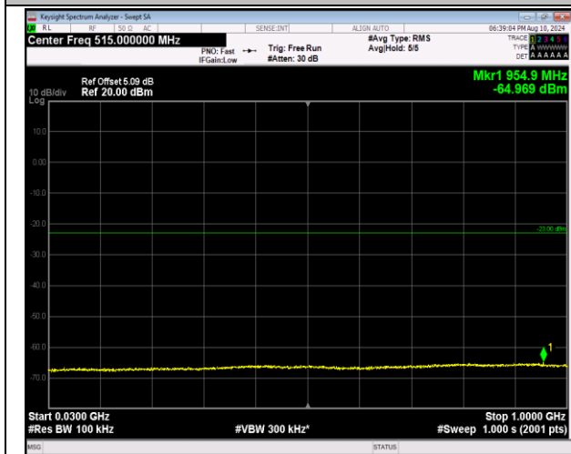
2-2-5MHz-20MHz-QPSK-QPSK-18983-19100-1RB#0-0R B#0-30~1000MHz-PASS
