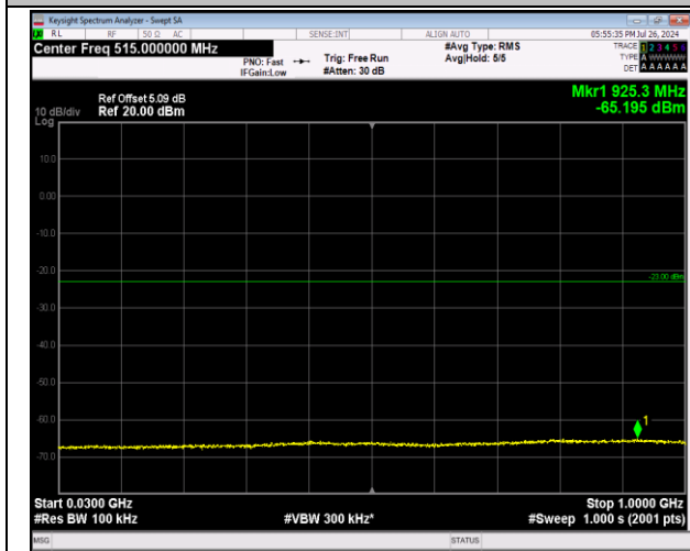
2-2-5MHz-20MHz-64QAM-64QAM-18983-19100-1RB#0- 0RB#0-30~1000MHz-PASS
