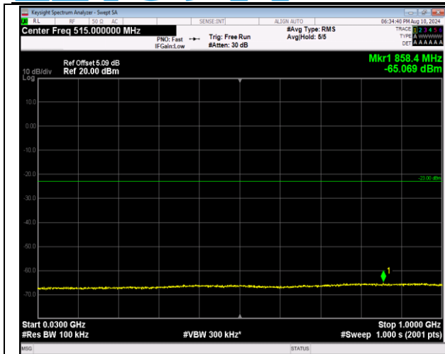
2-2-5MHz-20MHz-16QAM-16QAM-18808-18925-1RB#0-0RB#0-30~1000MHz-PASS
