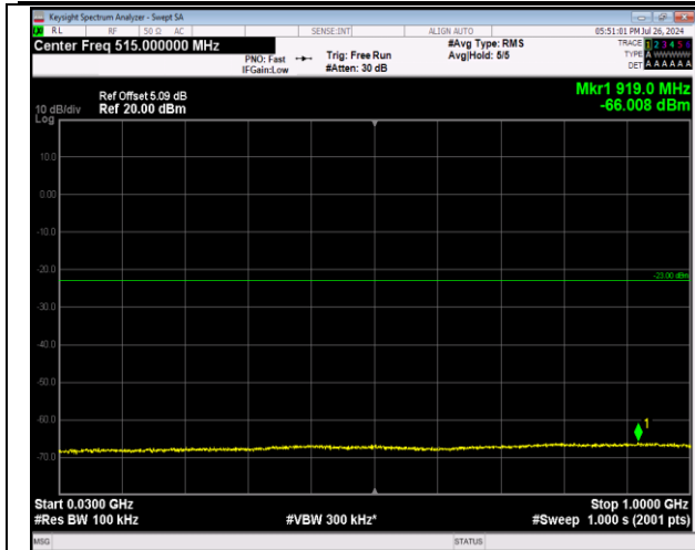
2-2-5MHz-20MHz-64QAM-64QAM-18633-18750-1RB#24 -0RB#0-30~1000MHz-PASS
