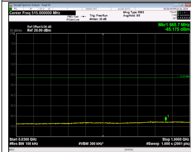
2-2-5MHz-20MHz-64QAM-64QAM-18983-19100-1RB#0- 1RB#99-30~1000MHz-PASS
