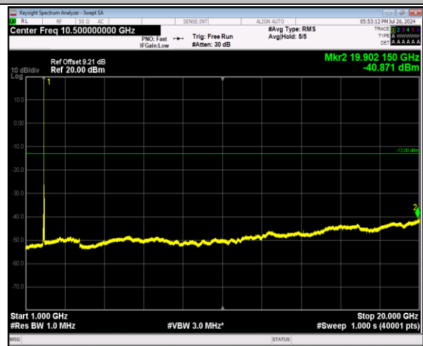
2-2-5MHz-20MHz-64QAM-64QAM-18808-18925-1RB#0-OR B#0-1000~20000MHz-PASS
