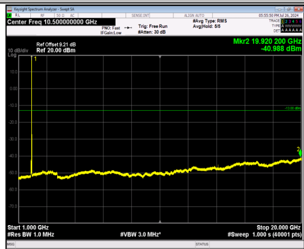
2-2-5MHz-20MHz-64QAM-64QAM-18983-19100-1RB#0-OR B#0-1000~20000MHz-PASS
