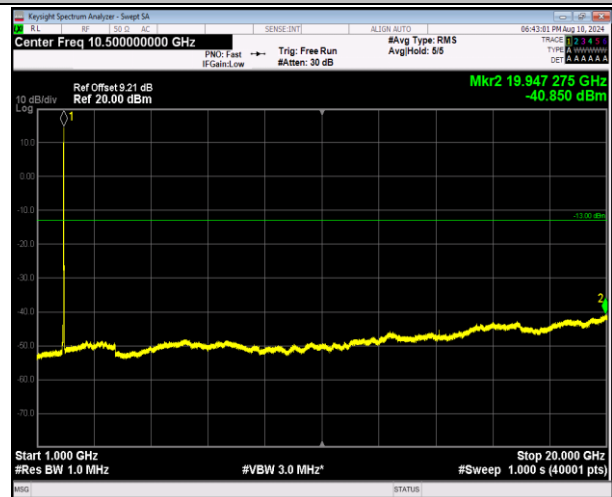
2-2-5MHz-20MHz-QPSK-QPSK-18983-19100-25RB#0-100 RB#0-1000~20000MHz-PASS
