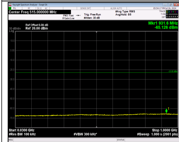
2-2-5MHz-20MHz-64QAM-64QAM-18808-18925-1RB#0- 1RB#99-30~1000MHz-PASS
