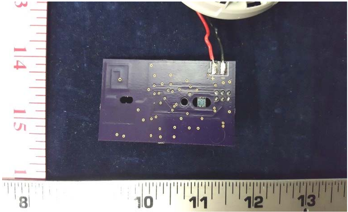
Figure 7.6 Foil Side
