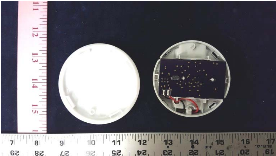
Figure 7.4 Inside View
