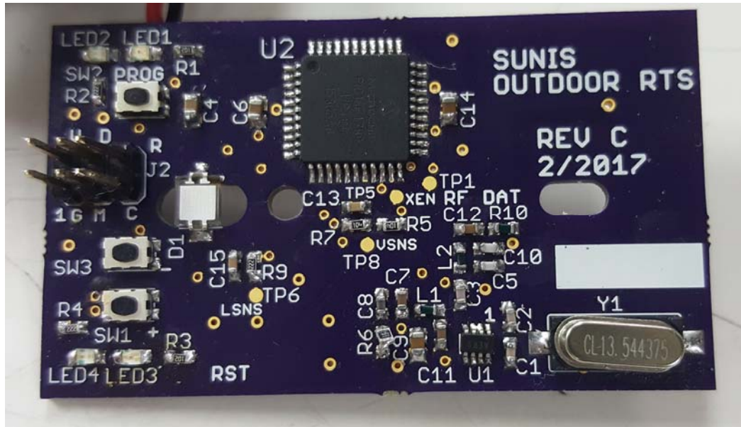
Figure 7.5 Component Side
