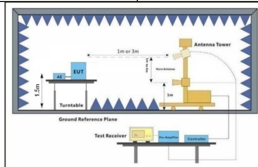
Figure 3. above 1GHz
