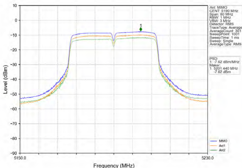
802.11n(HT40)_LCH_5190MHz_MIMO_NTNV
