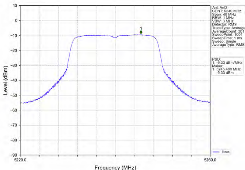
802.11n(HT20)_HCH_5240MHz_Ant2_NTNV
