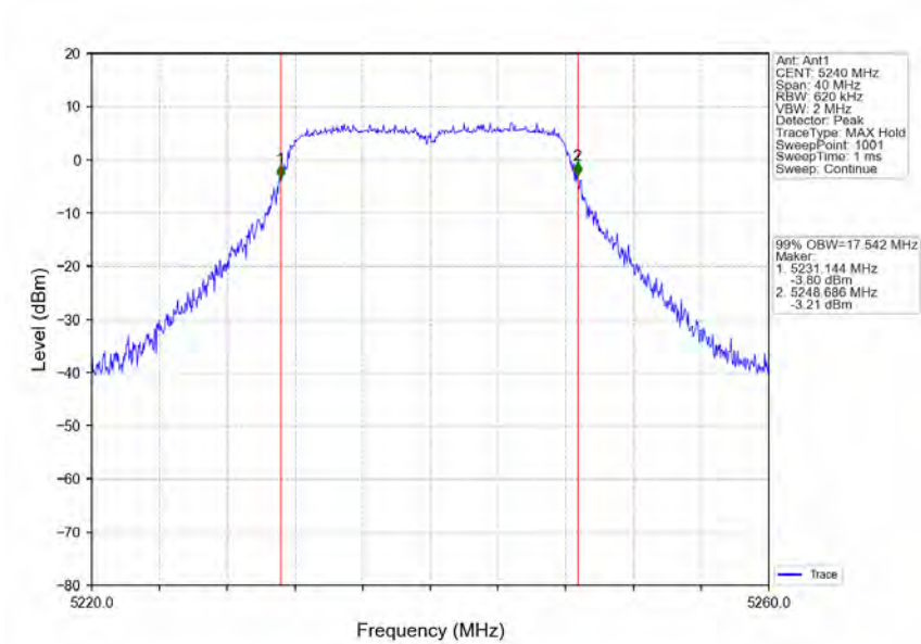
802.11a_HCH_5240MHz_Ant1_NTNV
