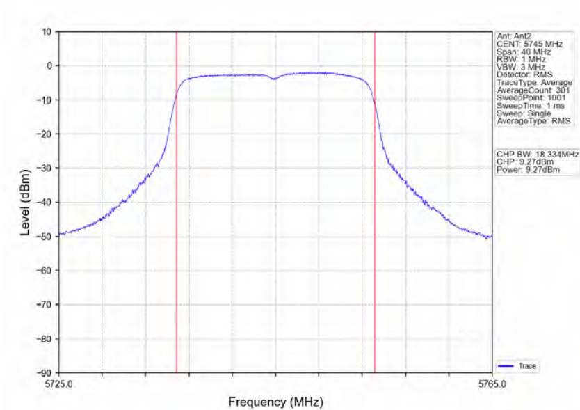
802.11n(HT20)_LCH_5745MHz_Ant2_NTNV
