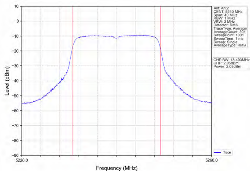
802.11n(HT20)_HCH_5240MHz_Ant2_NTNV
