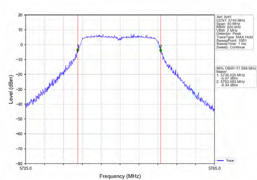
802.11a_LCH_5745MHz_Ant1_NTNV
