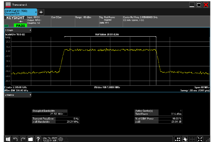
n38_40MHz_30kHz_2595MHz_DFT-s-OFDM \pi/2 BPSK_RB100@0
