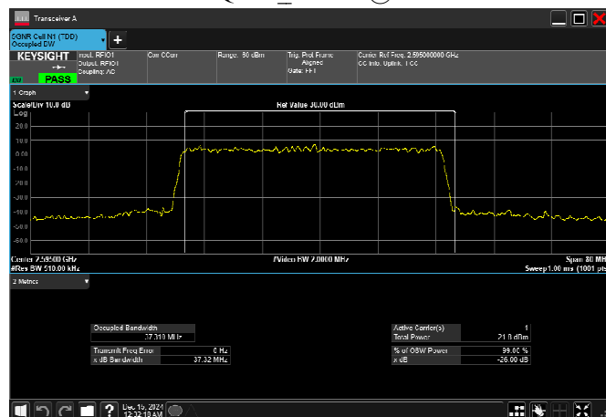
n38_40MHz_30kHz_2595MHz_CP-OFDM 16 QAM RB106@0
