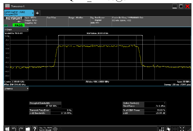
n38_40MHz_30kHz_2595MHz_DFT-s-OFDM 16 QAM_RB100@0
