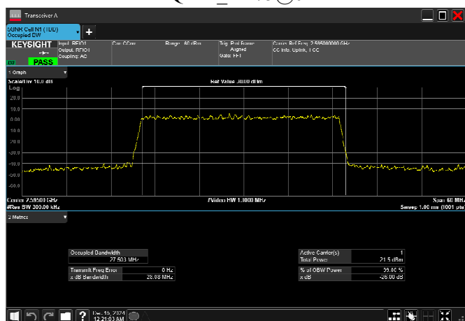
n38_30MHz_30kHz_2595MHz_DFT-s-OFDM 256 QAM_RB75@0
