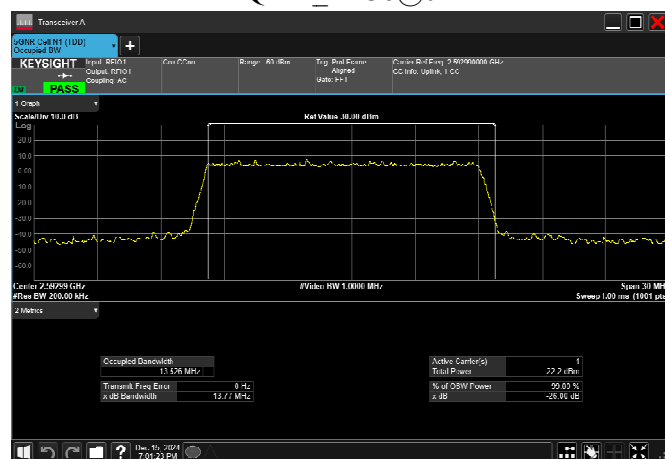
n41_15MHz_30kHz_2592.99MHz_DFT-s-OFDM 16 QAM RB36@0
