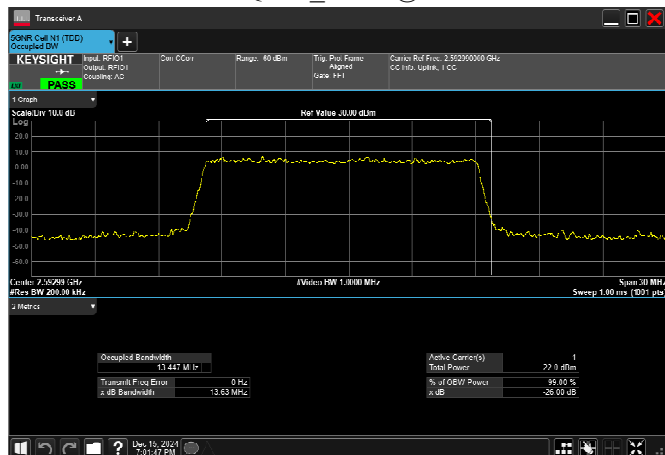
n41_15MHz_30kHz_2592.99MHz_CP-OFDM QPSK_RB38@0
