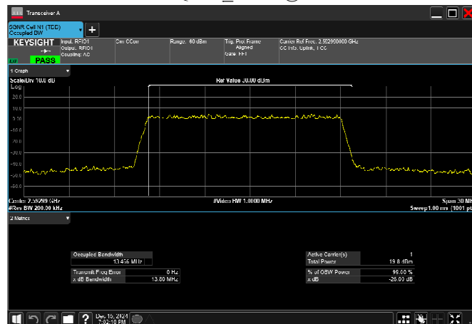
n41_15MHz_30kHz_2592.99MHz_CP-OFDM 16 QAM_RB38@0
