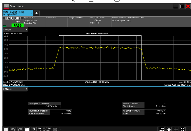
n41_15MHz_30kHz_2592.99MHz_CP-OFDM 64 QAM_RB38@0
