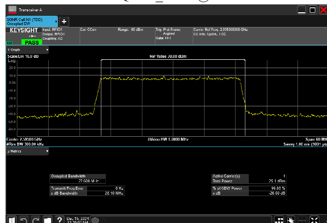
n38_30MHz_30kHz_2595MHz_DFT-s-OFDM 64 QAM_RB75@0
