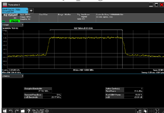
n38_40MHz_30kHz_2595MHz_DFT-s-OFDM QPSK_RB100@0
