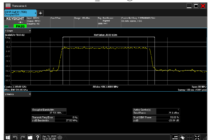
n38_40MHz_30kHz_2595MHz_DFT-s-OFDM 16 QAM_RB100@0
