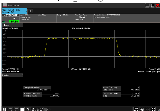
n38_40MHz_30kHz_2595MHz_DFT-s-OFDM QPSK_RB100@0
