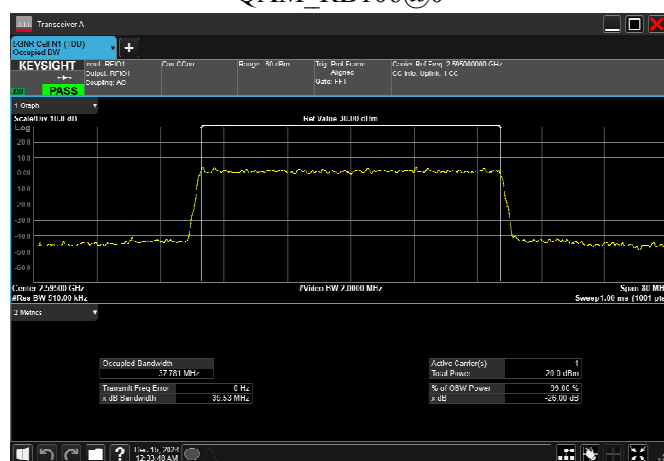
n38_40MHz_30kHz_2595MHz_CP-OFDM 256 OAM RB106@0
