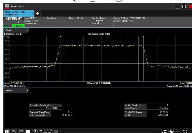
n41_15MHz_30kHz_2592.99MHz_CP-OFDM 256 QAM_RB38@0
