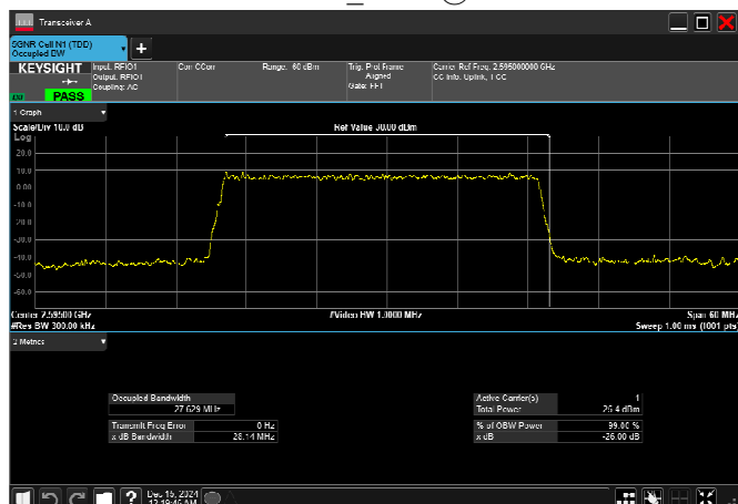
n38_30MHz_30kHz_2595MHz_DFT-s-OFDM 16 QAM_RB75@0
