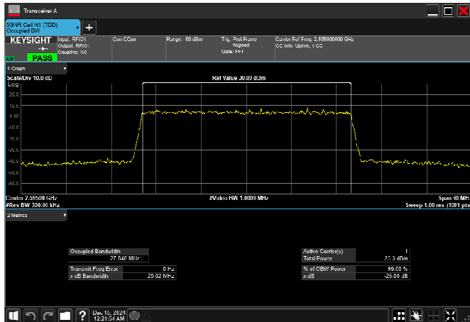
n38_30MHz_30kHz_2595MHz_CP-OFDM 256 QAM_RB78@0
