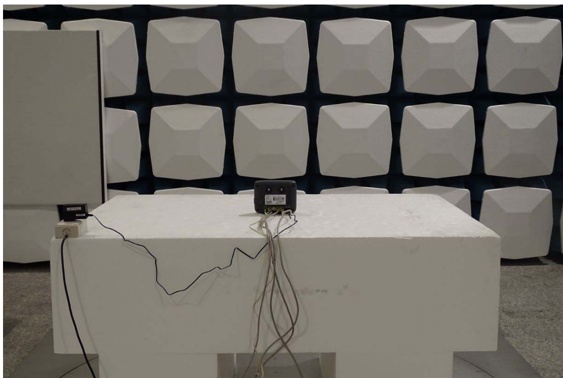
Back View of Radiated Test (M/N:MU12AR120100-A1)
