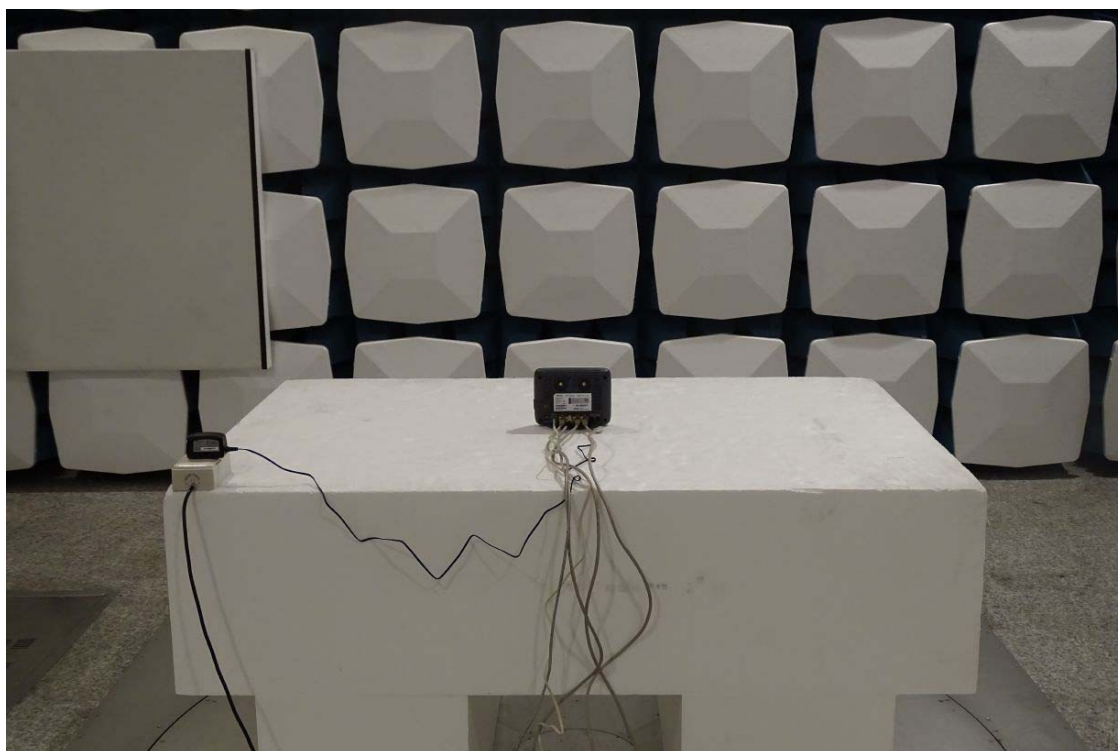
Back View of Radiated Test (M/N:WA-12M12FU)
