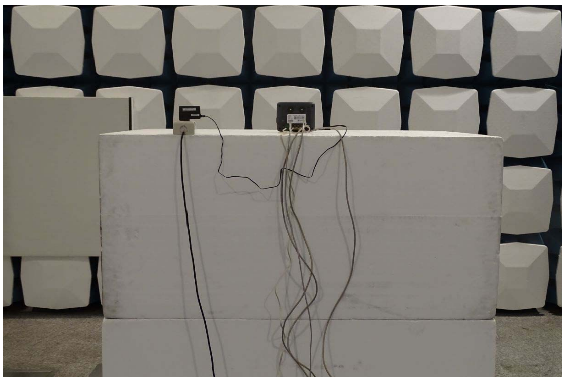
Back View of Radiated Test (Horn) (M/N:MU12AR120100-A1)
