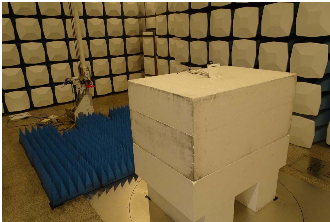
Back View of Radiated Test (Horn) (M/N:WA-12M12FU)
