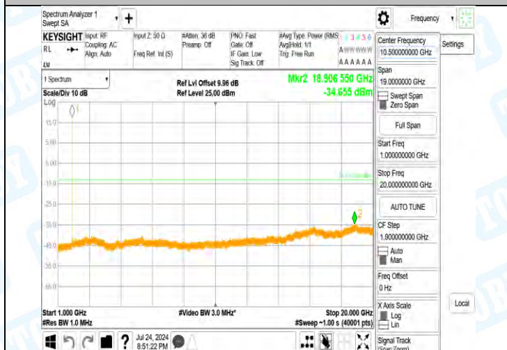
Band2-9400-3-1000~20000MHz-PASS
