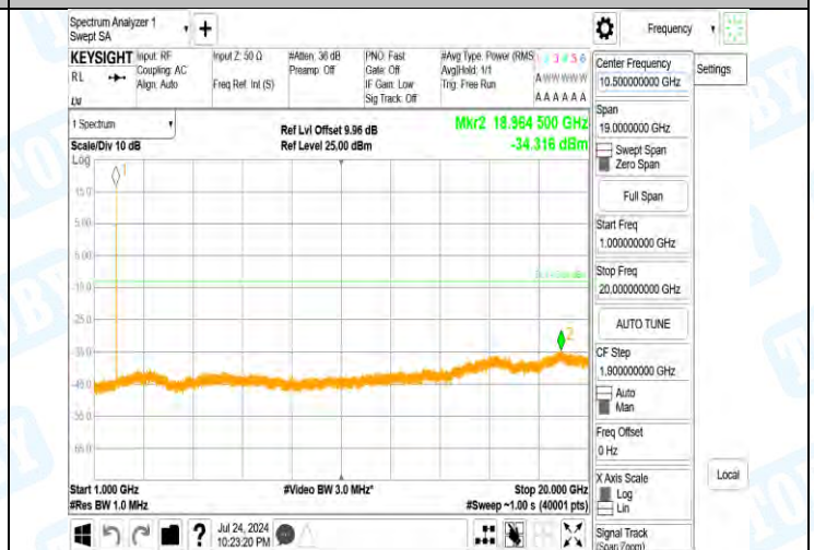
Band2-9262-5-1000~20000MHz-PASS
