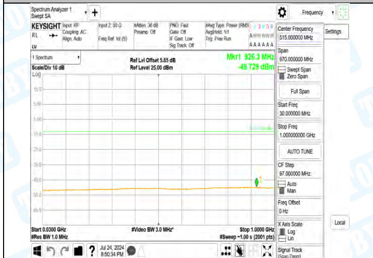
Band2-9262-3-30~1000MHz-PASS
