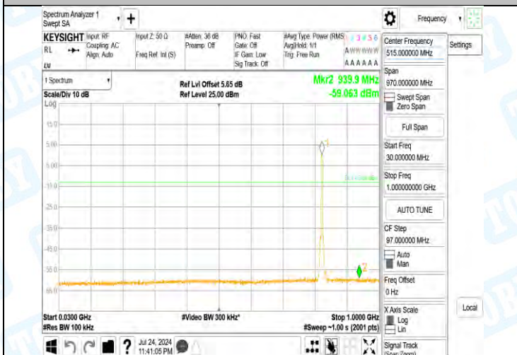
Band5-4132-3-30~1000MHz-PASS
