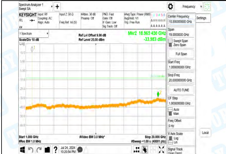
Band2-9400-4-1000~20000MHz-PASS
