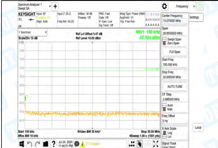
Band5-4132-4-0.15~30MHz-PASS
