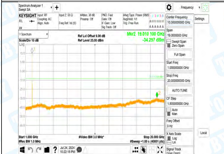
Band2-9538-4-1000~20000MHz-PASS
