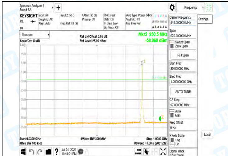
Band5-4132-5-30~1000MHz-PASS
