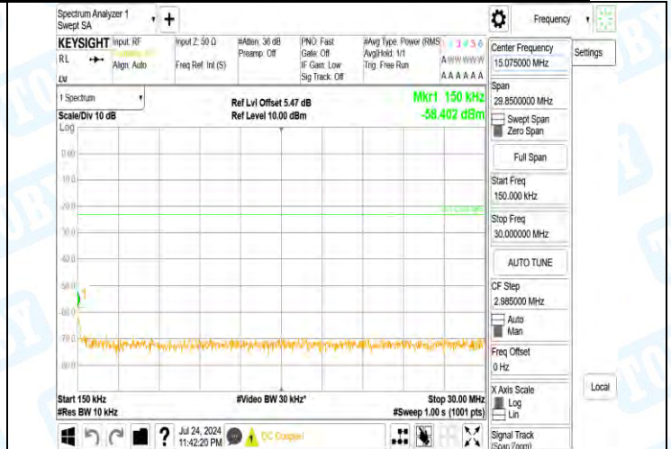
Band5-4182-3-0.15~30MHz-PASS
