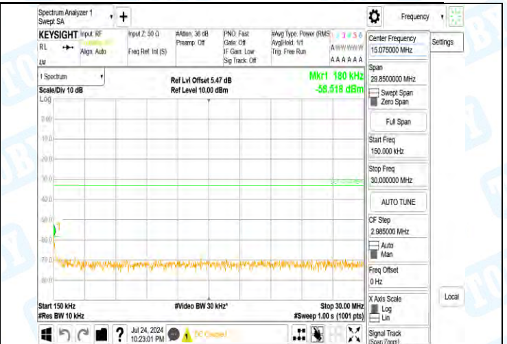
Band2-9262-5-0.15~30MHz-PASS
