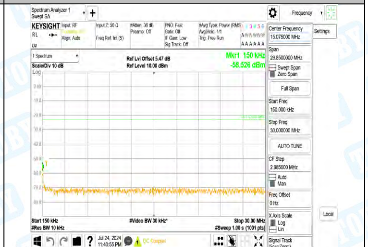
Band5-4132-3-0.15~30MHz-PASS
