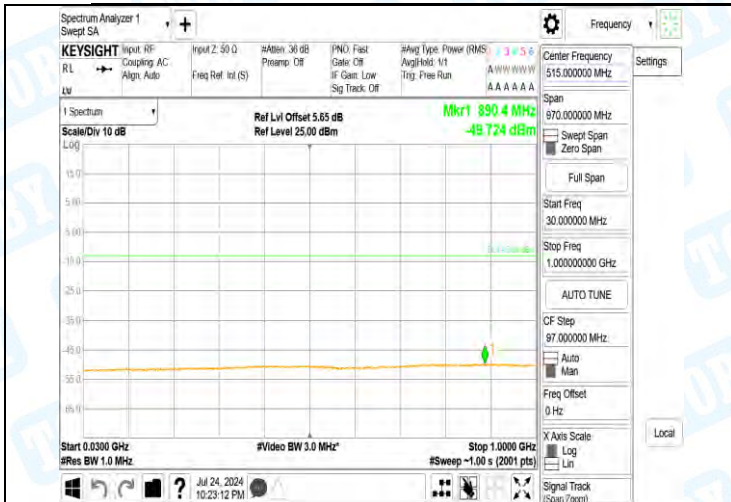
Band2-9262-5-30~1000MHz-PASS
