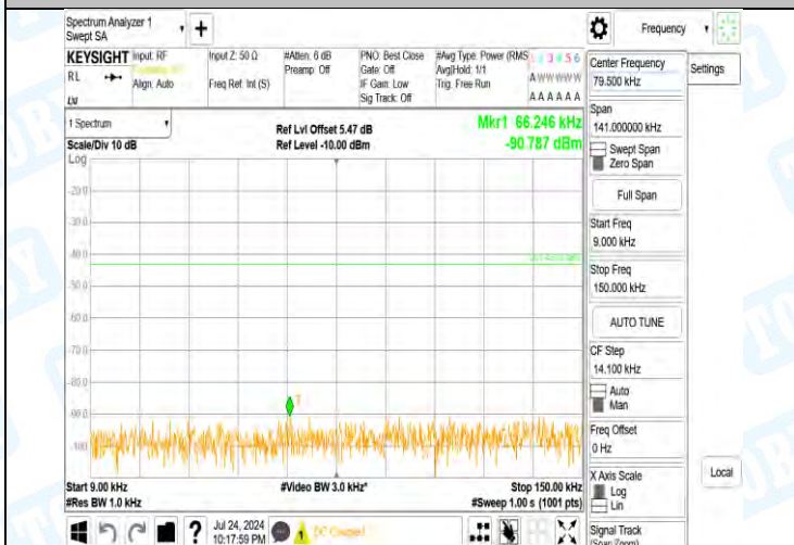
Band2-9538-3-0.009~0.15MHz-PASS
