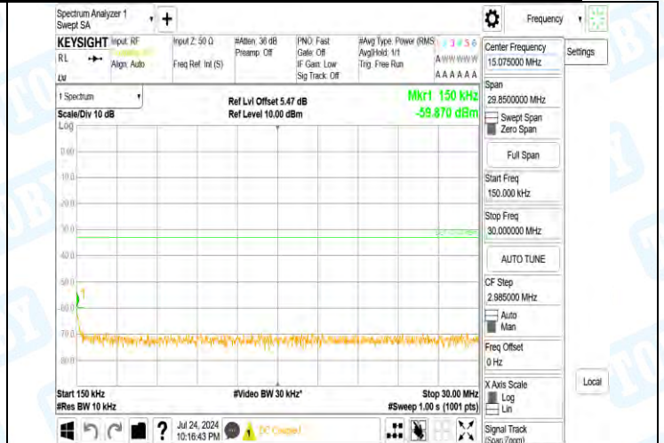
Band2-9400-3-0.15~30MHz-PASS
