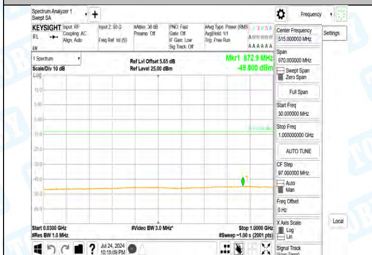
Band2-9262-3-30~1000MHz-PASS
