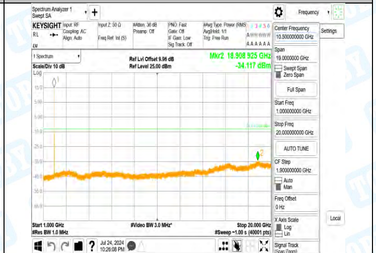
Band2-9538-5-1000~20000MHz-PASS
