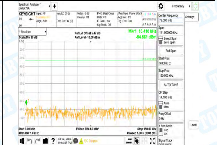
Band5-4132-4-0.009~0.15MHz-PASS
