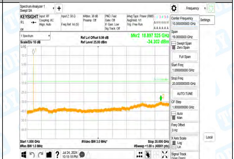
Band2-9262-3-1000~20000MHz-PASS
