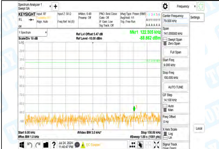
Band5-4132-3-0.009~0.15MHz-PASS
