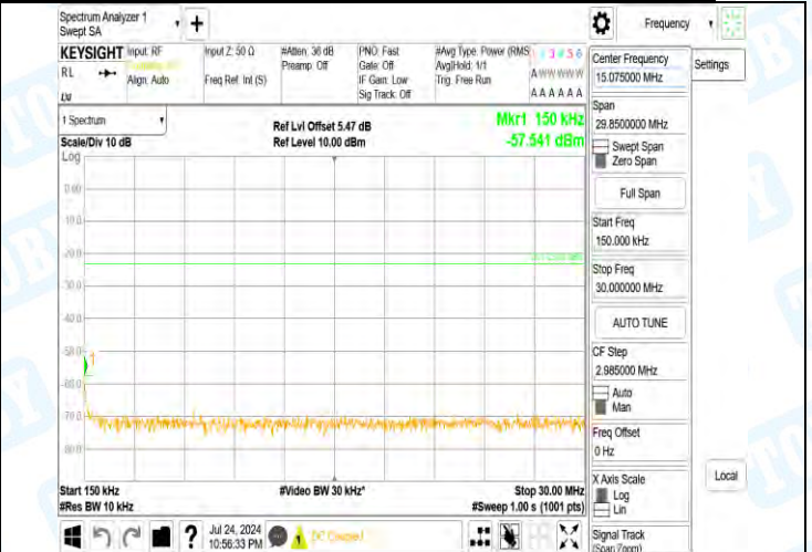
Band5-4233-4-0.15~30MHz-PASS
