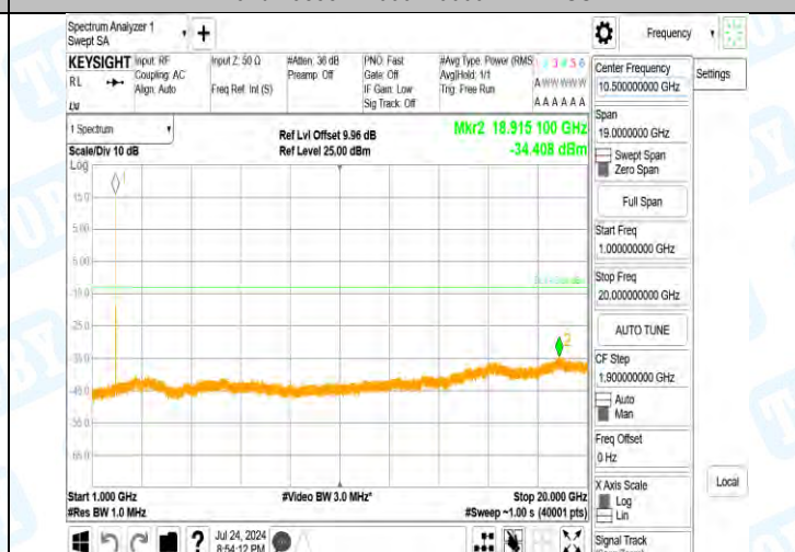
Band2-9538-4-1000~20000MHz-PASS
