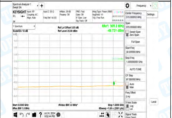
Band2-9262-4-30~1000MHz-PASS
