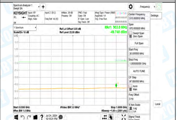
Band2-9262-4-30~1000MHz-PASS
