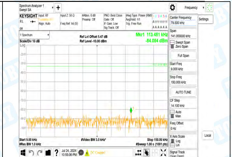
Band5-4132-4-0.009~0.15MHz-PASS
