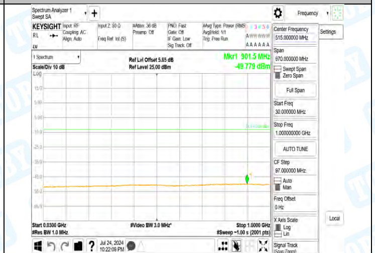
Band2-9538-4-30~1000MHz-PASS
