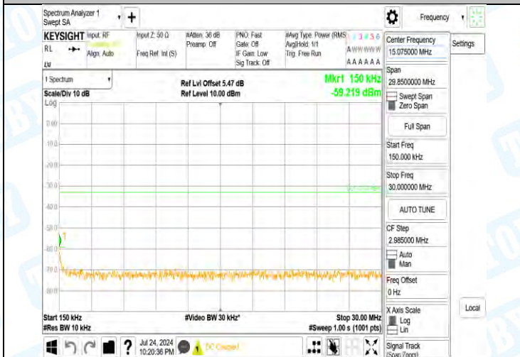
Band2-9400-4-0.15~30MHz-PASS
