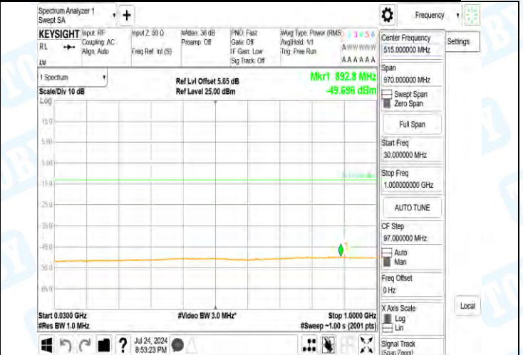
Band2-9400-4-30~1000MHz-PASS
