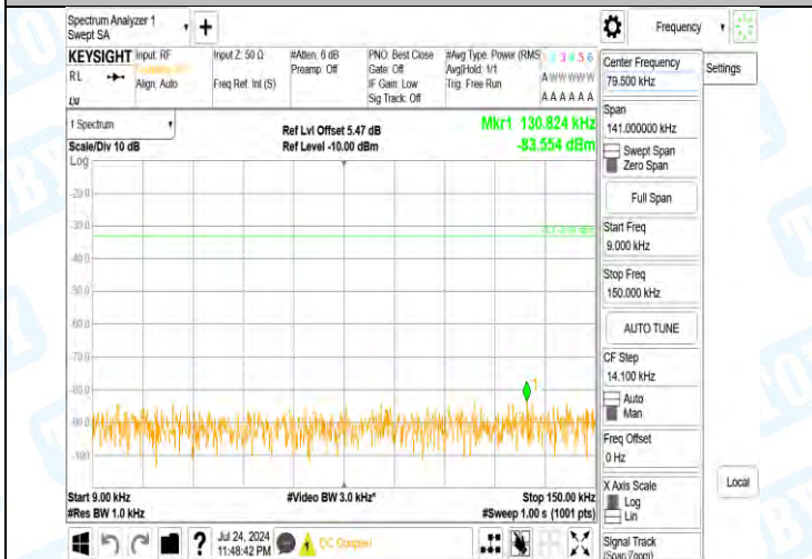
Band5-4132-5-0.009~0.15MHz-PASS
