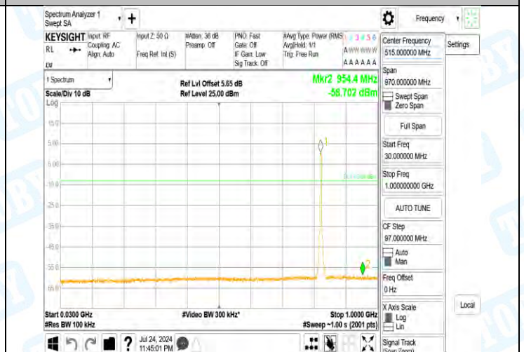
Band5-4132-4-30~1000MHz-PASS
