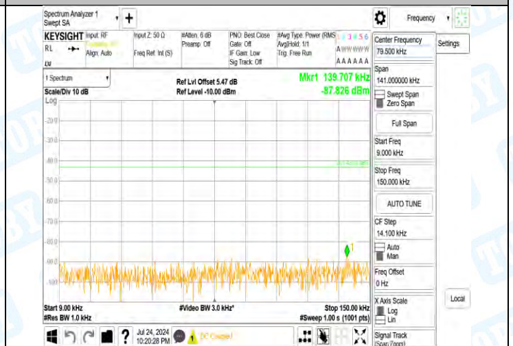
Band2-9400-4-0.009~0.15MHz-PASS
