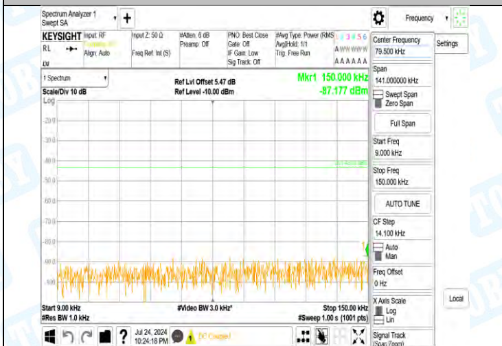
Band2-9400-5-0.009~0.15MHz-PASS
