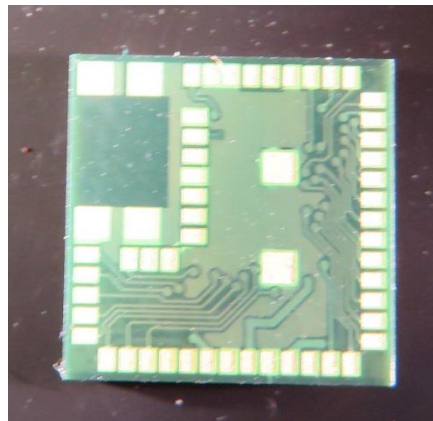
Figure 2: BGM12x external, bottom view
