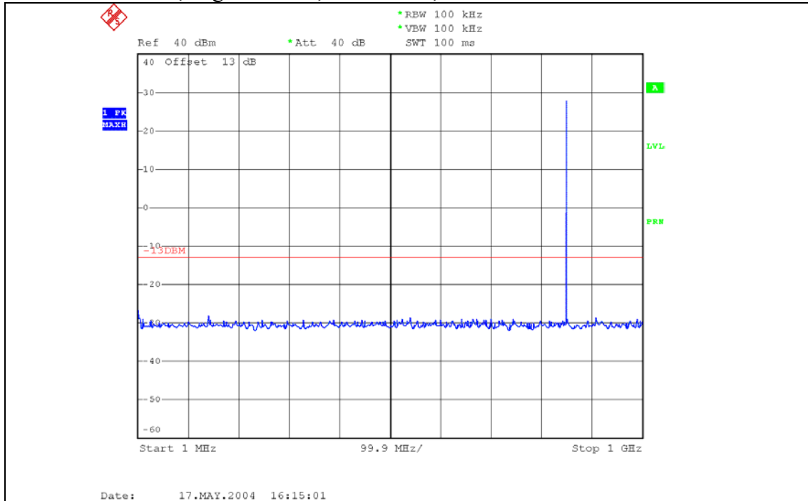
Plot 6.4.16) Out of Band Emissions at Antenna Terminals 8-PSK, High Channel, 848.8 MHz, 1 MHz to 1 GHz
