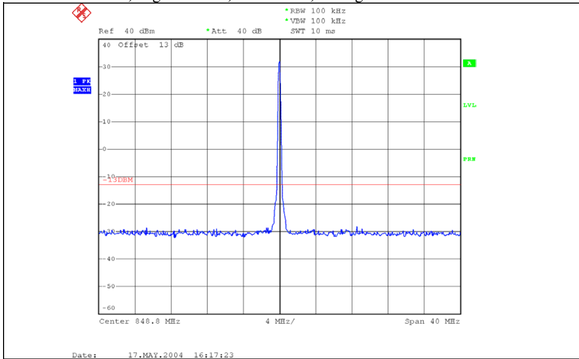
Plot 6.4.17) Out of Band Emissions at Antenna Terminals 8-PSK, High Channel, 848.8 MHz, TX signal +/- 20 MHz
