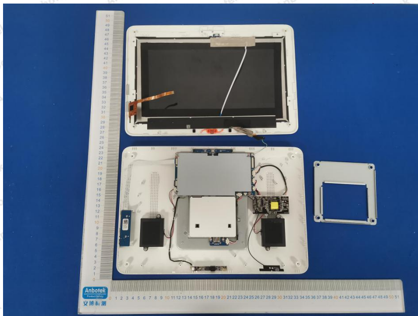
WIFI Antenna
