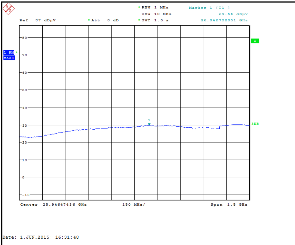
Plot 4-3: Radiated Fundamental (EIRP in 1 MHz) (TC #3)
