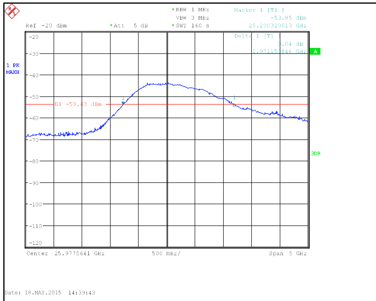
Plot 3-1: 10 dB Modulated Bandwidth – Standard Electronics PS60HK
