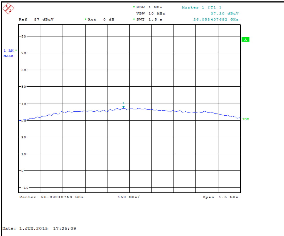
Plot 4-7: Radiated Fundamental (EIRP in 1 MHz) (TC #7)
