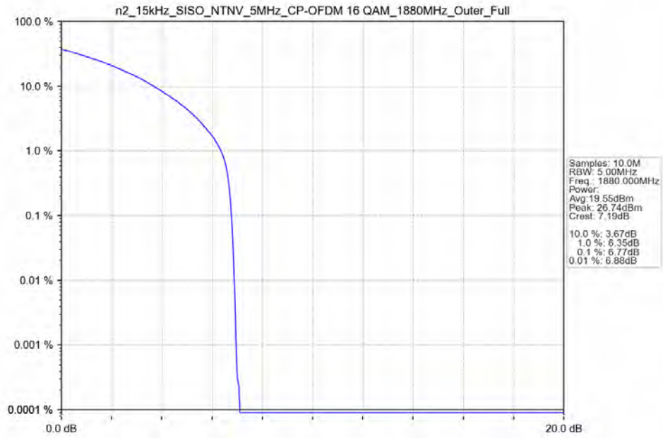
n2_15kHz_SISO_NTNV_5MHz_CP-OFDM_16_QAM_1880MHz_Outer_Full_Ant41
