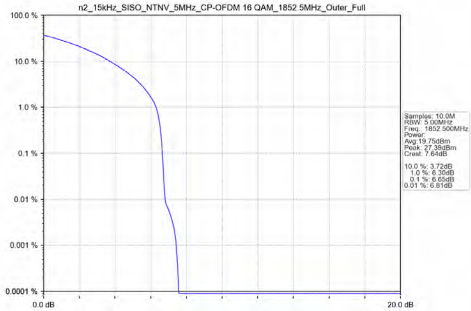
n2_15kHz_SISO_NTNV_5MHz_CP-OFDM_16_QAM_1852.5MHz_Outer_Full_Ant41
