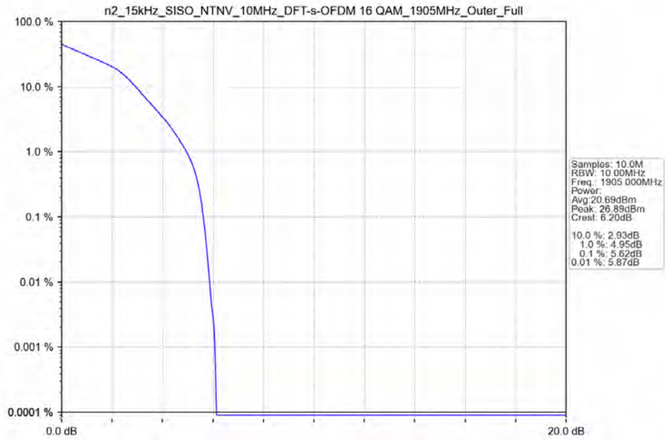
n2_15kHz_SISO_NTNV_10MHz_DFT-s-OFDM 16 QAM_1905MHz_Outer_Full_Ant41
