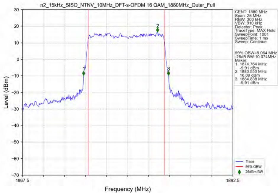
n2_15kHz_SISO_NTNV_10MHz_DFT-s-OFDM_16_QAM_1880MHz_Outer_Full_Ant41
