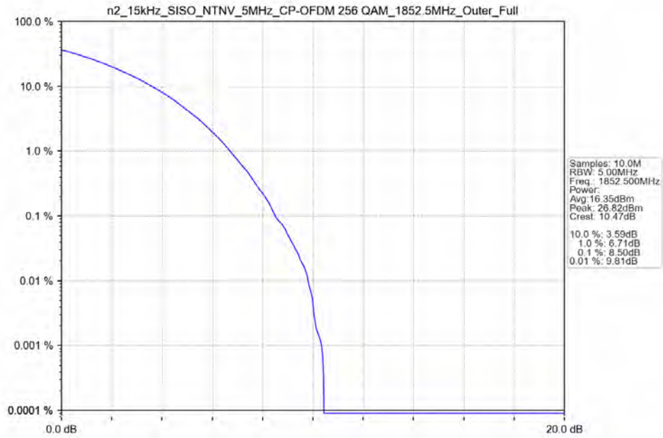
n2_15kHz_SISO_NTNV_5MHz_CP-OFDM_256_QAM_1852.5MHz_Outer_Full_Ant41
