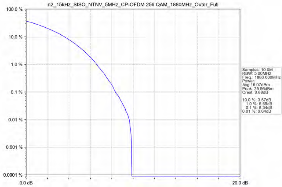
n2_15kHz_SISO_NTNV_5MHz_CP-OFDM_256_QAM_1880MHz_Outer_Full_Ant41
