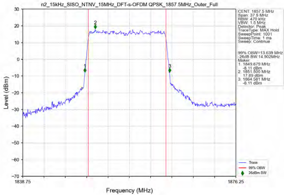
n2_15kHz_SISO_NTNV_15MHz_DFT-s-OFDM_QPSK_1857.5MHz_Outer_Full_Ant41
