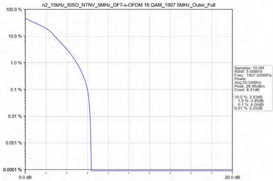
n2_15kHz_SISO_NTNV_5MHz_DFT-s-OFDM_16_QAM_1907.5MHz_Outer_Full_Ant41
