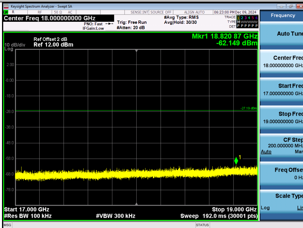
11N40SISO-Ant1-2437-17000~19000-PASS
