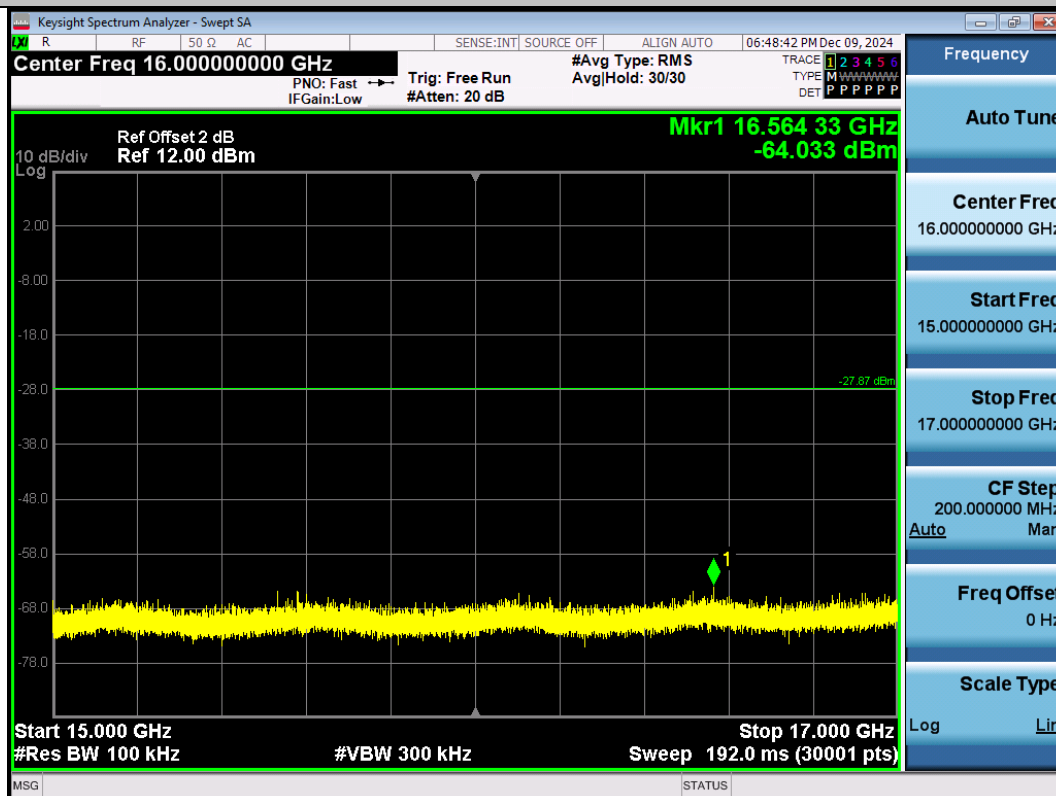
11N40SISO-Ant1-2452-15000~17000-PASS
