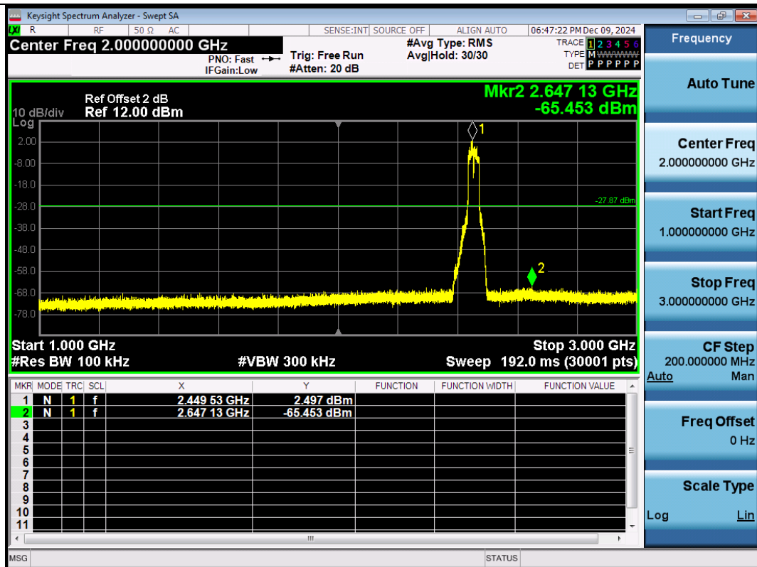
11N40SISO-Ant1-2452-1000~3000-PASS
