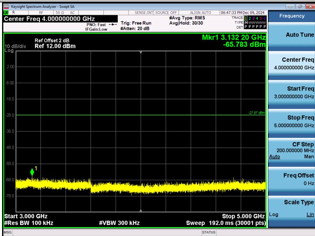
11N40SISO-Ant1-2452-3000~5000-PASS
