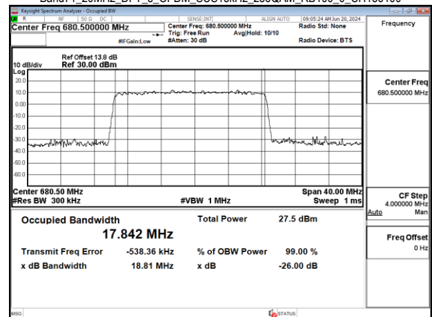
Band71_20MHz_DFT_s_OFDM_SCS15kHz_256QAM_RB100_0_CH136100
