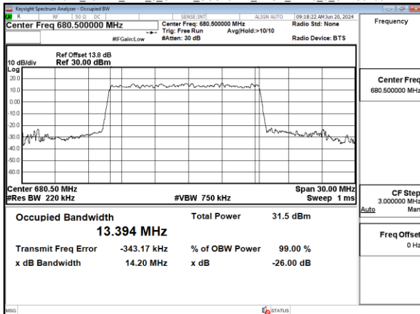
Band71_15MHz_DFT_s_OFDM_SCS15kHz_BPSK_RB75_0_CH136100
