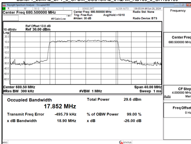
Band71_20MHz_DFT_s_OFDM_SCS15kHz_64QAM_RB100_0_CH136100
