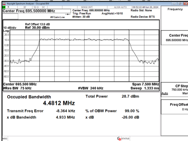
Band71_5MHz_DFT_s_OFDM_SCS15kHz_256QAM_RB25_0_CH139100
