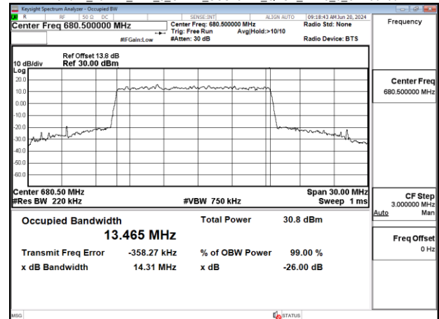
Band71_15MHz_DFT_s_OFDM_SCS15kHz_QPSK_RB75_0_CH136100
