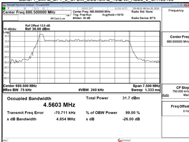
Band71_5MHz_DFT_s_OFDM_SCS15kHz_16QAM_RB25_0_CH136100
