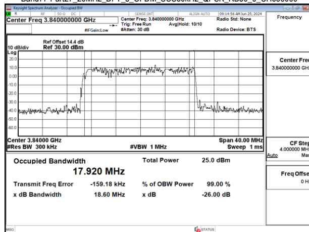
Band77-Part27_20MHz_DFT_s_OFDM_SCS30kHz_QPSK_RB50_0_CH656000
