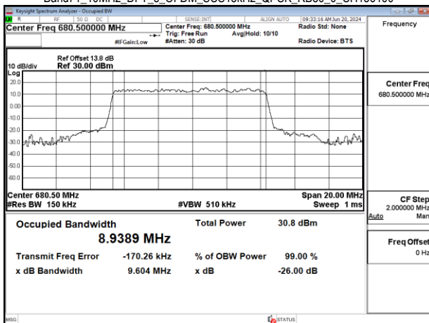
Band71_10MHz_DFT_s_OFDM_SCS15kHz_QPSK_RB50_0_CH136100
