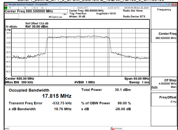
Band71_20MHz_DFT_s_OFDM_SCS15kHz_16QAM_RB100_0_CH136100
