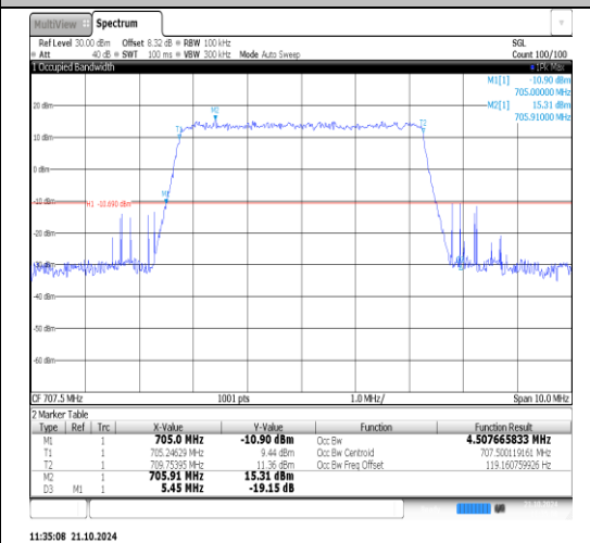
Band12-10MHz-16QAM-23095-50RB#0-PASS
