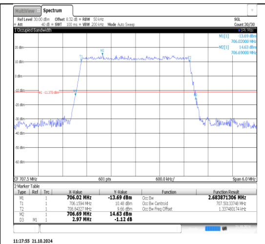
Band12-5MHz-16QAM-23095-25RB#0-PASS
